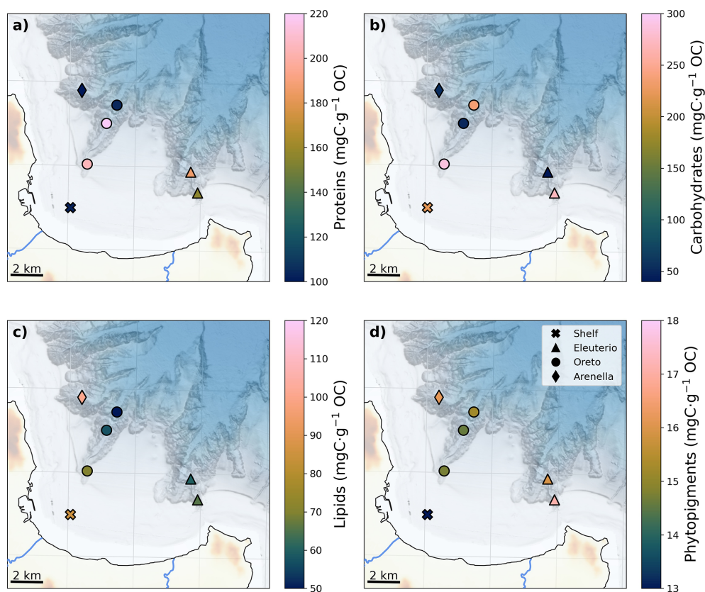
Figure 3. Spatial distribution of composition of organic matter: (a) proteins, (b) carbohydrates, (c) lipids, and phytopygments. Colour bars are adjusted to highlight the minimum, mean, and maximum values for each variable.
