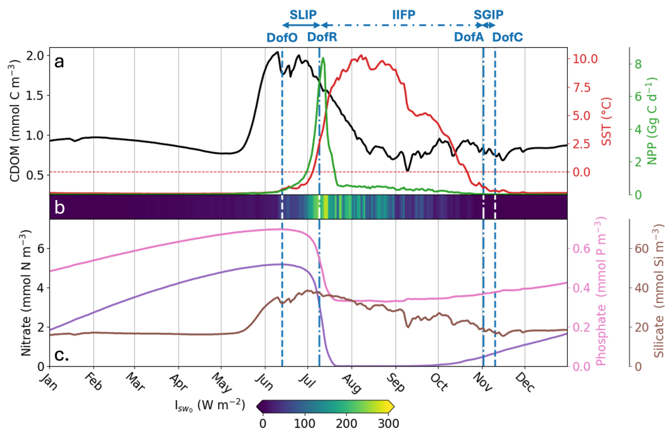
Figure 3. Spatially-averaged surface-ocean parameters simulated by \text{Run}_{\text{full}} in the Mackenzie River plume during 2012. Parameters shown are: (a) CDOM concentration ( \text{mmol C m}^{-3} ; black line), SST ( ^{\circ}\text{C} ; red line), NPP ( \text{Gg C d}^{-1} ; green line), (b) shortwave downwelling irradiance at the ocean surface ( I_{\text{sw}0} ; \text{W m}^{-2} ), (c) nitrate concentration ( \text{mmol N m}^{-3} ; purple line), phosphate concentration ( \text{mmol P m}^{-3} ; pink line) and, silicate concentration ( \text{mmol Si m}^{-3} ; brown line). The vertical dashed blue lines show the spatial-mean day of opening (DofO) and day of closing (DofC) and the vertical dashed-dotted blue lines show the spatial-mean day of retreat (DofR) and day of advance (DofA). Sea ice melting periods are shown consecutively, the seasonal loss of ice period (SLIP), the inner ice-free period (IIFP), and the seasonal gain of ice period (SGIP).
