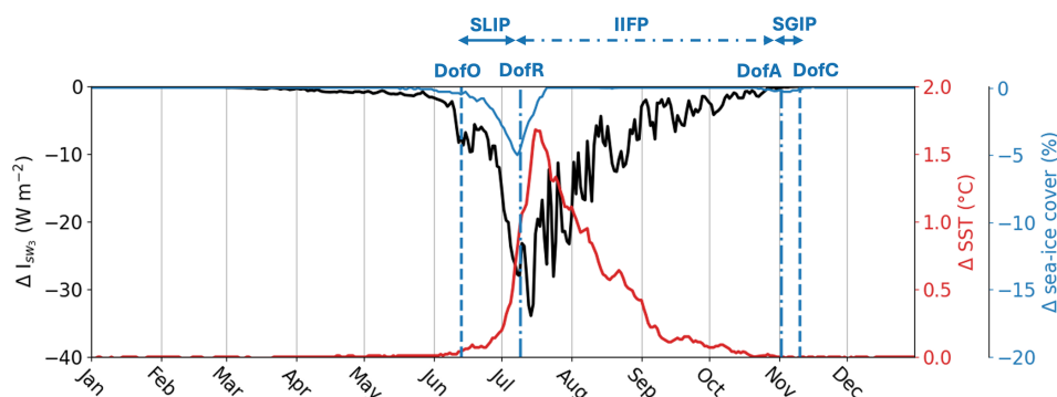
Figure 5. Difference in subsurface shortwave downwelling irradiance at 3 m depth ( I_{\text{sw}3} in \text{W m}^{-2} ; black line), SST ( ^{\circ}\text{C} ; red line) and sea ice concentration (%; blue line) between \text{Run}_{\text{full}} and \text{Run}_{\text{ctrl}} . The vertical dashed blue lines show the spatial-mean Day of Opening (DofO) and Day of Closing (DofC) and the vertical dashed-dotted blue lines show the spatial-mean Day of Retreat (DofR) and Day of Advance (DofA) simulated by \text{Run}_{\text{full}} .
