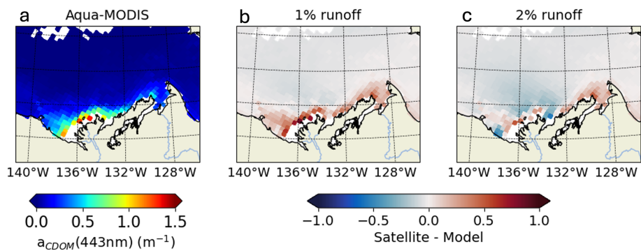
Figure B1. 2009 annual-mean CDOM absorption at 443 nm from (a) remotely-sensed observations and differences from simulated CDOM fields with (b) 1 % and (c) 2 % of tDOC redistributed into CDOM tracer. Simulated CDOM absorption is compared with satellite observations that are space-time colocated with the simulations.
