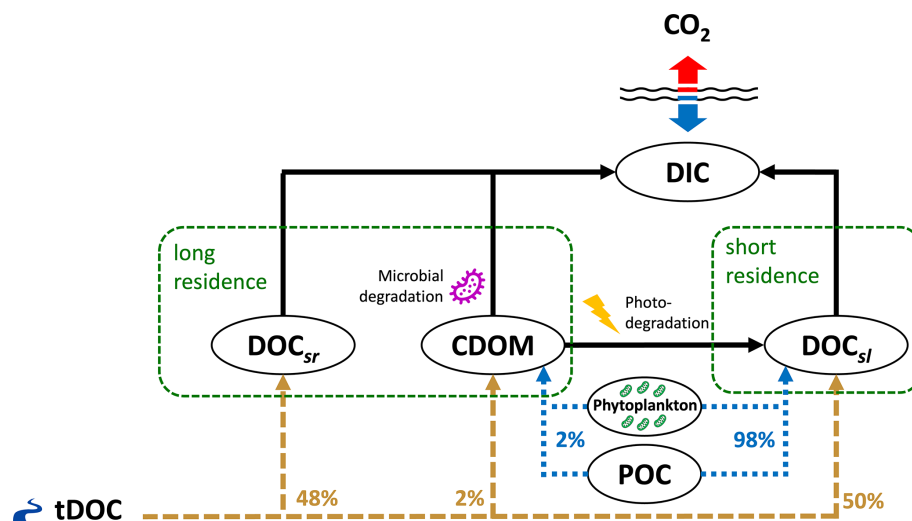
Figure 1. Conceptual diagram of dissolved carbon mass fluxes in the ED-SBS model. The Mackenzie River terrestrial DOC (tDOC) mass flux (dashed brown lines) is distributed into marine DOC and CDOM pools according to the percentages shown in brown text. The result of phytoplankton grazing/mortality and particulate organic carbon (POC) dissolution is distributed over the DOC sl and CDOM pools (dotted blue lines).
