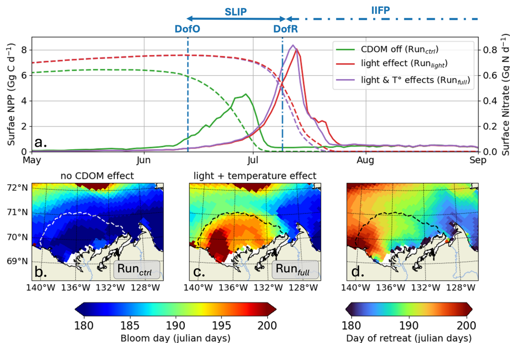
Figure 7. (a) Surface-ocean NPP ( \text{Gg C d}^{-1} ; thick lines) and nitrate stock ( \text{Gg N d}^{-1} ; dashed lines) simulated by ED-SBS without the CDOM light attenuation effect (green line; \text{Run}_{\text{ctrl}} ), including (1) CDOM PAR light attenuation (red line; \text{Run}_{\text{light}} ) and (2) CDOM light attenuation and ocean warming effect (purple line; \text{Run}_{\text{full}} ). Maps of bloom day (julian days) (b) without the CDOM light attenuation effect, (c) including CDOM PAR light attenuation, and (d) map of DofR (julian days) simulated by EDS-SBS. Dashed line on the maps show the time-mean SSS isohaline of 27; vertical dashed and dashed-dotted blue lines show the DofO and DofR, respectively.
