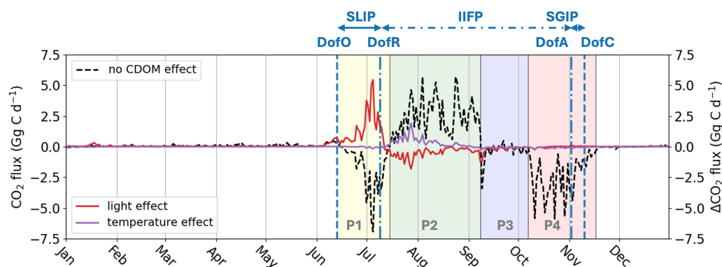
Figure 8. Air-sea \text{CO}_2 flux ( \text{Gg C d}^{-1} ) simulated by \text{Run}_{\text{ctrl}} in the plume region without CDOM biophysical feedback effects (black dashed line) and the change in air-sea \text{CO}_2 flux ( \text{Gg C d}^{-1} ) induced by the PAR light attenuation effect (red thick line) and warming effect (purple thick line). The vertical dashed blue lines show the average DofO and DofC and the vertical dashed-dotted blue lines show the average DofR and DofA. Phases with a switch in air-sea \text{CO}_2 flux simulated by \text{Run}_{\text{ctrl}} are indicated by four colors (P1: yellow, P2: green, P3: blue, and P4: red).
