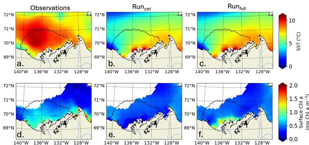
Figure D1. SST ( ^{\circ}\text{C} ) averaged from July to September 2012 (top row) and surface Chl a ( \text{mg Chl } a \text{ m}^{-3} ) averaged from June to July 2012 (lower row) for observations (a, d), \text{Run}_{\text{ctrl}} (b, e), \text{Run}_{\text{full}} (c, f). The dashed line shows the plume region (time-mean SSS isohaline of 27).
