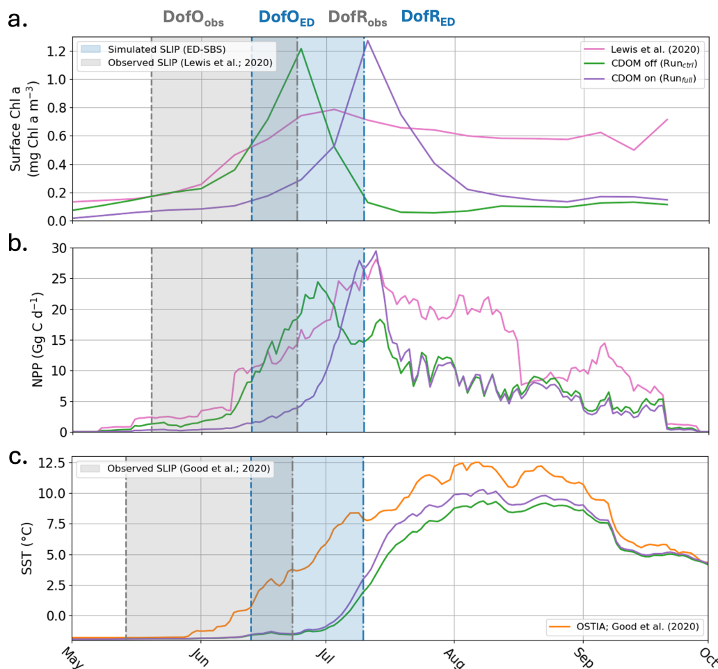
Figure 9. 2012 (a) averaged Surface Chl a (mg Chl a m -3 ), (b) integrated NPP (Gg C d -1 ), and (c) averaged SST (°C) over the Mackenzie River plume region for Run ctrl (green line), Run full (purple line), satellite observations (pink line; Lewis et al., 2020), and in-situ/satellite observations (orange line; Good et al., 2020). The blue (grey) area indicates the simulated (observed) seasonal loss of ice period.
