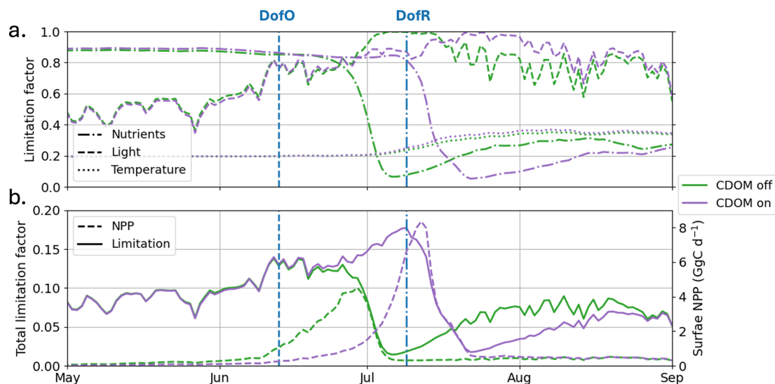
Figure E1. 2012 (a) simulated limitation factors for nutrients (dash-dotted lines), light (dashed lines), and temperature (dotted lines), averaged between the two phytoplankton functional types and in the plume region for Run ctrl (green lines) and Run full (purple lines) and (b) simulated total limitation averaged between the two phytoplankton functional types and in the plume region and NPP spatially-integrated in the plume region for Run full (purple lines) and Run ctrl (green lines).
