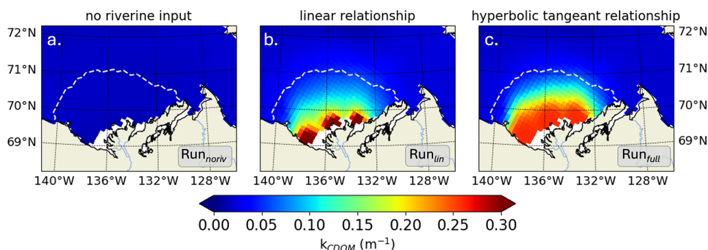
Figure 4. For July 2012, time-mean CDOM diffuse attenuation coefficient ( k_{\text{CDOM}} , \text{m}^{-1} ) for (a) \text{Run}_{\text{noriv}} , (b) \text{Run}_{\text{lin}} , and (c) \text{Run}_{\text{full}} . The white dashed line marks the time-mean spatial extent of the Mackenzie River plume.
