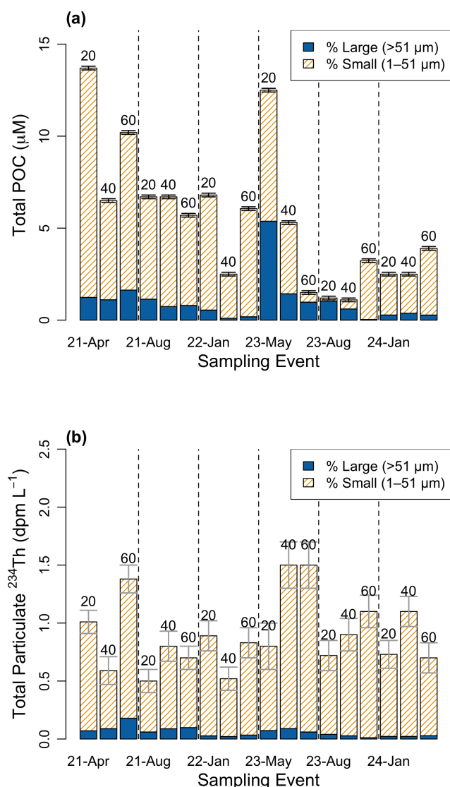
Figure 4. Size-fractionated (1–51, > 51 \mu\text{m} ) pools of (a) particulate organic carbon ( \mu\text{M} ) and (b) total particulate ^{234}\text{Th} ( \text{dpm L}^{-1} ) at approximately 20, 40, and 60 m for each sampling event. Bars are stacked and totals equal the sum of the small and large fractions (legend shows % contribution by size class). Numbers above bars indicate approximate sampling depth. Dashed lines separate events. The small fraction generally dominates both POC and ^{234}\text{Th} .
