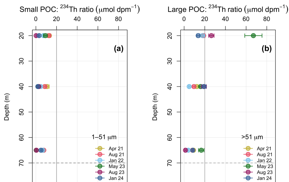
Figure 5. Water column ratios of POC to ^{234}\text{Th} ( \text{POC} : ^{234}\text{Th} ; \mu\text{mol C dpm}^{-1} ) in each sampling event throughout 2021–2024. Error bars indicate propagated uncertainties associated with measurements. (a) \text{POC} : ^{234}\text{Th} on the small particle (1–51 \mu\text{m} ) fraction (b) \text{POC} : ^{234}\text{Th} on the large particle (> 51 \mu\text{m} ) fraction. Other than a few large \text{POC} : ^{234}\text{Th} ratios that correspond with greater chl a in the water column (Fig. 2d), the \text{POC} : ^{234}\text{Th} ratios are similar in magnitude on both size fractions (< 20 \mu\text{mol C dpm}^{-1} ; grey reference line). The dashed grey line at 70 m represents the bottom of the Bedford Basin.
