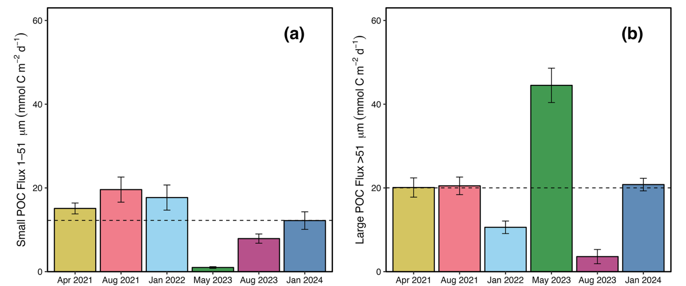
Figure 7. Depositional POC fluxes to the seabed in the Bedford Basin. Measured 234 Th-derived mean (± s.d.) particulate organic carbon fluxes deposited to the near bottom (~ 65 m) of the Bedford Basin on the (a) small particle (1–51 μm) and (b) large particle (> 51 μm) size fractions. The dashed black line represents the mean POC flux for each size fraction respectively.
