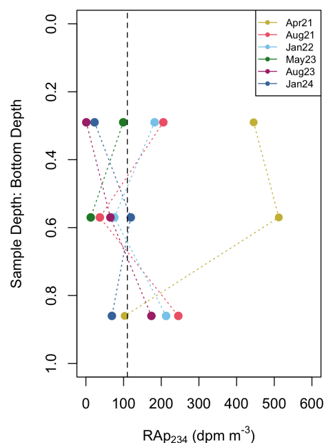
Figure 9. Profiles of the total residual activity of particulate ^{234}\text{Th} ( \text{Rap}_{234} ) at the Compass Station vs. normalized depth calculated as sample depth divided by total water depth (0 = surface, 1 = bottom). \text{Rap}_{234} values represent the sum of residual counts from both size fractions. Only \text{Rap}_{234} signals above the detection limit were found on the small particulate fraction. The dashed vertical line is the detection limit (derived from filter blank analyses).
