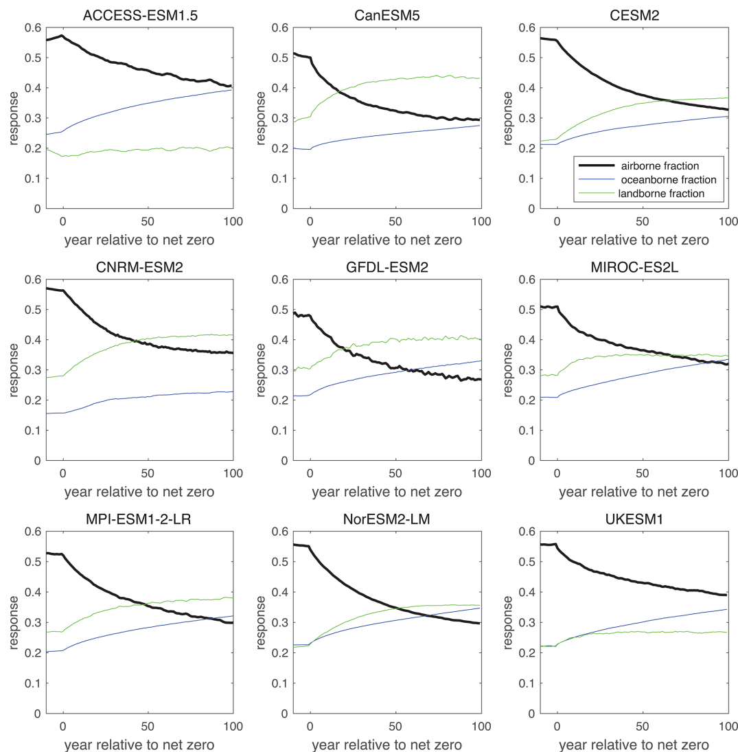
Figure 5. Temporal evolution of cumulative airborne fraction, \Delta I_A(t') (black), landborne fraction \Delta I_L(t') (green) and oceanborne fraction \Delta I_O(t') (blue) for time (year) relative to net zero for 9 different Earth system models.
