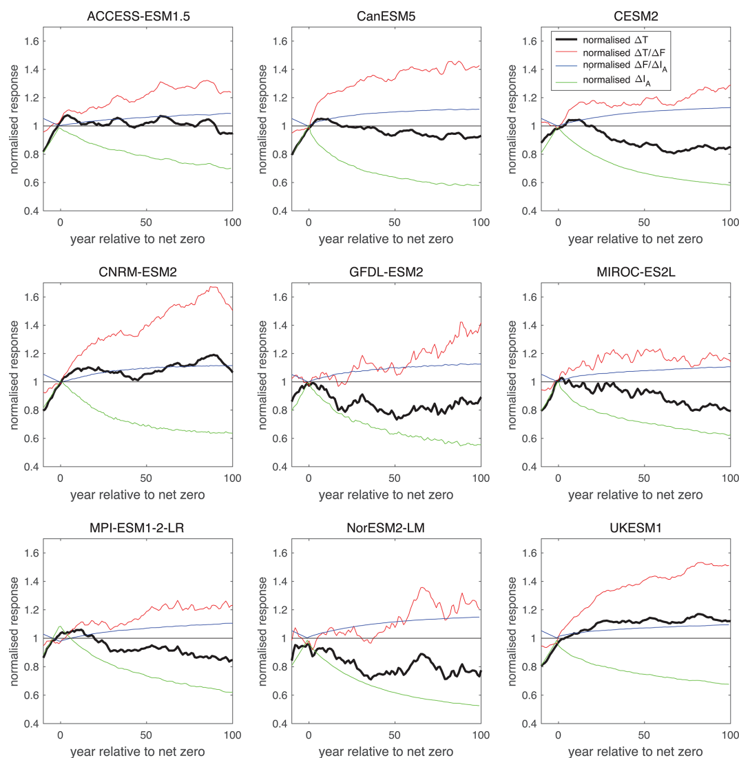
Figure 4. Temporal evolution of the geometric ZEC and its contributions for 9 different Earth system models: the normalised surface temperature change, \Delta T(t') , (black line); the thermal contribution from the normalised dependence of surface temperature on radiative forcing, \Delta T(t')/\Delta F(t') (red line); the radiative contribution from the normalised dependence of radiative forcing on atmospheric carbon, \Delta F(t')/\Delta I_A(t') (blue line); and carbon contribution from the normalised atmospheric carbon, \Delta I_A(t') (green line). The normalisation is based on the values of each variable at the time of net zero. The plot includes smoothing of temperature, the alignment of the time series and normalisation as in Fig. 3.
