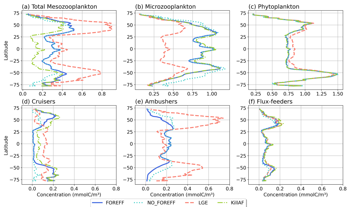
Figure 9. Annual and zonal (averaged over 150 m depth) mean biomass of (a) total mesozooplankton, (b) microzooplankton, (c) phytoplankton, (d) cruisers, (e) ambushers, and (f) flux-feeders for the different experiments (in \text{mmol C m}^{-3} ): FOREFF in dark blue line, NO_FOREFF in dotted blue is similar to FOREFF but with constant foraging effort, LGE (Low Growth Efficiency) in dashed pink corresponds to same growth rate for suspension feeders but lower growth efficiency for cruisers, and KILL_AF in dash and dotted green is similar to FOREFF but ambushers are removed.
