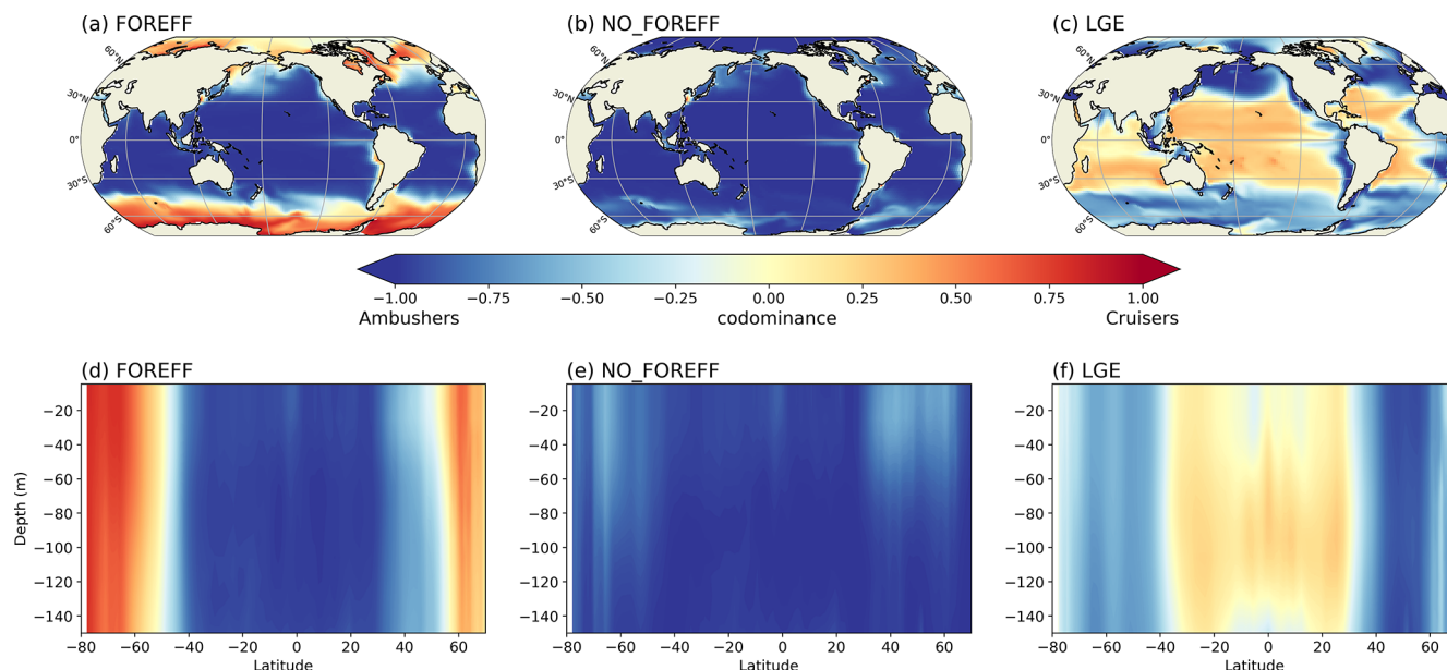
Figure 6. Annual mean of the dominance index between cruisers (CF) and ambushers (AF), averaged over 150 m (a–c) and zonally averaged (d–f) for the different experiments: (a, d) reference (FOREFF), (b, e) constant foraging effort (NO_FOREFF), and (c, f) same growth rate for suspension feeders but lower growth efficiency for cruisers (LGE).
