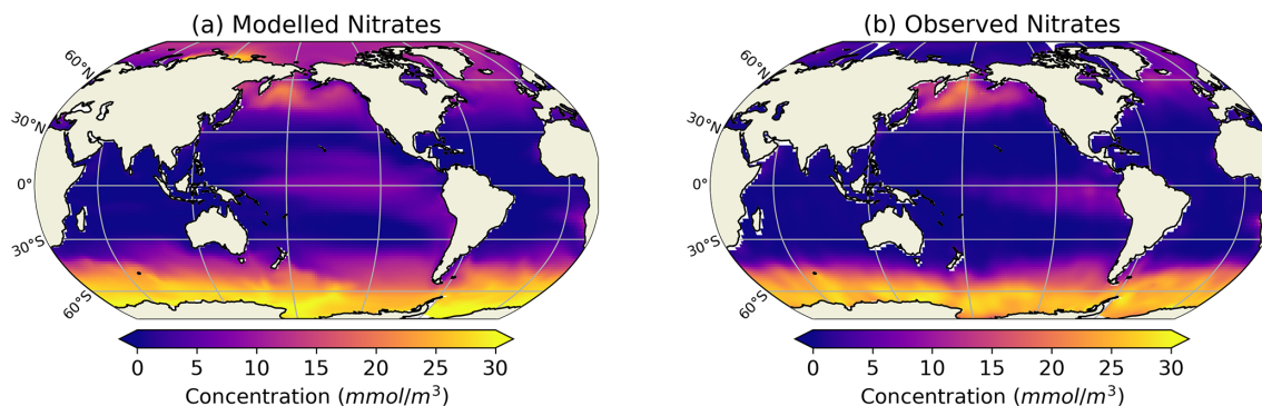
Figure A3. Comparison between modelled and observed annual average surface nitrate. Observed surface nitrate are from World Ocean Atlas (Garcia et al., 2010).
