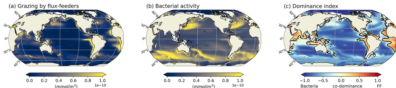
Figure A11. Annual mean (a) grazing by flux-feeders, (b) bacterial activity, and (c) dominance index between the effect of flux-feeders and bacterial activities, averaged between 150–1000 m. Regions in blue indicate a larger bacterial activity, while regions in red indicate a larger flux-feeders activity. The black line indicates where the index is 0, i.e. where we obtain a co-dominance between the effect of flux-feeders and the effect of bacterial activity.
