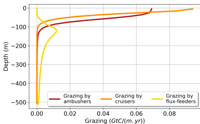
Figure 5. Annual mean of the modelled grazing rate ( \text{GtC (m yr)}^{-1} ) of the different mesozooplankton groups (ambushers in red, cruisers in orange, and flux-feeders in yellow) along the vertical dimension from 0 to 500 m deep.
