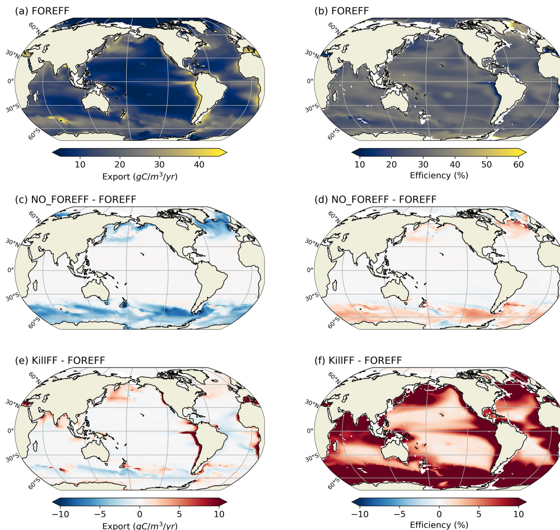
Figure 10. Annual mean of carbon export at 150 m ( a, c, e , in \text{g C m}^{-3} \text{ yr}^{-1} ) and of carbon transfer efficiency between 150–1000 m ( b, d, f , in %). ( a, b ) Values obtained for the reference FOREFF simulation. ( c, d ) Differences between FOREFF and NO_FOREFF (similar to FOREFF but without a variable foraging effort). ( e, f ) Differences between FOREFF and KILL_FF (similar to FOREFF but flux-feeders are killed).
