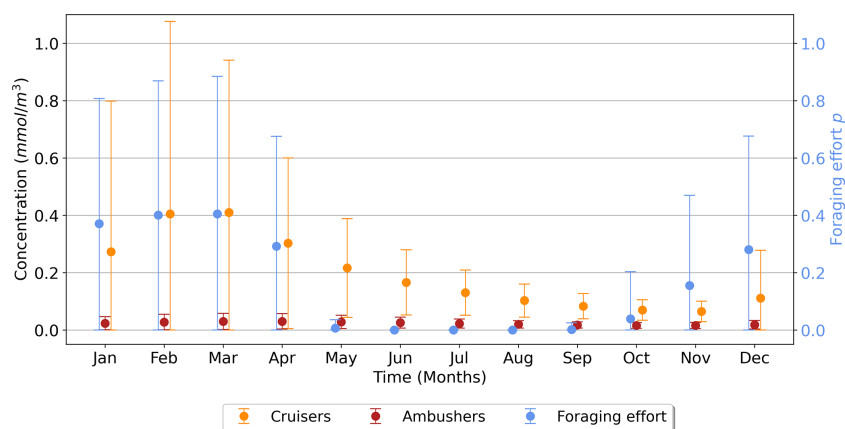
Figure 8. Time series (in months) over the high latitudes of the Southern Ocean (> 60° S) for the suspension feeders' concentration (cruisers in orange, ambushers in red, in mmolC m -3 ) and the foraging effort (unitless, in blue), averaged over the top 150 m. The vertical bars represent the standard deviation.
