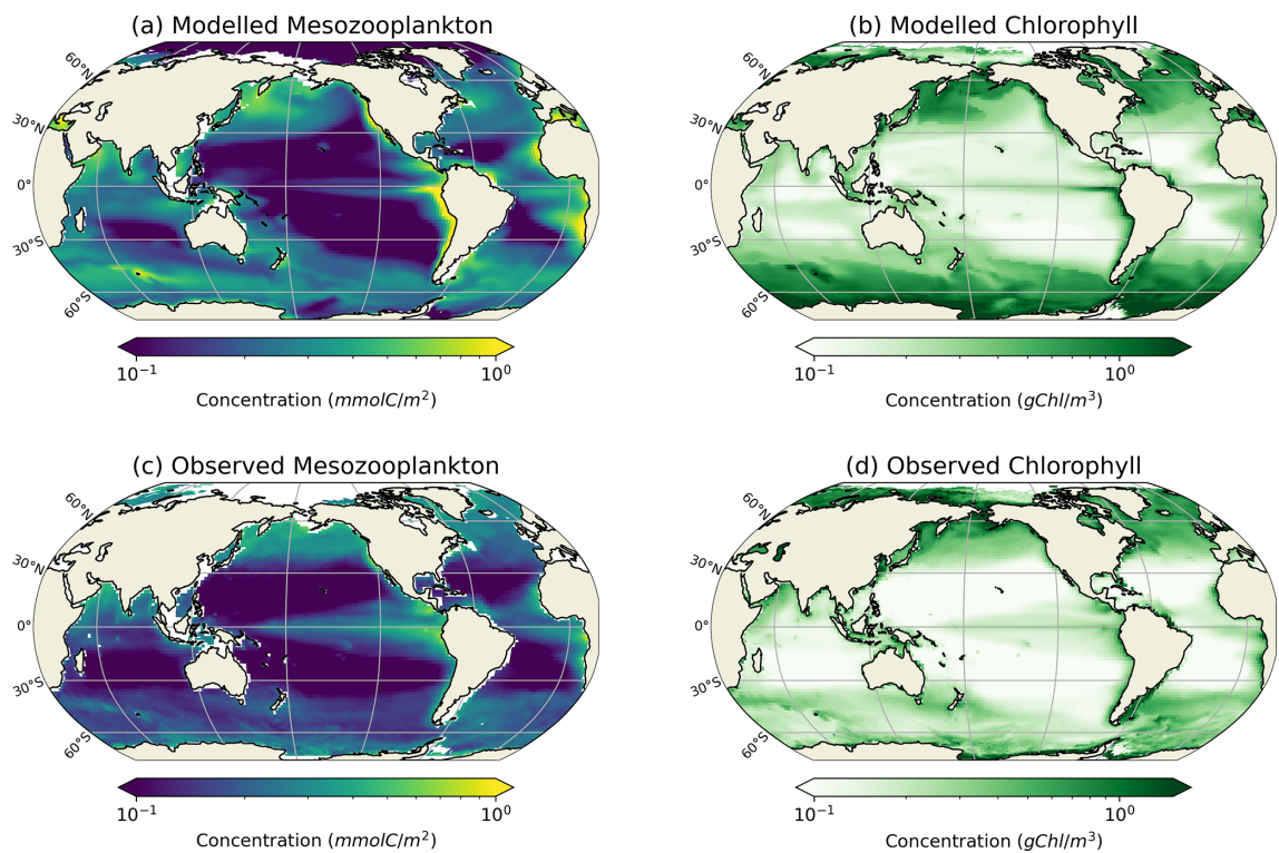
Figure 3. Comparison between modelled (a, b) and observed (c, d) log-scaled mean annual mesozooplankton biomass concentration integrated over the top 200 m and mean annual surface chlorophyll concentration. (a) Total modelled mesozooplankton concentration, (b) modelled chlorophyll, (c) observed mesozooplankton biomass obtained from the BDM pipeline trained on the MAREDAT annual climatology made by Clerc et al. (2024), and (d) observed chlorophyll concentration from OC-CCI (ESA). Mesozooplankton biomass are expressed in \text{mmol C m}^{-3} and chlorophyll concentration in \text{g Chl m}^{-3} .
