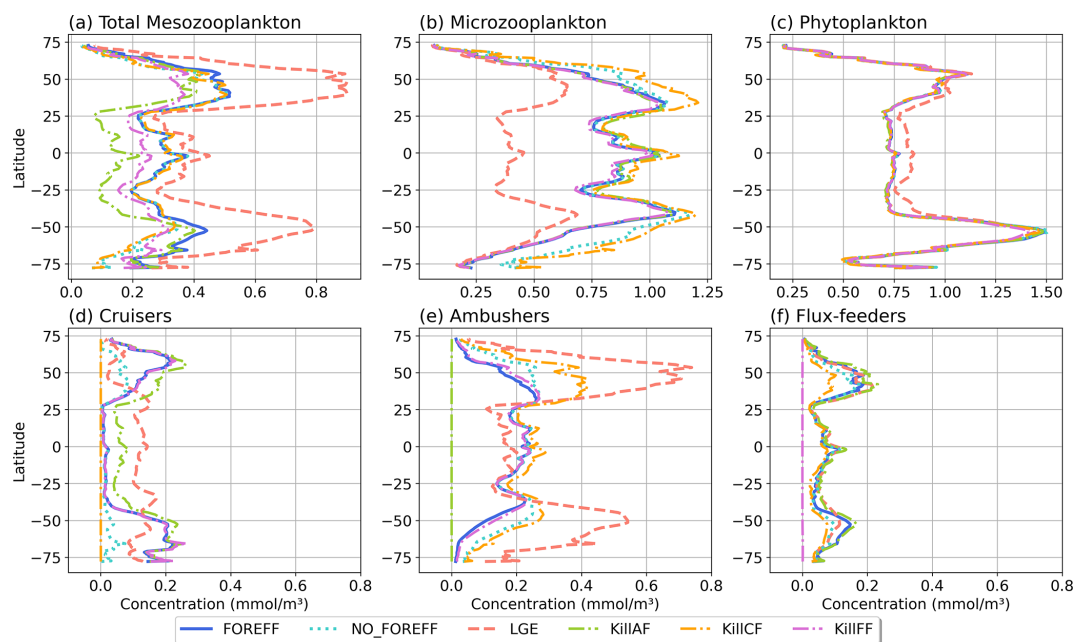
Figure A6. Annual and zonal average calculated over 150 m for different tracers in different experiments. (a) Total meso zooplankton, (b) microzooplankton, (c) phytoplankton, (d) cruisers, (e) ambushers, and (f) flux-feeders.
