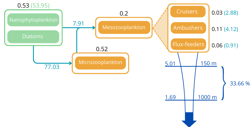
Figure A12. Representation of the global ecosystem dynamics in the FOREFF configuration. Values are in \text{GtCyr}^{-1} . Values in black correspond to the biomass of each plankton group integrated over the top 150 m. Values in blue correspond to grazing by zooplankton and in green to phytoplankton primary production, integrated over the top 150 m. Values in dark blue correspond to carbon export and efficiency.
