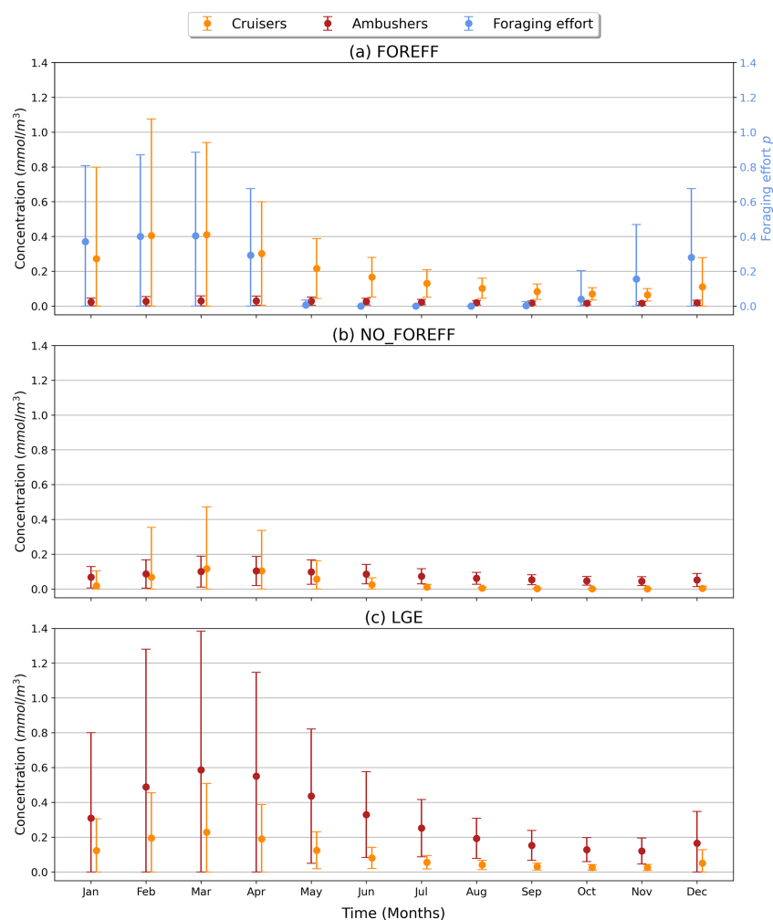
Figure A7. Time series (in months) averaged over the top 150 m of cruisers (orange) and ambushers (red) in Southern latitudes ( > 60^{\circ} S) for (a) FOREFF, (b) NO_FOREFF, and (c) LGE.
