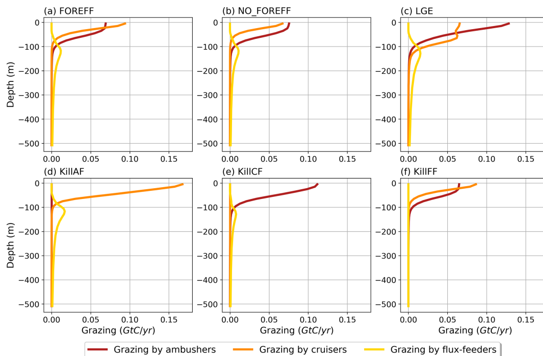
Figure A5. Annual and spatial mean of the total modelled grazing fluxes (in \text{GtCyr}^{-1} ) for the different meso zooplankton groups in (a) FOREFF, (b) NO_FOREFF, (c) LGE, (d) KILL_AF, (e) KILL_CF, and (f) KILL_FF.
