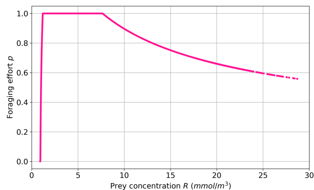
Figure 2. Foraging effort vs. prey concentration based on the parameter set of FOREFF (Table 1).
