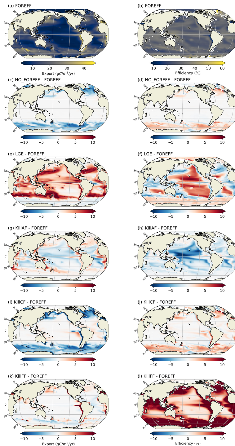
Figure A9. Annual mean of (a) FOREFF carbon export at 150 m difference in carbon export and (b) FOREFF carbon transfer efficiency between 150–1000 m. Difference between FOREFF and (c, d) NO_FOREFF, (e, f) LGE, (g, h) KILL_AF, (i, j) KILL_CF, and (k, l) KILL_FF in carbon export over 150 m (left) and carbon transfer efficiency between 150–1000 m (right).
