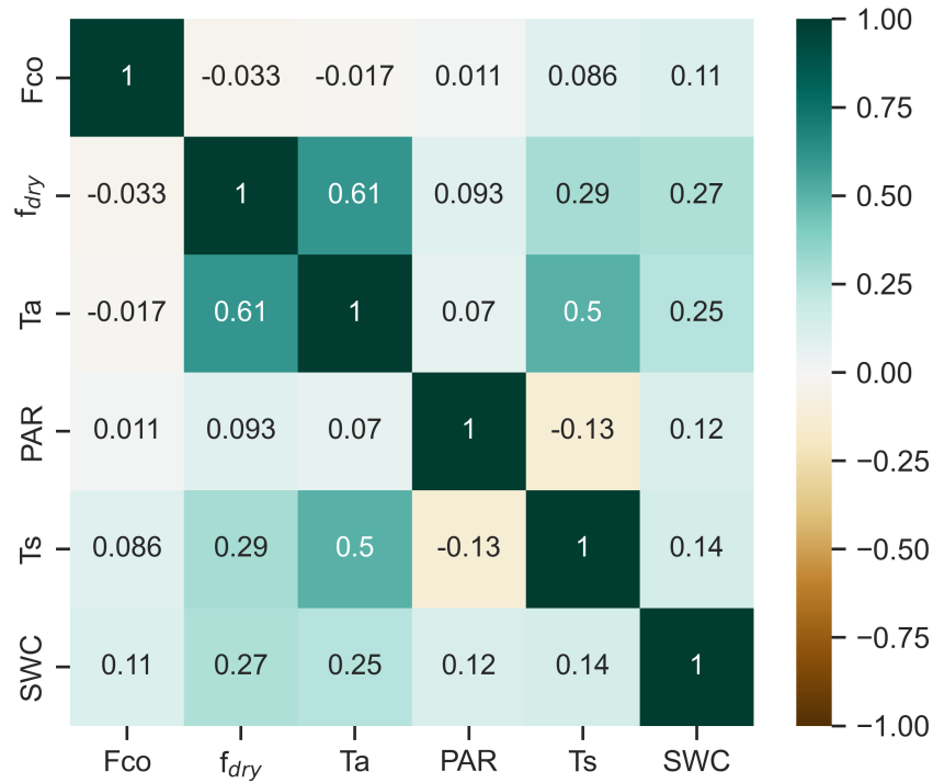
Figure S3: The correlation matrix of Spearman's rank correlation coefficients for wintertime CO flux (Fco) and flux drivers: soil temperature at a depth of 10 cm (Ts), soil water content at a depth of 10 cm (SWC), photosynthetically active radiation (PAR), air temperature (Ta), and fraction of dry surface area ( f_{dry} ) calculated for half-hourly values.
