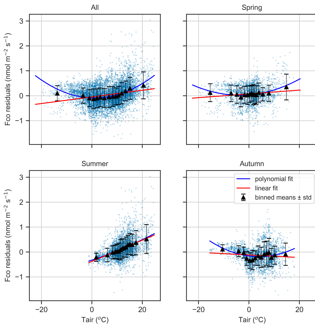
Figure S4: CO flux residuals from a linear model ( F_{co} = a \cdot \text{PAR} + c ) plotted against air temperature. Residuals are shown as 30-minute flux data (blue dots), aggregated into binned means \pm standard deviation (black triangle). Both least-squares linear (red) and second-degree polynomial (blue) fits are applied to the data.
