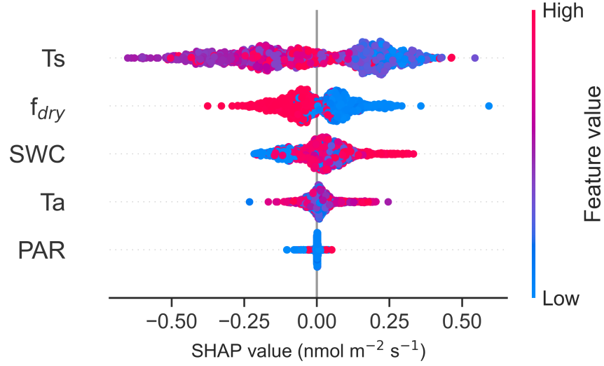
Figure S6: SHAP values of the nighttime RF model for CO flux drivers: photosynthetically active radiation (PAR), air temperature (Ta), soil temperature at a depth of 10 cm (Ts), soil water content at a depth of 10 cm (SWC) and fraction of dry surface area ( f_{dry} ). The SHAP values indicate the impact each feature has on the model output, with a negative value indicating a reduced flux and a positive value an increased flux. The blue color represents low feature values and red color high feature values. The zero line is the baseline (the average prediction). The SHAP values are calculated data from March to November and nighttime was defined as PAR < 1 \mu\text{mol m}^{-2}\text{s}^{-1} .
