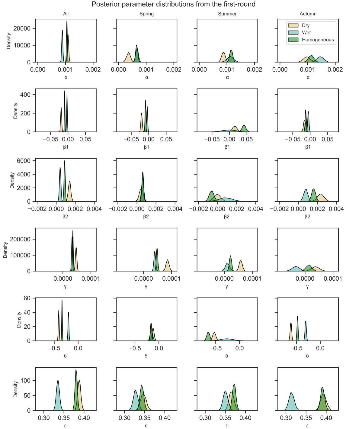
Figure S8: Posterior parameter distributions of the model parameters \alpha and \beta_1 , \beta_2 , \gamma , \delta , and residuals ( \epsilon ) after the first model run. The parameters are estimated separately for wet (turquoise) and dry (yellow). Homogeneous parameters represent the parameters without considering surface structure (green).
