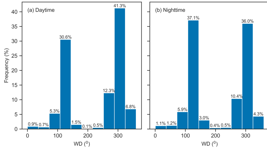
Figure S2: Wind direction distributions: a) daytime and b) nighttime including data from March to November.
