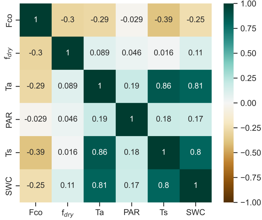
Figure S5: The correlation matrix of Spearman's rank correlation coefficients for nighttime CO flux (Fco) and flux drivers: soil temperature at a depth of 10 cm (Ts), soil water content at a depth of 10 cm (SWC), photosynthetically active radiation (PAR), air temperature (Ta), and fraction of dry surface area (fdry) calculated for half-hourly values. Nighttime was defined as \text{PAR} < 1 \mu\text{mol m}^{-2} \text{s}^{-1} .
