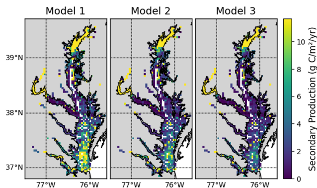
Figure C1. Long-term average secondary production across the Chesapeake Bay for each of the three secondary production models.
