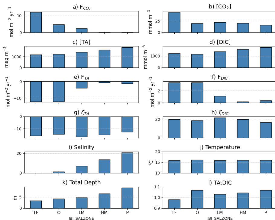
Figure E1. Carbon flux-related parameters averaged within salinity zones of Chesapeake Bay. [\text{CO}_2] was calculated using PyCO 2 SYS; temperature, salinity, total depth, [\text{TA}] and [\text{DIC}] were obtained from ROMS model output. F_{\text{TA}} and F_{\text{DIC}} were calculated following Eqs. (12)–(13), \zeta_{\text{TA}} and \zeta_{\text{DIC}} from Eqs. (15)–(16), and F_{\text{CO}_2} from Eq. (14).
