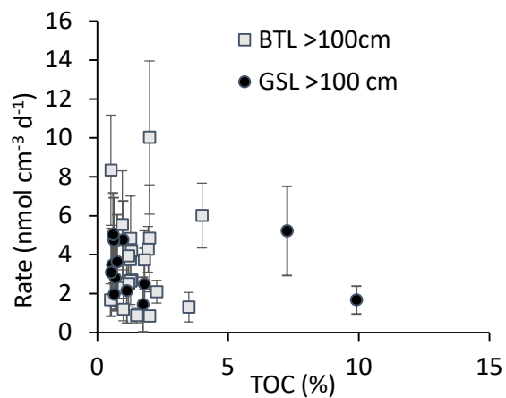
Figure S4: Methane production rates as a function of TOC in BTL and GSL depths greater than 100 cm. The CH 4 production rates between GSL and BTL are not significantly different.
