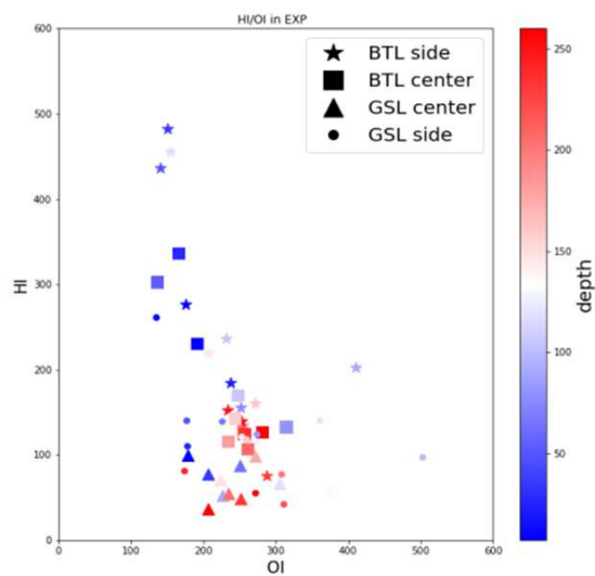
Figure S3: Hydrogen index (HI) versus oxygen index (OI) calculated from Rock Eval analyses at the study sites. The depths are marked as different colors. A decrease in HI and an increase in OI in greater depths and with lake aging is observed.
