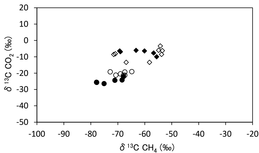
Figure S7: The \delta^{13}\text{C}_{\text{CO}_2} vs \delta^{13}\text{C}_{\text{CH}_4} in BTL (Circles) and GSL (Diamonds). Full symbols for Center, empty symbols for Edge of lake.
