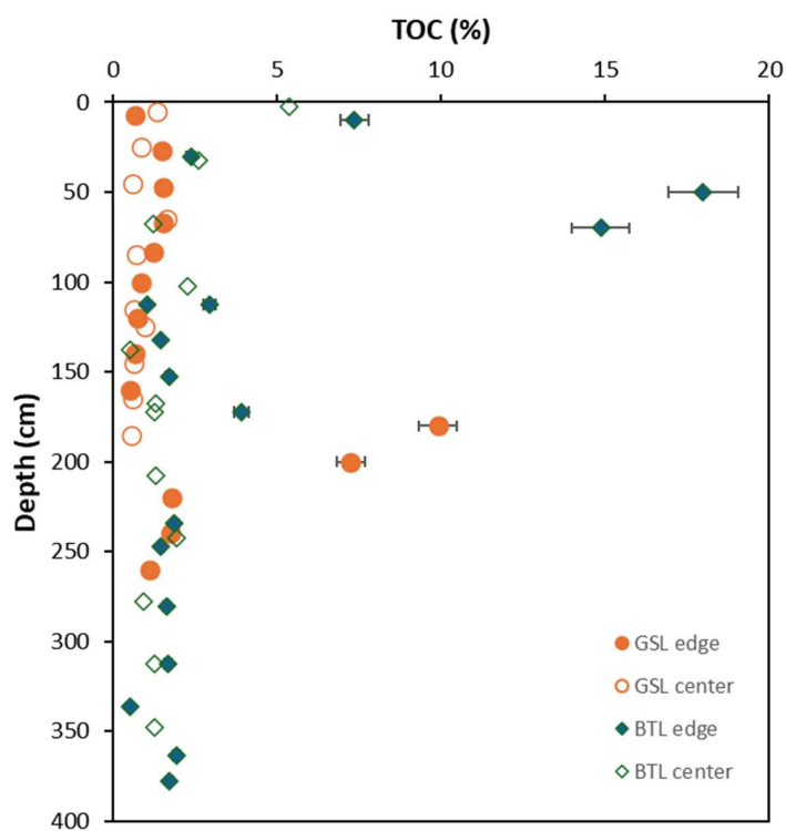
Figure S2: TOC percentage in cores.
