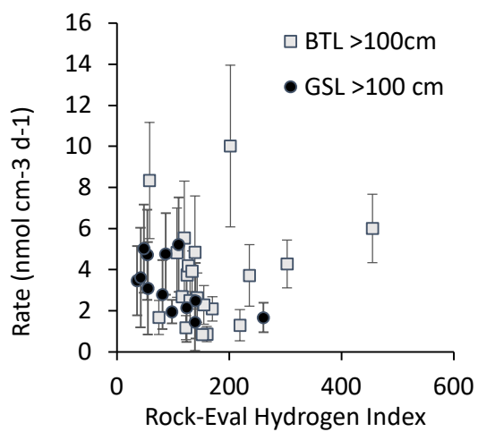
Figure S5: Methane production rates are not correlated to the lability of organic matter for thermal reactions, as indicated by the hydrogen index obtained by Rock Eval pyrolysis at depths greater than 100cm in GSL and BTL talik.
