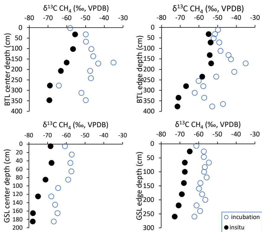
Figure S1: \delta^{13}\text{C}_{\text{CH}_4} profiles in situ and long term (90 days) incubations.
