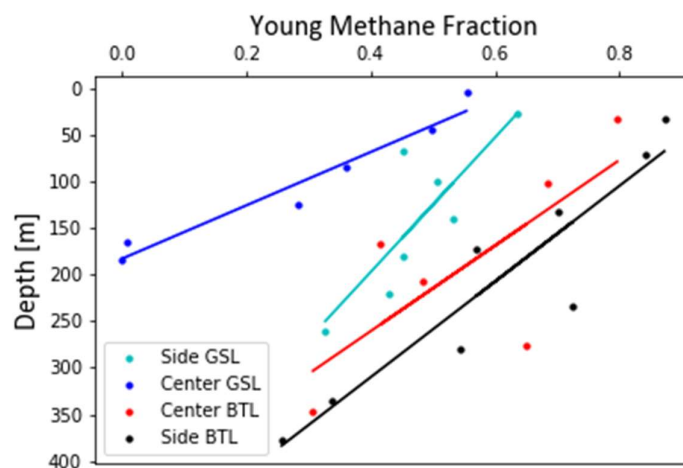
Figure S6: Newly Produced CH 4 Fraction in Each Core at Various Depths. Calculated from \delta^{13}\text{C}_{\text{CH}_4} measured in situ and from the incubation experiment. Blue dots denote GSL center core, light blue denotes GSL edge core, red dots denote BTL center core, and black dots denote BTL edge core. A similar color trend line has been fitted for each core. It can be observed that the fraction becomes smaller with depth, and the fraction is smaller as the core area matures.
