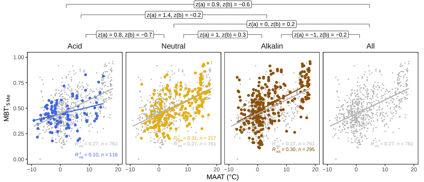
Figure S7. Effect of the alkalinity (i.e., the pH of each surface sample) on the linear relation between temperature (here MAAT) and the MBT'_{5Me}. Based on the alkalinity classes (i.e., acid, neutral, and alkaline), different temperature calibration MBT'_{5Me}-based are proposed following MAAT = a \times MBT'_{5Me} + b . Using the z -statistic with its p -value (Clogg et al., 1995), the significance of the difference between the slopes (a) of the linear regression is evaluated. Similarly, the z -statistic was used for the intercept (b) differences. For the p -values we have *** for p \leq 0.01 , ** for p \leq 0.05 and * for p \leq 0.1 .
