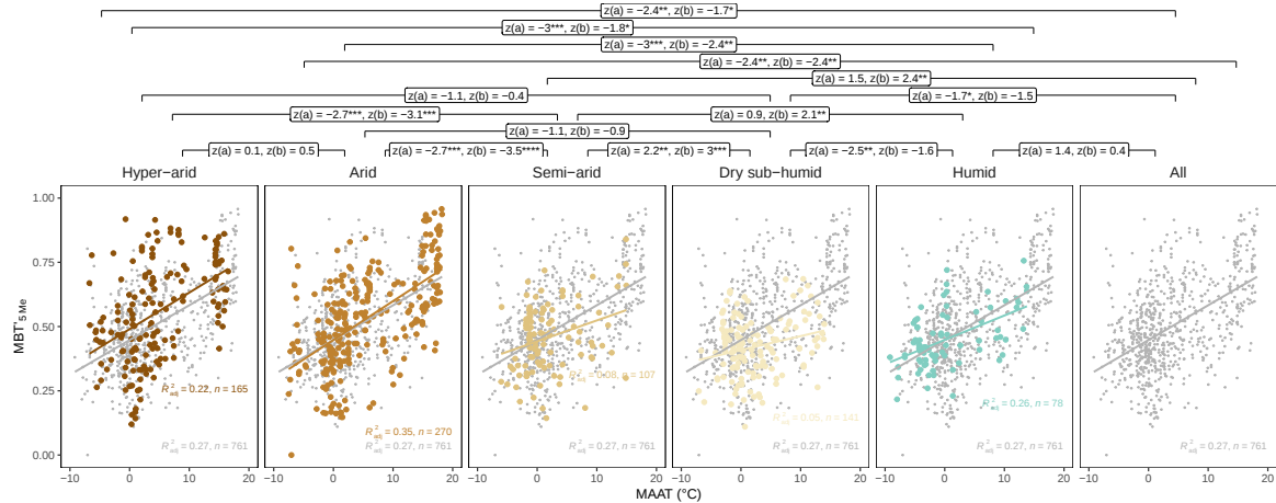
Figure S8. Effect of the aridity (i.e. the AI of each surface sample) on the linear relation between temperature (here MAAT) and the MBT'_{5Me}. Based on the aridity classes (i.e., hyper-arid, arid, semi-arid, dry sub-humid, and humid), different temperature calibration MBT'_{5Me}-based are proposed following MAAT = a \times MBT'_{5Me} + b . Using the z -statistic with its p -value (Clogg et al., 1995), the significance of the difference between the slopes (a) of the linear regression is evaluated. Similarly, the z -statistic was used for the intercept (b) differences. For the p -values we have *** for p \leq 0.01 , ** for p \leq 0.05 , and * for p \leq 0.1 .
