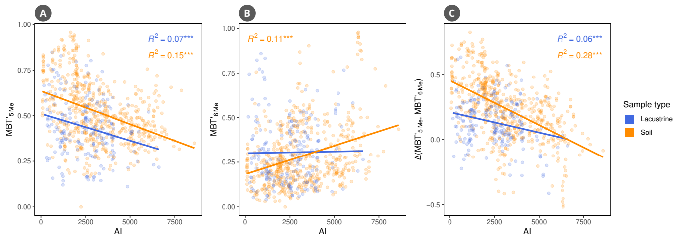
Figure S5. Relationships between the Aridity Index (AI) and Methylation indices, i.e. MBT'_{5Me} (A), MBT'_{6Me} (B), and \Delta(MBT'_{5Me}, MBT'_{6Me}) (C) linear relationships with AI. The regressions were tested for soil (orange) and lacustrine (blue) samples. Solely, the R^2 for significant regression ( p -value < 0.001) were displayed.
