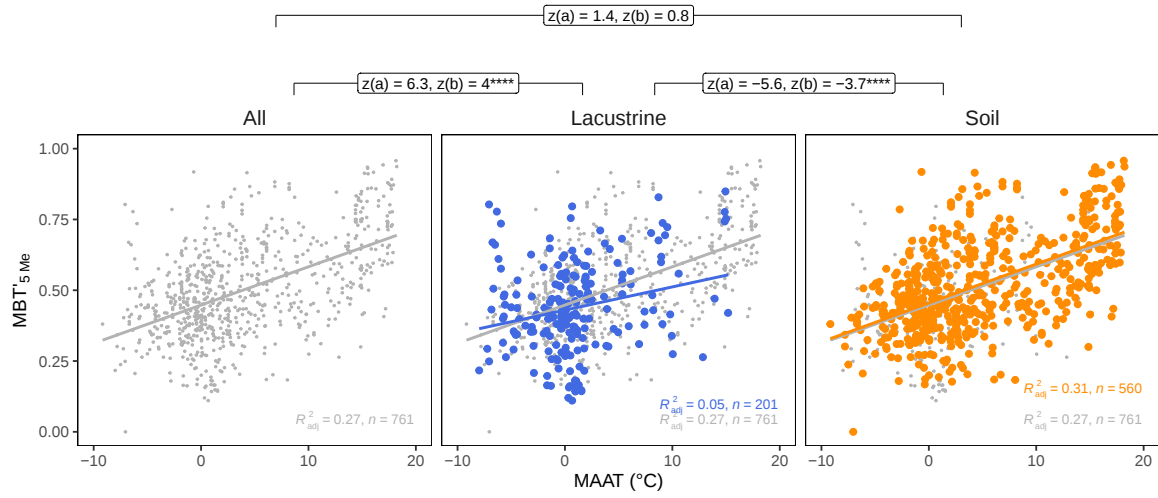
Figure S9. Effect of the sample type on the linear relation between temperature (here MAAT) and the MBT'_{5Me} . Based on the sample types (i.e., soil or lacustrine), different temperature calibration MBT'_{5Me} -based are proposed following MAAT = a \times MBT'_{5Me} + b . Using the z -statistic with its p -value (Clogg et al., 1995), the significance of the difference between the slopes (a) of the linear regression is evaluated. Similarly, the z -statistic was used for the intercept (b) differences. For the p -values we have *** for p \leq 0.01 , ** for p \leq 0.05 , and * for p \leq 0.1 .
