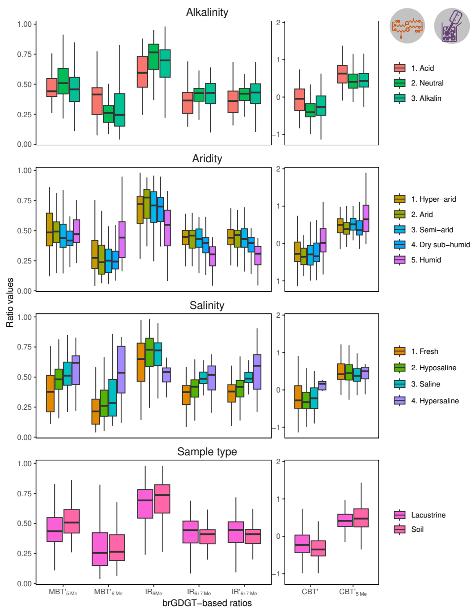
Figure S4. Boxplot for the main brGDGT-based ratios presented in this study clustered by the four grouping factors (i.e., alkalinity, aridity, salinity, and sample type). This figure is associated with the MANOVA and ANOVA results of Table 3.
