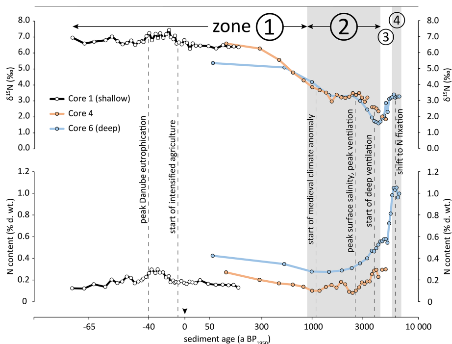
Figure 7. Evolution of N content and \delta^{15}\text{N} values in sediment cores 1, 4 and 6 from the NW shelf. Grey and white backgrounds indicate \delta^{15}\text{N}/[\text{N}] zones 1–4, additionally marked by circled numbers. Vertical dashed lines mark significant events mentioned in the discussion. Age scale is log transformed (see methods Sect. 2.6 for details).
