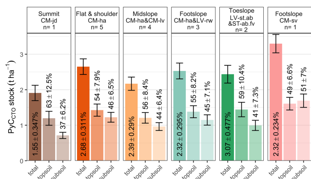
Figure 4. PyC CTO stocks in the soil profile down to 60 cm (darker shade), topsoil (0–30 cm, intermediate shade), and subsoil (30–60 cm, lighter shade) by soil group according to the gradient of soil evolution with slope position. CM – Cambisol, LV – Luvisol, ST – Stagnosol, jd – hyperdystric, ha – haplic, lv – luvic, rw – relectistagnic, st – stagnic, ab – albic, fv – fluvic, sv – solimovic. The numbers above the bars are the proportion of the topsoil (resp. subsoil) PyC stock in the total stock, the numbers inside the bars are the proportion of PyC stock in the total SOC stocks. Error bars represent the propagated standard error.
