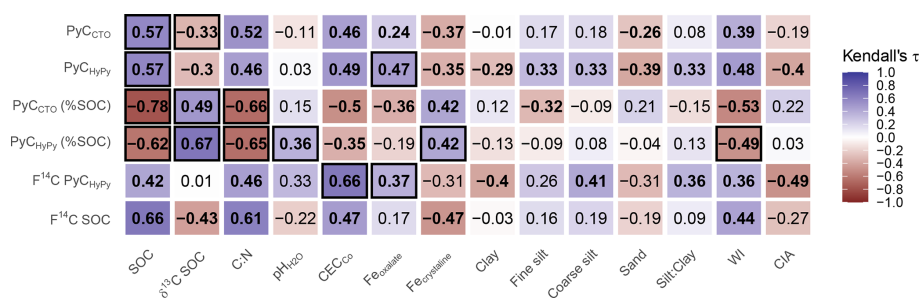
Figure 6. Kendall's rank correlation between PyC content (CTO and HyPy), PyC proportion in SOC (CTO and HyPy), F 14 C (PyC HyPy and bulk SOC) and selected soil characteristics, including SOC and indicators of SOC quality ( \delta^{13}\text{C} , C : N), soil chemistry (pH H2O , CEC Co , Fe oxalate and Fe crystalline ), soil texture (Clay to Sand) and soil evolution (Silt : Clay, weathering index WI and chemical index of alteration CIA), across depths. Significant correlations at the 95 % confidence level are in bold. Correlations that remain significant and of the same sign in at least one depth increment (0–10 or 50–60 cm) are outlined in black.
