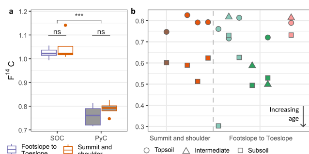
Figure 5. (a) F^{14}C of bulk SOC (white fill) and PyC H Py (grey fill) in the topsoil (0–10 cm) for upslope positions (orange) and downslope positions (purple). Two-sided Wilcoxon–Mann–Whitney test for the difference between C pools (***) – p < 0.01 and between slope positions within each pool (ns – not significant, p > 0.1 ). (b) F^{14}C of PyC H Py in topsoil (0–10 cm, circles), intermediate (20 to 40 cm depth, triangles) and subsoil (50 to 70 cm depth, squares) horizons in upslope and downslope positions. brown – Hyperdystric Cambisol at the summit, dark orange – Haplic Cambisols at intermediate flats and shoulders, aquamarine – Haplic Cambisol and relectistagnic Luvisols and the footslope, green – Stagnic Albic Luvisol and Albic Fluvic Stagnosol at the toeslope and pink – Solimovic Cambisol at the footslope. Note the different x-axis scale between the two panels.
