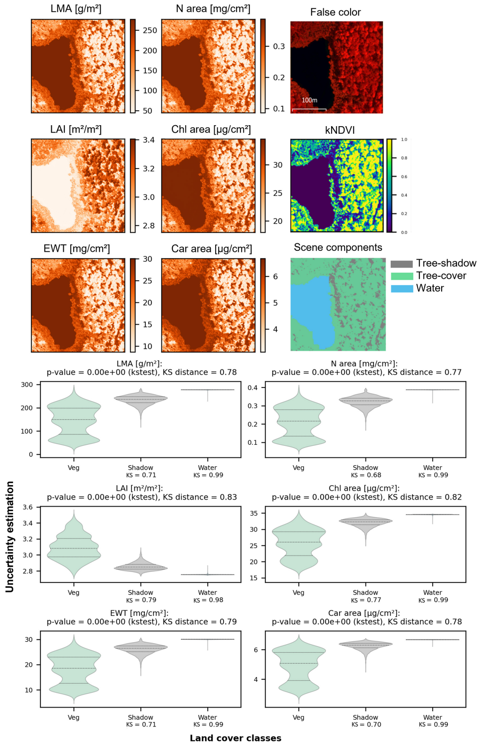
Figure 5. NEON scene (Right panels) Description of the scene including false-color composite highlighting vegetation in red, kernel normalized difference vegetation index (kNDVI) map showing higher values for denser vegetation area, and component scene map. (Left panels) Spatial distribution of uncertainty estimation for six plant traits: Leaf Mass per Area (LMA), Nitrogen content (N), Leaf Area Index (LAI), Chlorophyll content (Chl), Equivalent Water Thickness (EWT), and Carotenoid content (Car), showing how uncertainty varies across the scene. (Bottom panels) Trait-wise violin plots of predicted uncertainty distributions from randomly sampled pixels across the scene components. To evaluate the plausibility of uncertainty estimates, Kolmogorov–Smirnov (KS) distances measure the separability between vegetation and non-vegetation distributions, while KS p -values indicate whether these differences are statistically significant.
