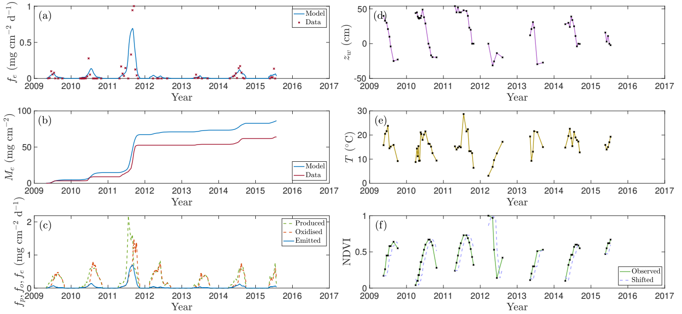
Figure S4: Baseline predictions for the centre of the T5 wetland. Panel (a) shows the modelled (blue line) and observed (red crosses; based on data from Bansal and Tangen, 2022) \text{CH}_4 fluxes over the growing seasons 2009–2016, the associated cumulative \text{CH}_4 emissions from the solver (blue line) and approximated from integration of the data (red line) are shown in panel (b). The rate of \text{CH}_4 production and oxidation in the soil column and \text{CH}_4 emissions from the soil column are summarised in panel (c). Each of these model predictions are forced by the drivers water table depth (panel d), temperature (panel e) and NDVI (panel f). Crosses in panels (d–f) reflect observed data, whilst lines show interpolated data between data points. The shifted NDVI used to infer the available carbon substrate for methanogenesis is shown by the dashed line in panel (f).
