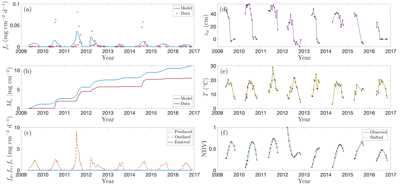
Figure S5: Baseline predictions for the centre of the T6 wetland. Panel (a) shows the modelled (blue line) and observed (red crosses; based on data from Bansal and Tangen, 2022) \text{CH}_4 fluxes over the growing seasons 2009–2016, the associated cumulative \text{CH}_4 emissions from the solver (blue line) and approximated from integration of the data (red line) are shown in panel (b). The rate of \text{CH}_4 production and oxidation in the soil column and \text{CH}_4 emissions from the soil column are summarised in panel (c). Each of these model predictions are forced by the drivers water table depth (panel d), temperature (panel e) and NDVI (panel f). Crosses in panels (d–f) reflect observed data, whilst lines show interpolated data between data points. The shifted NDVI used to infer the available carbon substrate for methanogenesis is shown by the dashed line in panel (f).
