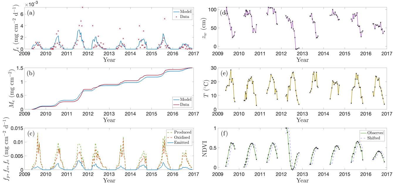
Figure S2: Baseline predictions for the centre of the P3 wetland. Panel (a) shows the modelled (blue line) and observed (red crosses; based on data from Bansal and Tangen, 2022) \text{CH}_4 fluxes over the growing seasons 2009–2016, the associated cumulative \text{CH}_4 emissions from the solver (blue line) and approximated from integration of the data (red line) are shown in panel (b). The rate of \text{CH}_4 production and oxidation in the soil column and \text{CH}_4 emissions from the soil column are summarised in panel (c). Each of these model predictions are forced by the drivers water table depth (panel d), temperature (panel e) and NDVI (panel f). Crosses in panels (d–f) reflect observed data, whilst lines show interpolated data between data points. The shifted NDVI used to infer the available carbon substrate for methanogenesis is shown by the dashed line in panel (f). Optimised parameters are detailed in Table 1 of the main text.
