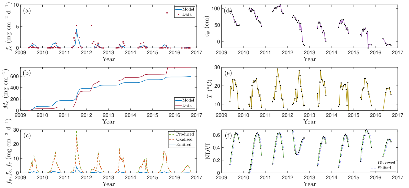
Figure S6: Baseline predictions for the centre of the T9 wetland. Panel (a) shows the modelled (blue line) and observed (red crosses; based on data from Bansal and Tangen, 2022) \text{CH}_4 fluxes over the growing seasons 2009–2016, the associated cumulative \text{CH}_4 emissions from the solver (blue line) and approximated from integration of the data (red line) are shown in panel (b). The rate of \text{CH}_4 production and oxidation in the soil column and \text{CH}_4 emissions from the soil column are summarised in panel (c). Each of these model predictions are forced by the drivers water table depth (panel d), temperature (panel e) and NDVI (panel f). Crosses in panels (d–f) reflect observed data, whilst lines show interpolated data between data points. The shifted NDVI used to infer the available carbon substrate for methanogenesis is shown by the dashed line in panel (f).
