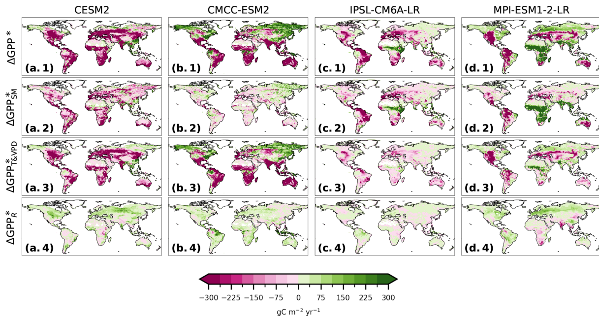
Figure 6. Contribution analysis estimate for LFMIP of the total changes in GPP due to SM ( \Delta\text{GPP}^* ) and the individual contributions from the direct SM effect ( \Delta\text{GPP}_{\text{SM}}^* ), the indirect SM effects via VPD and T ( \Delta\text{GPP}_{T\&VPD}^* ), and via R ( \Delta\text{GPP}_R^* ) for the future period (2070–2099). Pink indicates a reduction and green an increase of NBP due to SM. White indicates no data.
