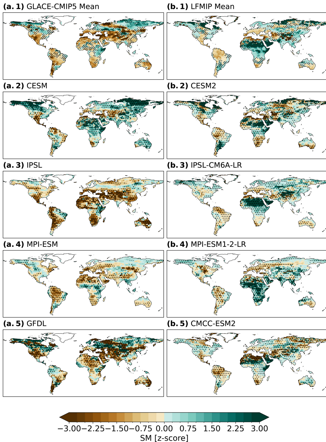
Figure 3. SM changes in standard deviations ( z -score) from the control simulation for the future period (2070–2099) relative to the baseline period (1981–2010) for (a.1) the GLACE-CMIP5 mean, (b.1) the LFMIP mean, (a.2–5) individual model projections of GLACE-CMIP5, and (b.2–5) individual model projections of LFMIP. Brown indicates drying and green wetting relative to the pre-industrial period. White indicates no data. In (a.1) and (b.1) hatching indicates less than 75 % agreement in the sign of change across models for the future period relative to the baseline period. In (a.2–5) and (b.2–5) stippling indicates areas where changes in SM for the future period differ significantly from the baseline period at the 5 % level (two-sided Welch's t -test).
