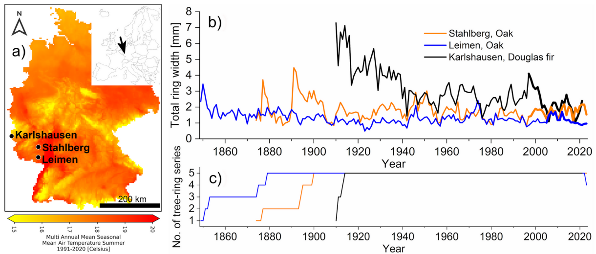
Figure 1. Area of interest and tree growth dynamic. (a) Map color shows the mean air summer temperature in the reference period 1991–2020 and the geographical location of the three sites. (b) Mean total ring width of oaks and Douglas firs at the different sites. (c) Number of used tree-ring series available per year.
