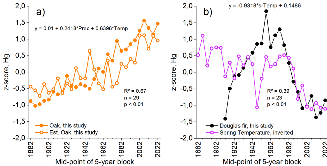
Figure 5. Climate response of tree-ring mercury (Hg) concentration variability for oak (a) and Douglas fir (b). Tree-ring Hg concentration in oak trees can be estimated by spring–summer mean air temperature (Temp) and spring–summer precipitation sum (Prec) and by spring mean air temperature (s-Temp) for Douglas fir trees (b).
