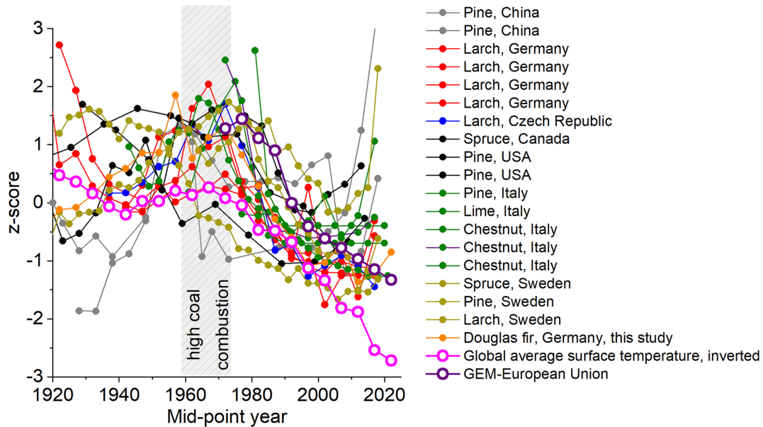
Figure 4. Records of tree-ring mercury concentration (filled points) at different sites in the Northern Hemisphere (colors refer to countries) (Scanlon et al., 2020; Chellman et al., 2020; Ghotra et al., 2020; Nováková et al., 2021; Wang et al., 2021; Baroni et al., 2023; Peng et al., 2024; Fornasaro et al., 2023) and records (circles) of global average surface temperature (inverted) and atmospheric mercury concentration emitted in the European Union. The grey shaded area shows the period of intense coal combustion in Europe according to Streets et al. (2017).
