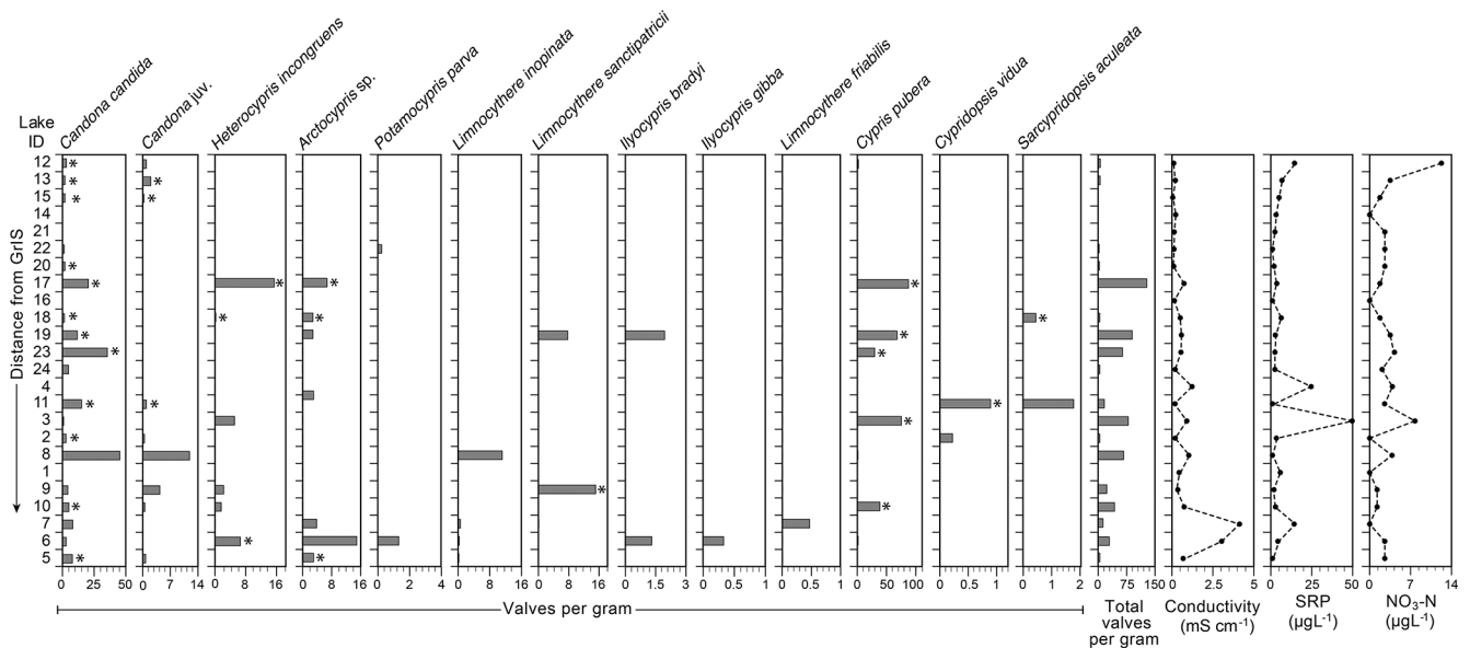
Figure 3. Ostracod species abundance as valves per gram in each of the 24 study lakes alongside selected recorded environmental variables (electrical conductivity, soluble reactive phosphorus (SRP) and nitrate (NO 3 -N)). The stars indicate the occurrence of individuals with soft parts, suggesting that they were collected alive. Table S2 provides a detailed breakdown of valves, carapaces and individuals with soft parts. Lakes are ordered in the distance from the Greenland Ice Sheet.
