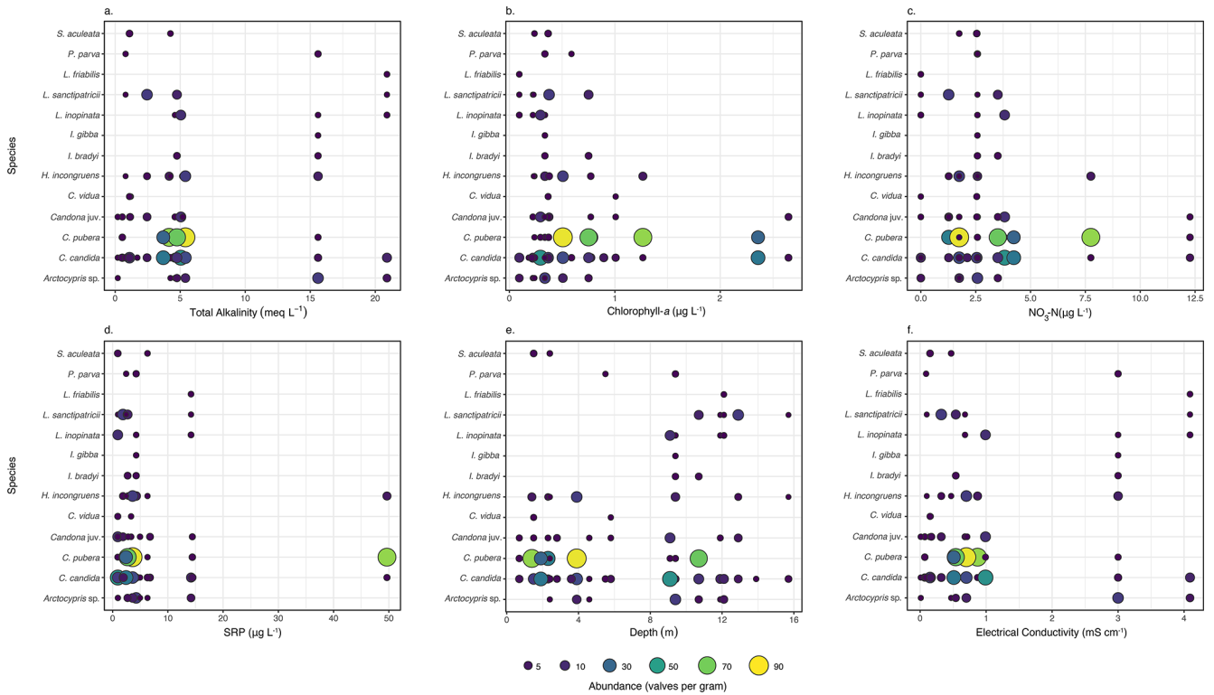
Figure 4. Abundance of ostracod species along gradients of (a) total alkalinity, (b) chlorophyll- a concentration, (c) nitrate (NO 3 -N) concentration, (d) soluble reactive phosphorus (SRP) concentration, (e) water depth and (f) electrical conductivity. Ostracod abundance is given in valves per gram and includes all specimens collected. Table S2 provides a detailed breakdown of valves, carapaces and individuals with soft parts.
