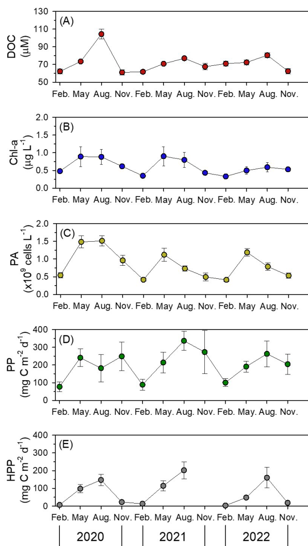
Figure 4. Seasonal variations of dissolved organic carbon (DOC) concentrations with values averaged to the mixed layer depth (a), chlorophyll a (Chl a ) concentrations (b), and prokaryotes abundance (PA) (c) averaged within the euphotic depth, primary production (PP) (d), and heterotrophic prokaryotes production (HPP) (e) values integrated over the euphotic depth in the northern East China Sea. Error bars represent standard errors.
