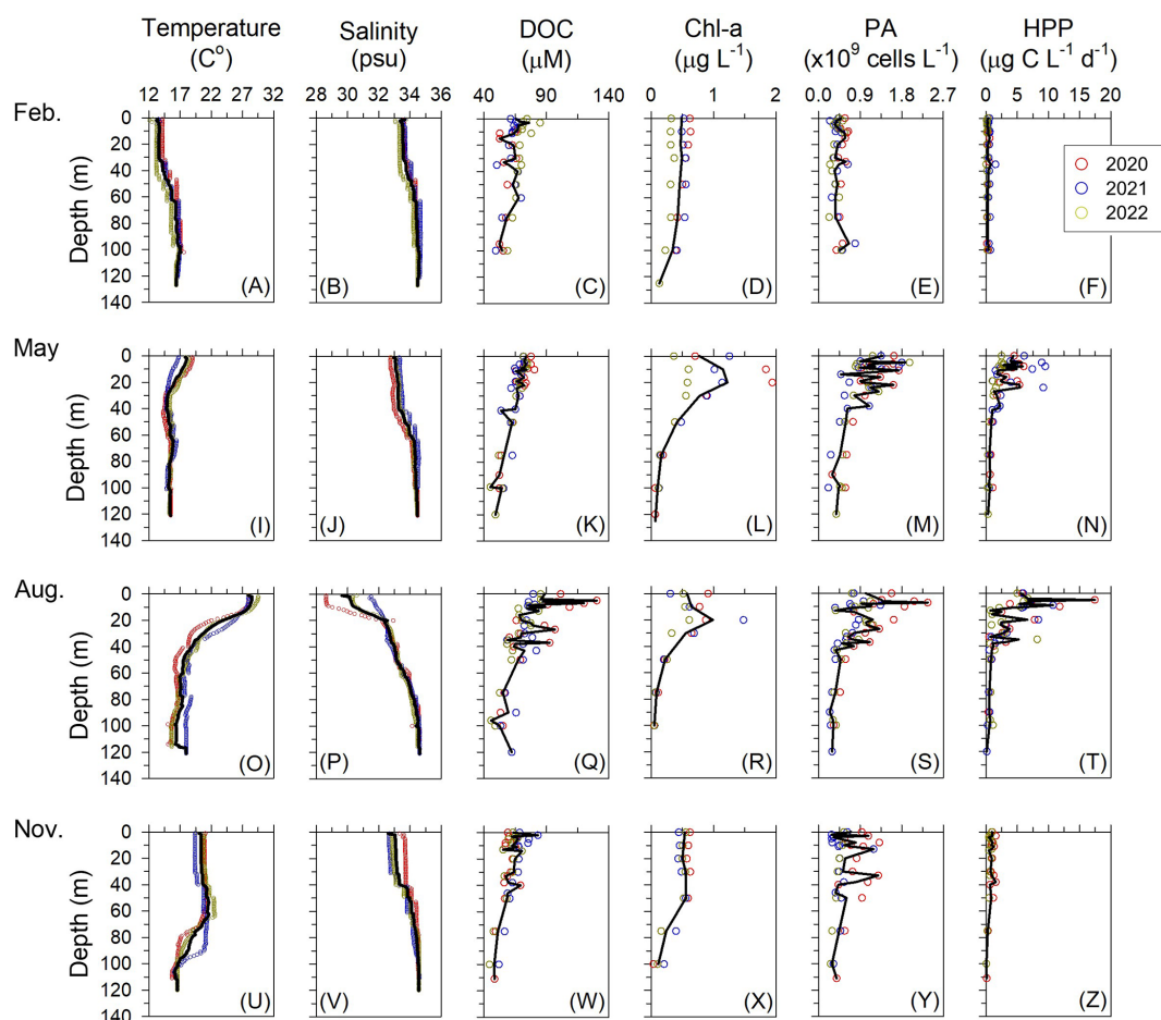
Figure 3. Vertical profiles of temperature, salinity, dissolved organic carbon (DOC), chlorophyll a (Chl a ), heterotrophic prokaryotes abundance (PA), and heterotrophic prokaryotes production (HPP) in the northern East China Sea from 2020 to 2022. Each symbol represents the average value at a given depth from 7–8 stations sampled during each survey, and the solid black line denotes the mean of the three-year averages.
