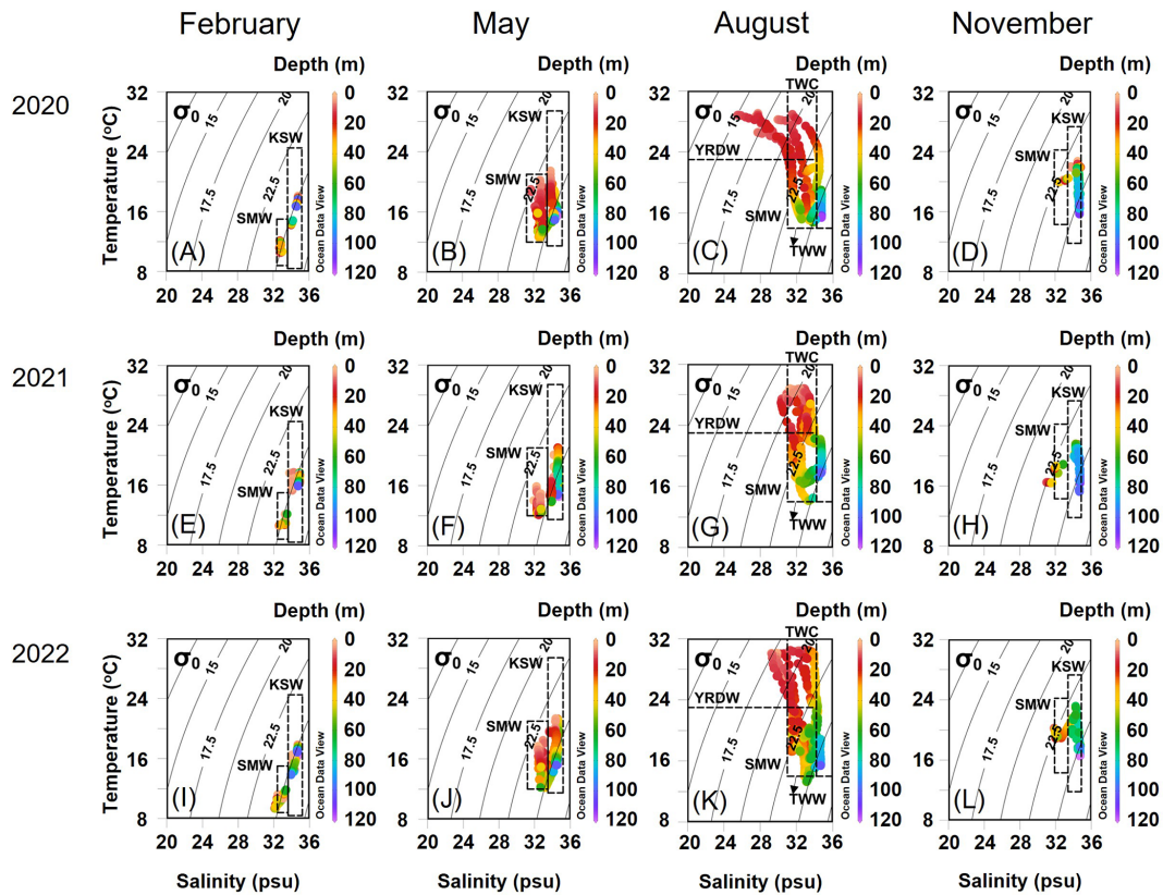
Figure 2. Seasonal T - S diagrams of the East China Sea (ECS) in 2020 (a–d), 2021 (e–h), and 2022 (i–l). The dashed box indicates the defined water masses in this study observed in the northern ECS (Gong et al., 1996; Hur et al., 1999; Kim and Youn, 2023). Grey contour lines represent the \sigma - t . The color bar indicates the depth of the water column. KSW: Kuroshio source water, SMW: Shelf mixed water, YRDW: Yangtze River diluted water, TWW: Tsushima warm water, TWC: Taiwan warm current.
