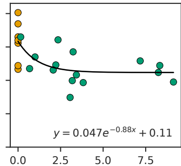
13 CS 2
