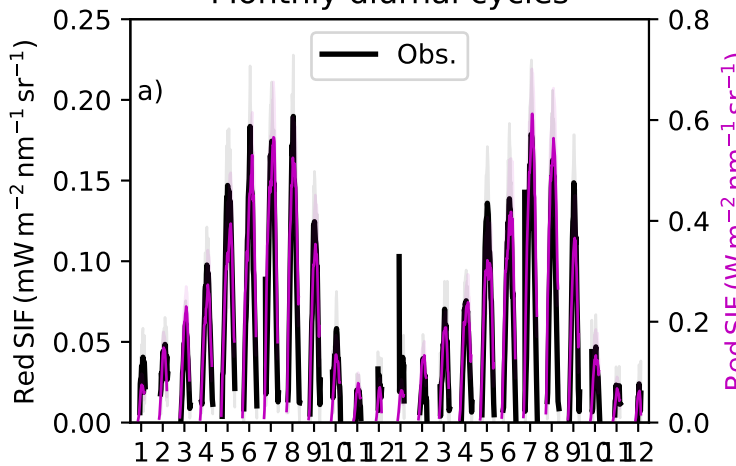
Monthly diurnal cycles
