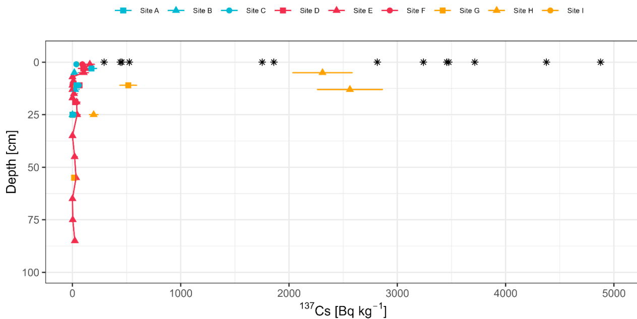
Figure S15. 137 Cs distribution in our cores [Bq kg -1 ]. The * symbols indicate peak values of total 137 Cs deposition observed in deeper areas of the studied lakes (Junna et al., in press ).
