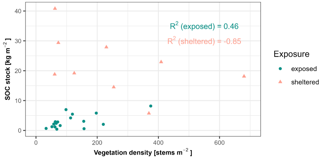
Figure S24. Comparison between sedimentary organic carbon (SOC) [ \text{kg m}^{-2} ] and vegetation density [ \text{stems m}^{-2} ], grouped by average fetch length (“exposed”: fetch > 500 m; “sheltered”: fetch \leq 500 m).
