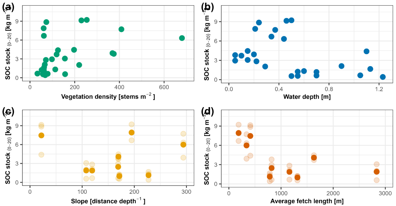
Figure S21. Relationship between sedimentary organic carbon (SOC) stocks [kg m -2 ] based on the top 20 cm of the sediment cores and environmental parameters: (a) vegetation density [number of helophyte stems, in stems m -2 ], (b) water depth [m], (c) slope (calculated as the distance between the landside and waterside sampling locations divided by the difference in their depth), (d) and the average fetch length [m]. In plots (c) and (d), the translucent points indicate the SOC stocks per zone (landside, transitional, waterside) in each site (A to I), while the opaque points indicate the average SOC stock estimates in each site.
