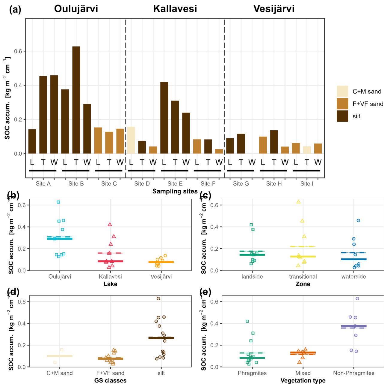
Figure S19. Sedimentary organic carbon (SOC) accumulation [ \text{kg m}^{-2} \text{cm}^{-1} ] of the sediment cores (a) and grouped by lakes (b), shoreline zones (c), grain size classes (d) and vegetation type (e). Accumulation estimates consider only samples with > 1\% of organic matter. In panels (b) to (e), the dashed horizontal lines indicate the mean, and the continuous bold horizontal lines indicate the median. Abbreviations: L = landside zone; T = transitional zone; W = waterside zone; C+M sand = coarse and medium sands; F+VF sand = fine and very fine sands. In (a), the bars are coloured according to the grain size averaged through the whole sediment core.
