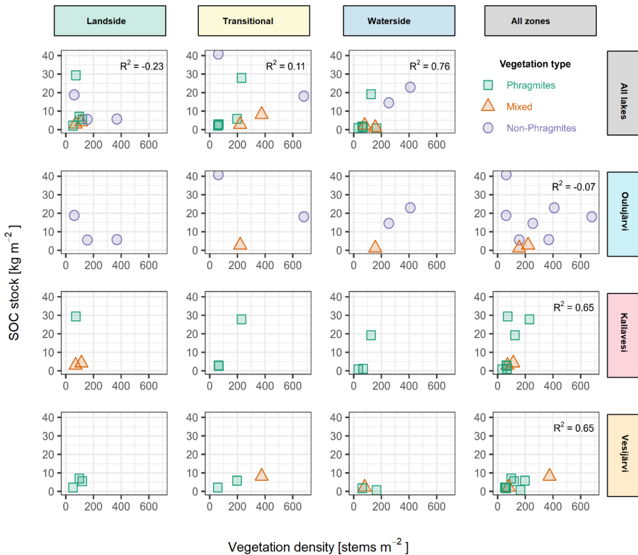
Figure S20. Comparison between sedimentary organic carbon (SOC) [kg m -2 ] and vegetation density [stems m -2 ], grouped by zones (columns), lakes (rows) and type of vegetation (symbol colours).
