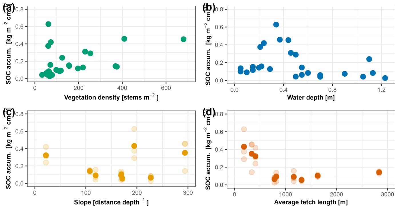
Figure S22. Relationship between sedimentary organic carbon (SOC) accumulation [ \text{kg m}^{-2} \text{cm}^{-1} ] and environmental parameters: (a) vegetation density [number of helophyte stems, in stems \text{m}^{-2} ], (b) water depth [m], (c) slope (calculated as the distance between the landside and waterside sampling locations divided by the difference in their depth), (d) and the average fetch length [m]. In plots (c) and (d), the translucent points indicate the SOC stocks per zone (landside, transitional, waterside) in each site (A to I), while the opaque points indicate the average SOC stock estimates in each site.
