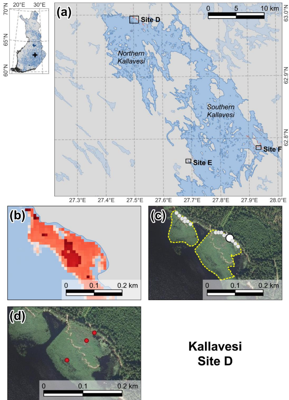
Figure S4. Location of sampling Site D in Kallavesi (a), with details of: (b) the vegetation patch (Koponen et al., 2022); (c) the starting points of the transect following a grid of 10 x 10 m; (d) the location of the sediment cores following the transect of landside, transitional and waterside. Aerial images from Finnish National Geoportal (Orthophotos) (2023).
