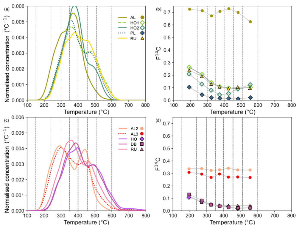
Figure 3. (a, c) Thermograms showing the concentration of CO 2 (as area normalized concentration per °C) as a function of temperature during progressive thermal oxidation of samples from thaw slumps FM2 (a) and FM3 (c). Colours indicate feature type: active layer (AL), debris (DB), runoff (RU), and permafrost (PF), including Holocene (HO) and Pleistocene (PL) samples and line styles distinguish samples with the same geomorphological feature. All thermograms are normalised to the same integrated area, following the method of Hemingway et al. (2017). (b, d) Radiocarbon content (F 14 C) measured across thermal decomposition windows for FM2 (b) and FM3 (d). Symbol shapes represent geomorphological features: circle = AL, square = DB, triangle = RU, diamond = PF (for FM2 – open = HO; filled = PL) and measurement uncertainties are too small to be displayed.
