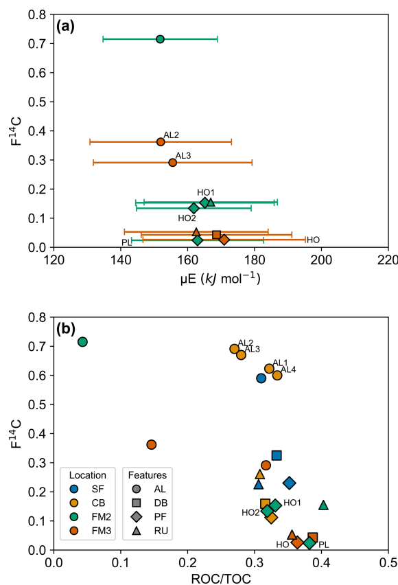
Figure 5. Panel (a): Relationship between F^{14}C and mean activation energy ( \mu_E ) across thaw slump samples from the Peel Plateau. Horizontal error bars represent the standard deviation ( \sigma_E ) of the activation energy distributions, reflecting the energetic heterogeneity of OM thermal decomposition. Panel (b): Bulk F^{14}C values (from Bröder et al., 2021) are compared with ROC/TOC ratios from SoliTOC measurements (see definition in the text) across four thaw slump locations and their respective features. Different features are indicated by shapes: circles represent active layer (AL), squares debris (DB), diamonds permafrost (PF), and triangles runoff (RU). Colours correspond to sampling locations: blue for SF, orange for CB, green for FM2, and red for FM3.
