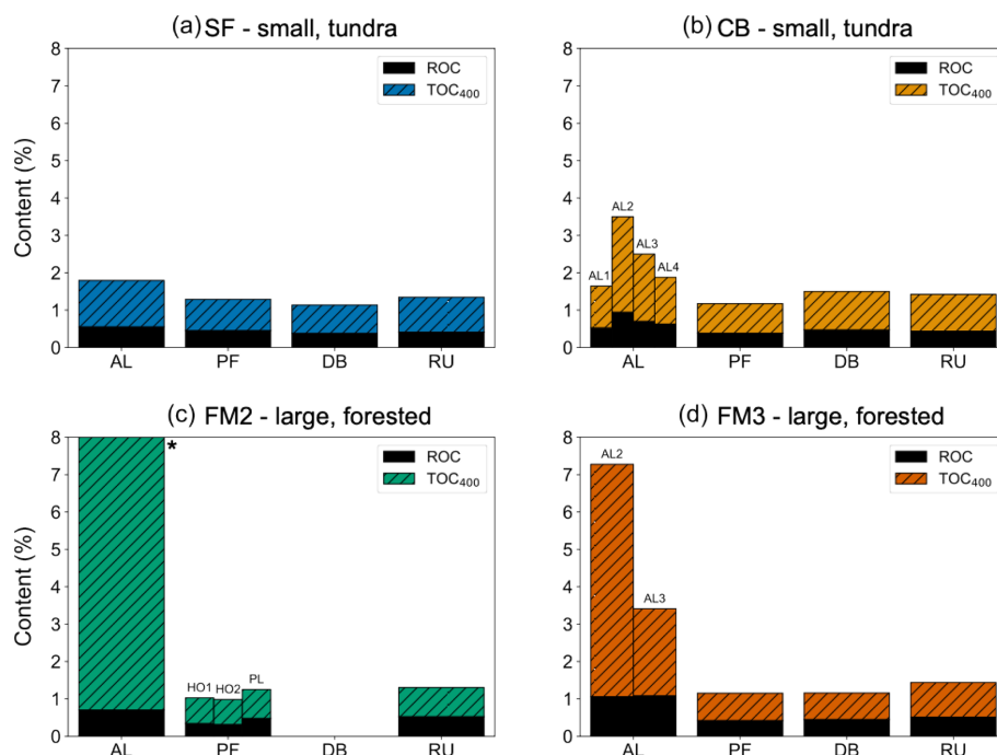
Figure 2. Carbon content in thaw slump samples as measured by Solid total organic carbon (SoliTOC) analysis. Bars represent thermally labile organic carbon (TOC 400 ; coloured) stacked above residual organic carbon (ROC; black), expressed as percent (%) of C content. Each panel (a)–(d) corresponds to one thaw slump site – SF (blue), CB (yellow), FM2 (green), and FM3 (red) – with bars grouped by geomorphological feature: active layer (AL), permafrost (PF), debris (DB), and runoff (RU). For FM2, both Holocene and Pleistocene permafrost layers were accessible in the field and are shown separately. Where multiple samples were collected from the same feature, individual sample names are indicated above each bar. * The active layer sample from FM2 exhibited exceptionally high TOC 400 content (> 15%), far exceeding values measured in other geomorphological units or sites, and contributing to a combined TOC 400 + ROC content of approximately 16%.
