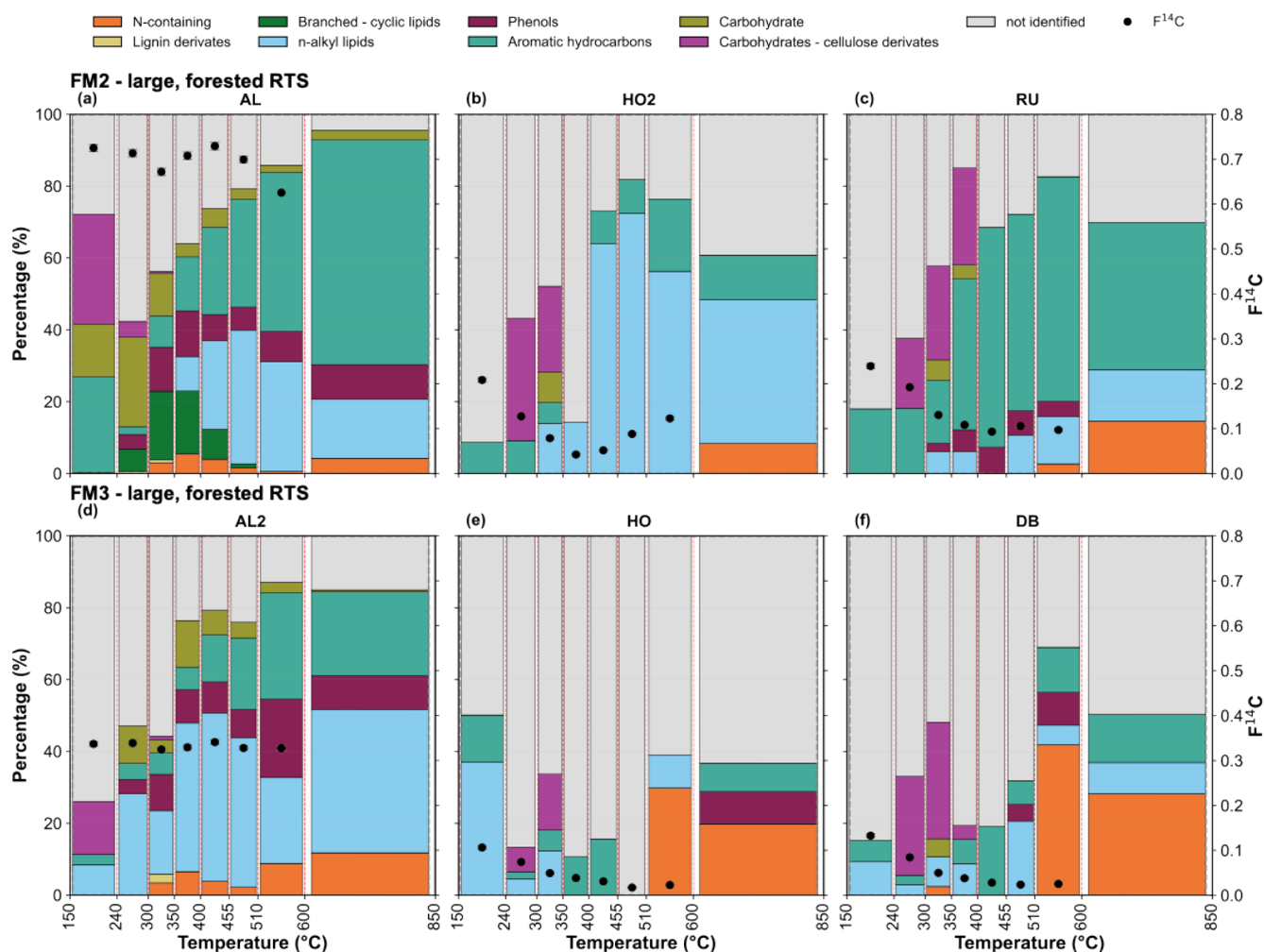
Figure 4. Normalized peak area distributions of molecular compound classes across thermal windows (150–850 °C) for selected thaw slump features (a–c) FM2: active layer (AL), deeper Holocene permafrost (HO2), and runoff (RU). (d–f) FM3: active layer (AL2), Holocene permafrost (HO), and debris (DB). Compound classes include nitrogen-containing compounds, lignin derivatives, branched–cyclic lipids, n -alkyl lipids, phenols, aromatic hydrocarbons, carbohydrates, and cellulose derivatives, with the F^{14}C fractions measured with ORO on the right. The combined presentation is intended to relate molecular composition to thermal stability and radiocarbon age, rather than to imply direct equivalence between fractions obtained by pyrolysis and combustion-based methods.
