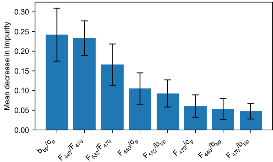
Feature importances using MDI
