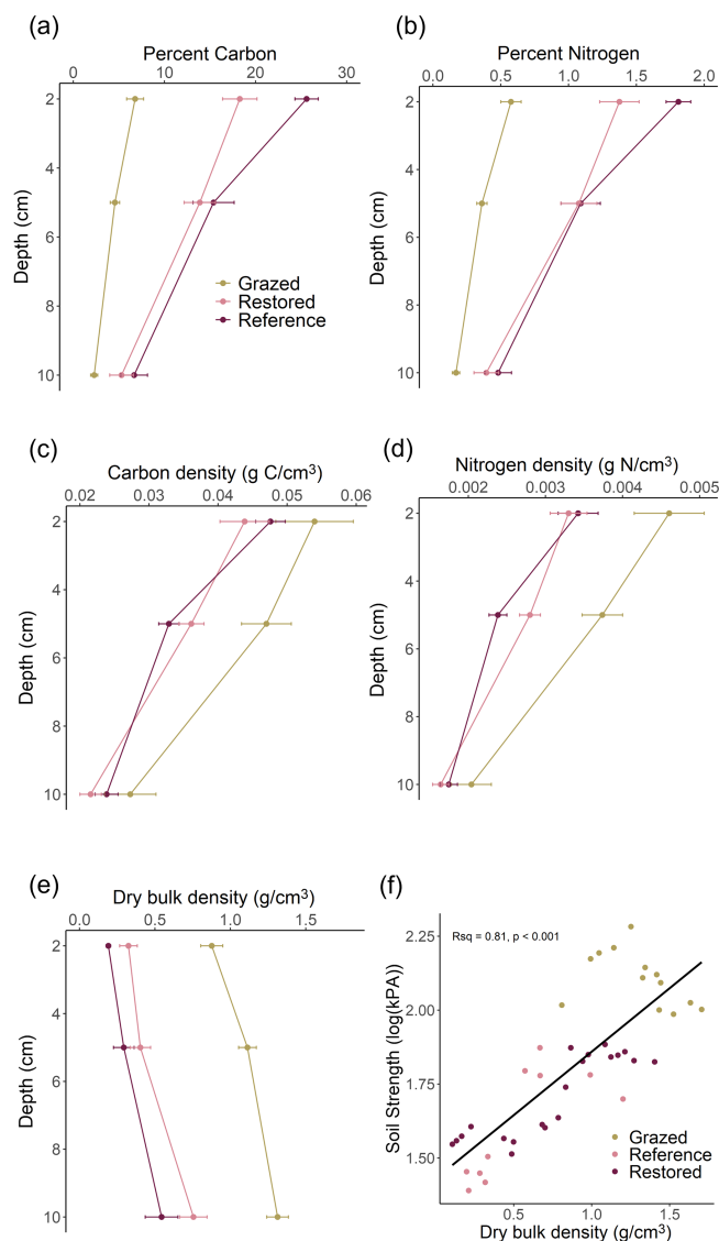
Figure 2. Top 10 cm saltmarsh soil characteristics at Grazed, Restored and Natural Reference sites. (a) Elemental percent organic carbon. (b) Elemental percent nitrogen. (c) Organic carbon density. (d) Nitrogen density. (e) Dry bulk density. Data represent means and standard error. (f) Relationship between dry bulk density and soil strength at ~10 cm depth. Note the log scale of soil strength. The line represents Pearson's correlation.
