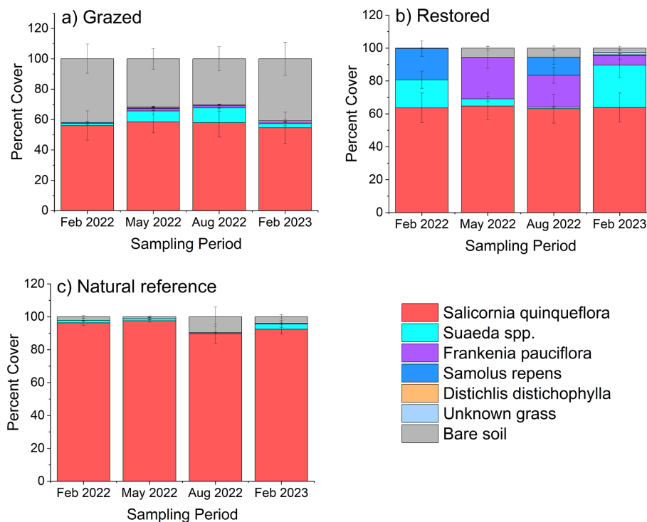
Figure 3. Saltmarsh vegetation cover over one year at (a) Grazed, (b) Restored and (c) Natural Reference sites. Vegetation surveys were taken of the experimental plots at initial, 3-, 6- and 12-month sampling periods. Data represent mean and standard error.
