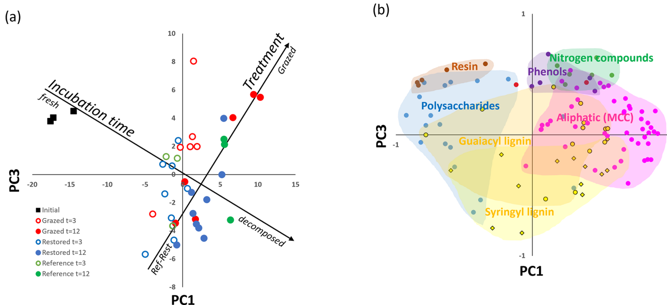
Figure 6. PC1–PC3 plots from principal components analysis of the molecular composition using pyrolysis-GC-MS of S. quinqueflora roots during one year of decomposition. (a) PC scores of the samples; (b) PC loadings of the pyrolysis products. MCC refers to methylene chain compounds (aliphatic organic matter).
