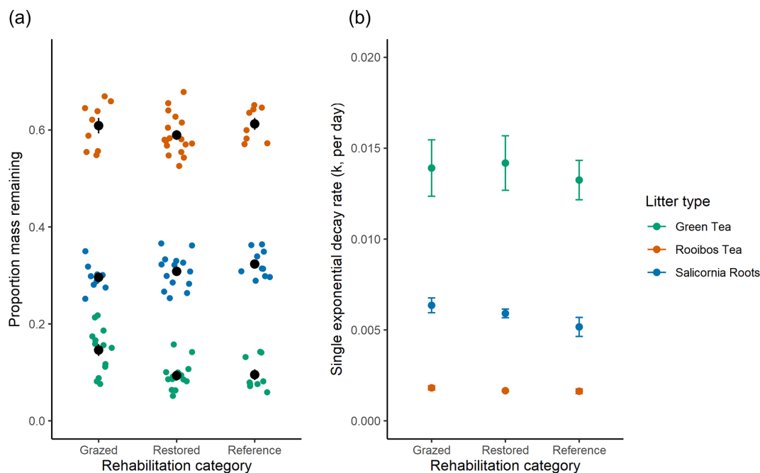
Figure 4. Decomposition parameters over 1 year of green tea, rooibos tea and S. quinqueflora root litters. (a) Proportion of mass remaining of litters after 12 months of decay. Coloured circles are raw values with central black circles representing mean and standard error for the litters at each rehabilitation category. (b) Decay rate constant ( k , proportion mass lost per day) from single exponential decay fit. Reference refers to Natural Reference sites. Data represent means and standard error.
