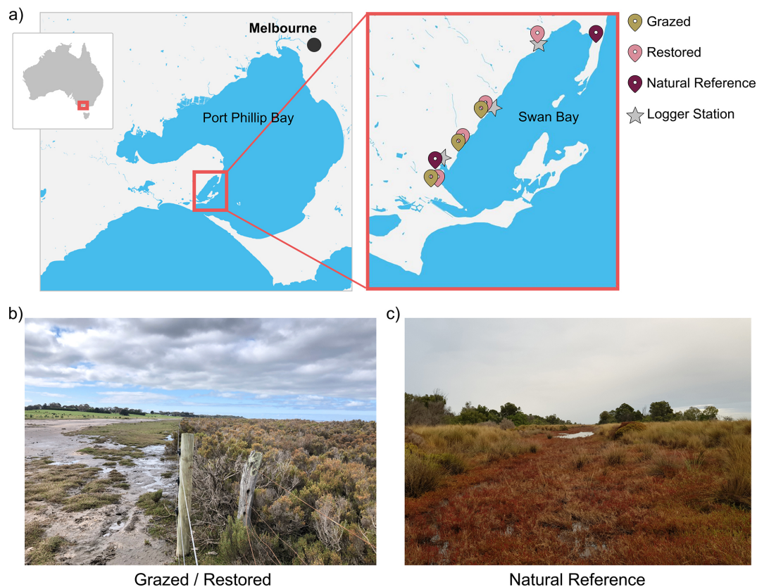
Figure 1. Site map. (a) Swan Bay is an embayment in Port Phillip Bay, Victoria, Australia. Points represent the site rehabilitation category and location of logger stations. (b) A site in Swan Bay, showing a currently grazed area on the left, and a > 25-year restored area on the right, following the installation of a fence by Parks Victoria in 1996 to restrict access and allow saltmarsh to return. (c) A natural reference site has had little to no modification in the last 50–60 years.
