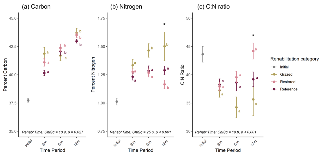
Figure 5. Elemental content of S. quinqueflora roots throughout 1-year of decomposition. (a) Percent organic carbon. (b) Percent nitrogen. (c) Molar Carbon : Nitrogen ratios. Letters indicate post-hoc differences over time for each rehabilitation category individually, not across categories for each time point. Asterisks indicate a significant difference at 12 months between Grazed sites and both Restored and Natural Reference sites. Data represent mean and standard error.
