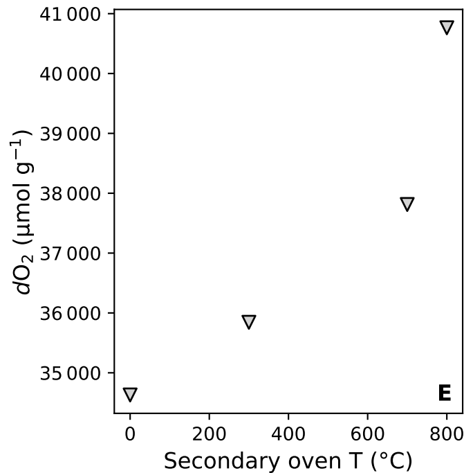
Congo Basin
