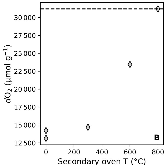
Congo Basin
