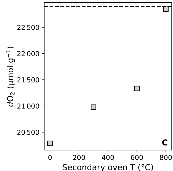
Pyrite
