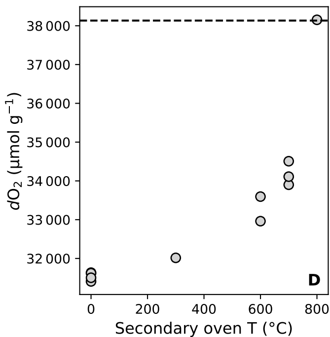
Natural samples: MSG9
