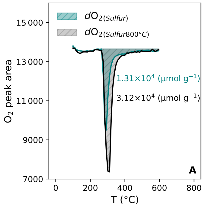
Standard samples: Sulfur
