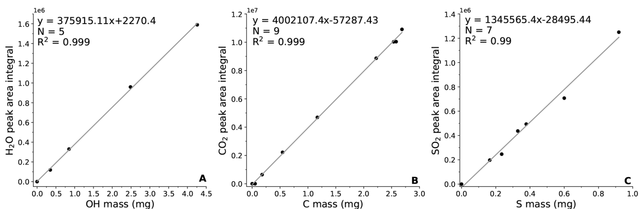
Figure 3. Gas concentration calibrations. (A), Hydrogen; (B), Carbon; (C), Sulfur. Note: The different mass ranges for H, C and S calibration due to our calibrations focus on the typical ranges of H, C, S concentrations in the natural samples. S is typically low, while H and C can reach much higher concentrations in rocks and sediments, so the calibration reflects this wider range (Table S2 in the Supplement). The different slopes are reflecting different behaviors of the elements and response of the sensor.
