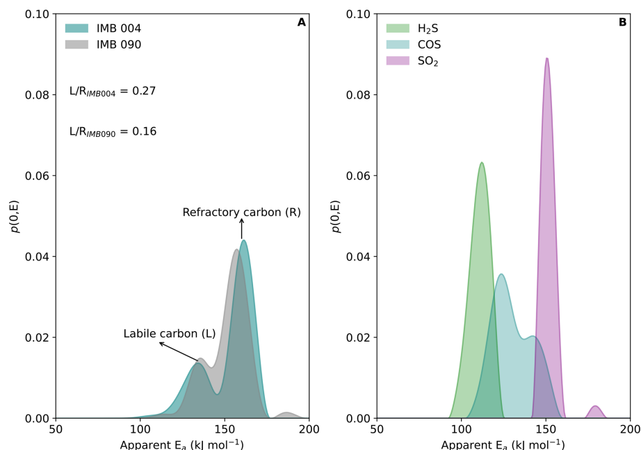
Figure 5. Kinetically-resolved carbon and sulfur speciation. (A) , aE_a distributions for carbon speciation in peat samples from the Congo Basin, including labile and refractory carbon fractions. (B) , aE_a distributions of sulfur speciation in a sample from Lake Cadagno, including \text{H}_2\text{S} , COS, and \text{SO}_2 .
