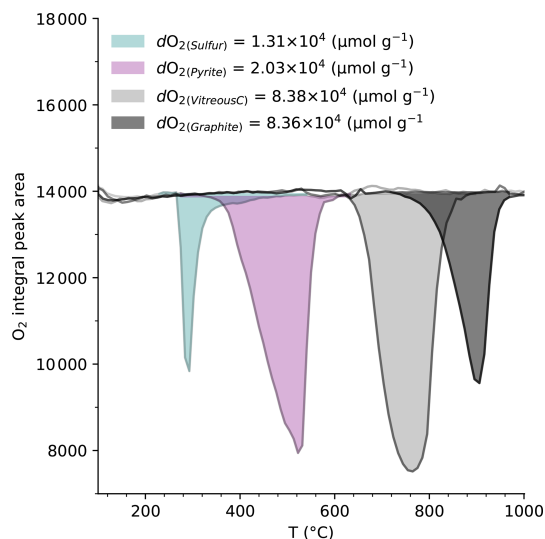
Figure 6. Oxygen consumption profiles of elemental sulfur, pyrite, vitreous carbon and graphite during controlled thermal oxidation. Replicate measurements for vitreous carbon and graphite yield high precision and reproductivity (Fig. S1).
