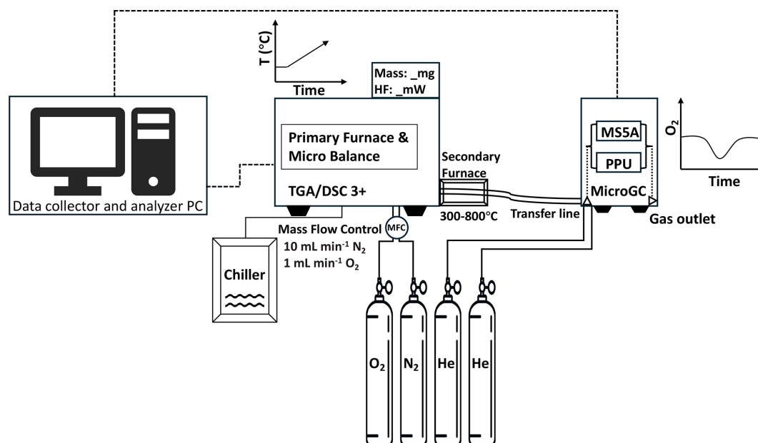
Figure 1. TGA/DSC-MicroGC instrument schematic.
