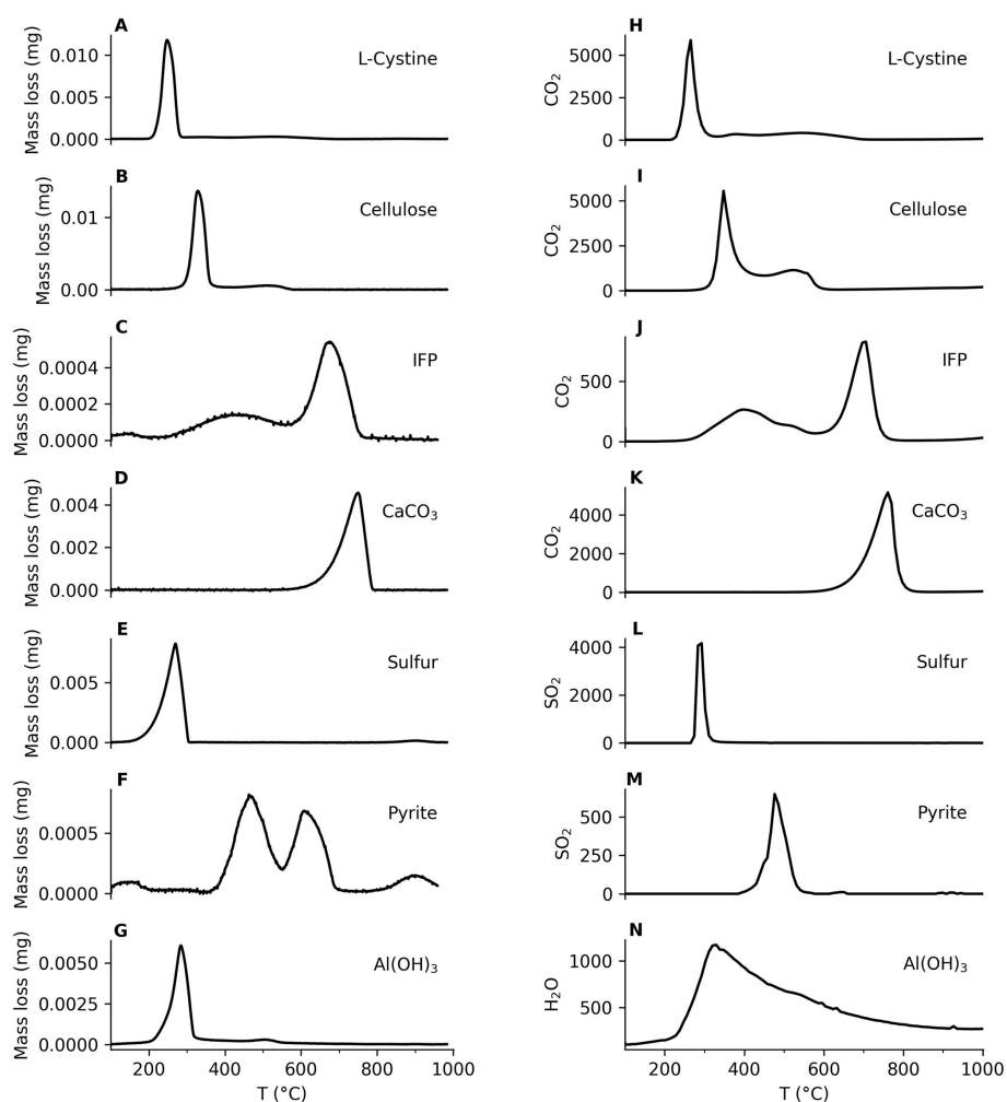
Figure 2. Mass loss and devolatilized components from standards evaluated by using TGA/DSC-MicroGC system. (A, H) L-Cystine; (B, I) Cellulose; (C, J) IFP; (D, K) \text{CaCO}_3 ; (E, L) Elemental sulfur; (F, M) Pyrite; (G, N) \text{Al}(\text{OH})_3 .
