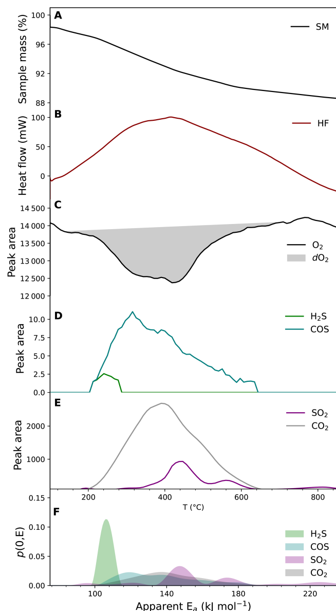
Figure 10. Kinetic fingerprint for a representative sulfidic sediment from Lake Cadagno. (A), Sample mass (SM) changes at heating rates of 10\text{ }^{\circ}\text{C min}^{-1} ; (B), Heat flow (HF) profile; (C), oxidation profile; (D), \text{H}_2\text{S} and COS profiles; (E), \text{SO}_2 and \text{CO}_2 profiles; (F), aE_a distribution of \text{H}_2\text{S} , COS, \text{SO}_2 and \text{CO}_2 .
