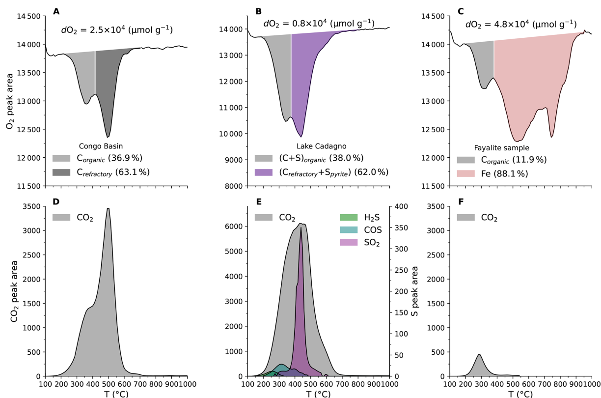
Figure 8. Oxidation profile with corresponding components. (A), Congo Basin peat sample; (B), Cadagno Lake sediment sample; (C), fayalite sample; (D–F), gases released through distinct reactions from samples (A), (B) and (C), respectively.
