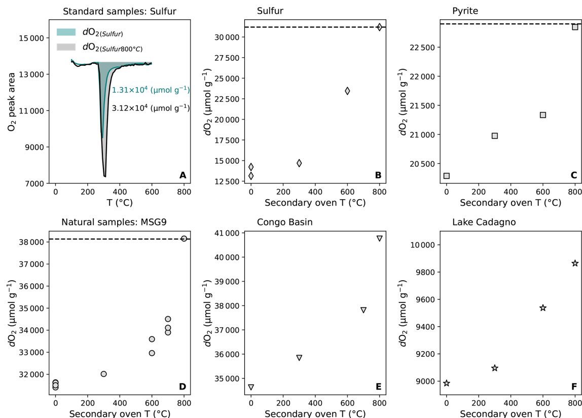
Figure 7. Optimized redox capacity with secondary oven. (A), Comparison of elemental sulfur measurements with secondary oven (at 800 ^{\circ}\text{C} , grey) and without secondary oven (teal); (B), elemental sulfur; (C), pyrite; (D), black shale (MSG9); (E), peat sediment from the Congo basin; (F), Lake Cadagno sediment. Black dashed lines in (B), (C) and (D) panels indicate the theoretical values.
