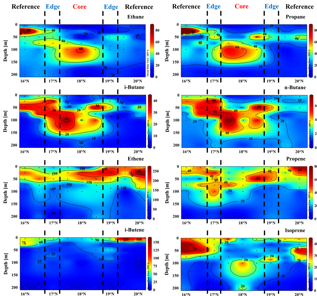
Figure 3. Vertical profiles of NMHCs ( \text{pmol L}^{-1} ) along transect C in the northern SCS. Figure credits: Schlitzer, Reiner, Ocean Data View, https://odv.awi.de/ (last access: 19 May 2026), 2026.
