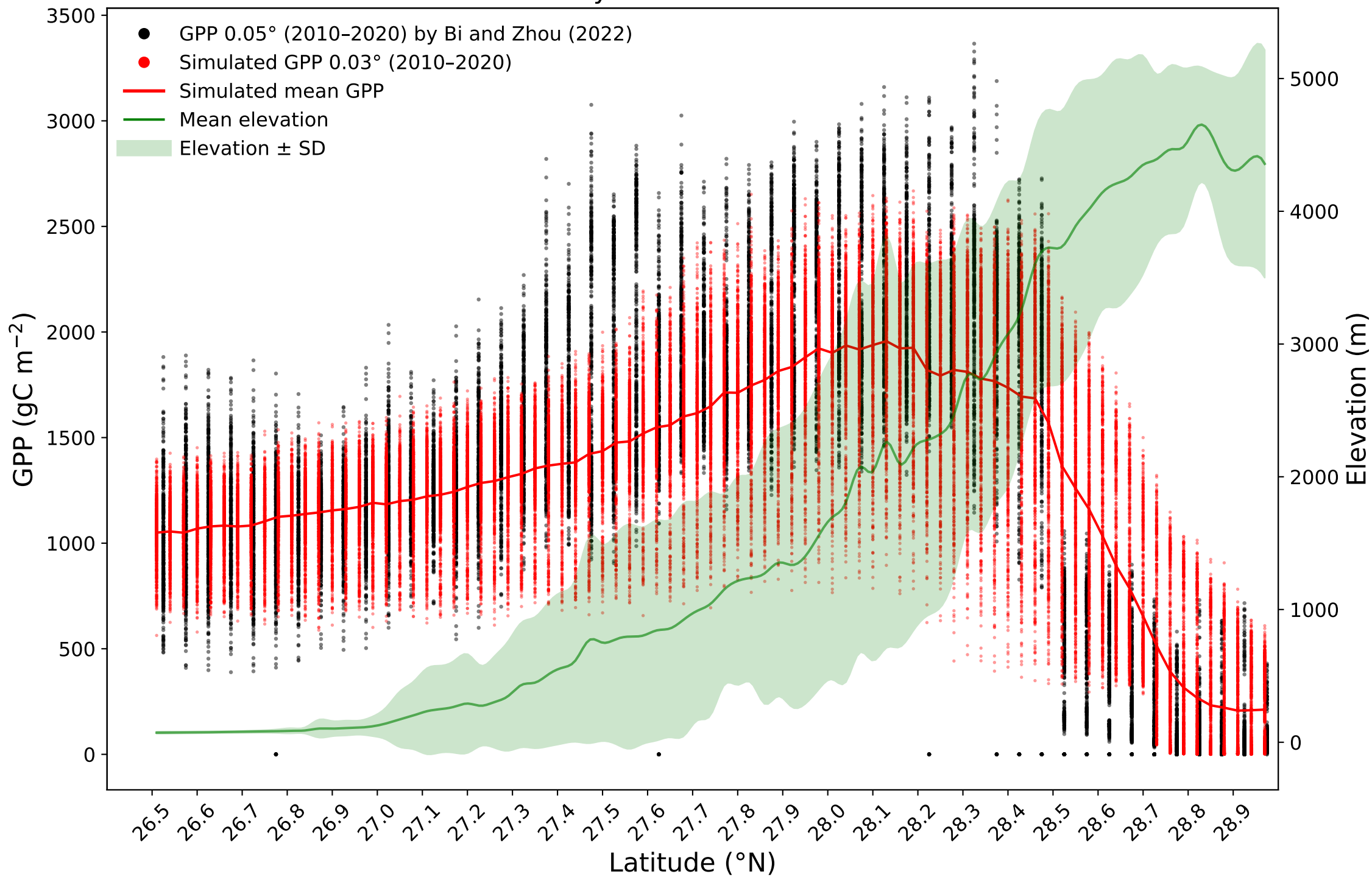
Yearly GPP and elevation
