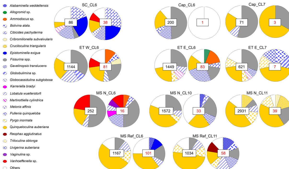
Figure 5. Relative abundance (pie charts) and absolute number of individuals of the main benthic foraminiferal species (e.g., representing > 5% of the total abundance) with dead communities represented on the left (black numbers) and living communities on the right (red numbers). Note that all Rotalida species are in blue and all Miliolida species in yellow.
