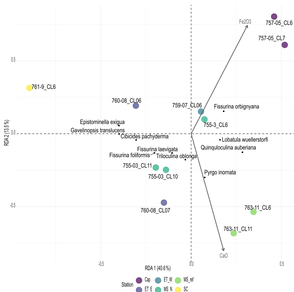
Figure 7. Redundancy Analysis of the main benthic foraminiferal species (> 5 % of the total abundance) of the Lucky Strike vent field based on dead communities and environmental parameters of the top sediment layers (0–1 cm).
