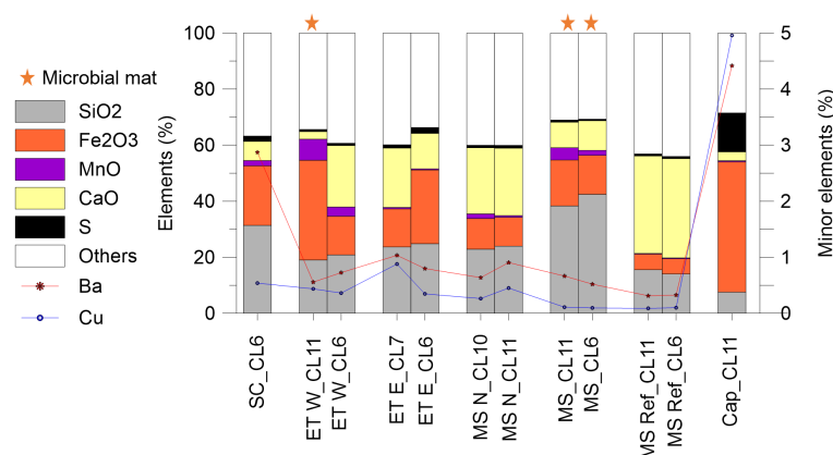
Figure 2. XRF analyses of top layers (0–1 cm) of the 12 sediment cores sampled in 2020 on the Lucky Strike vent field (Mid-Atlantic Ridge). Ba and Cu are plotted as minor elements (right scale).
