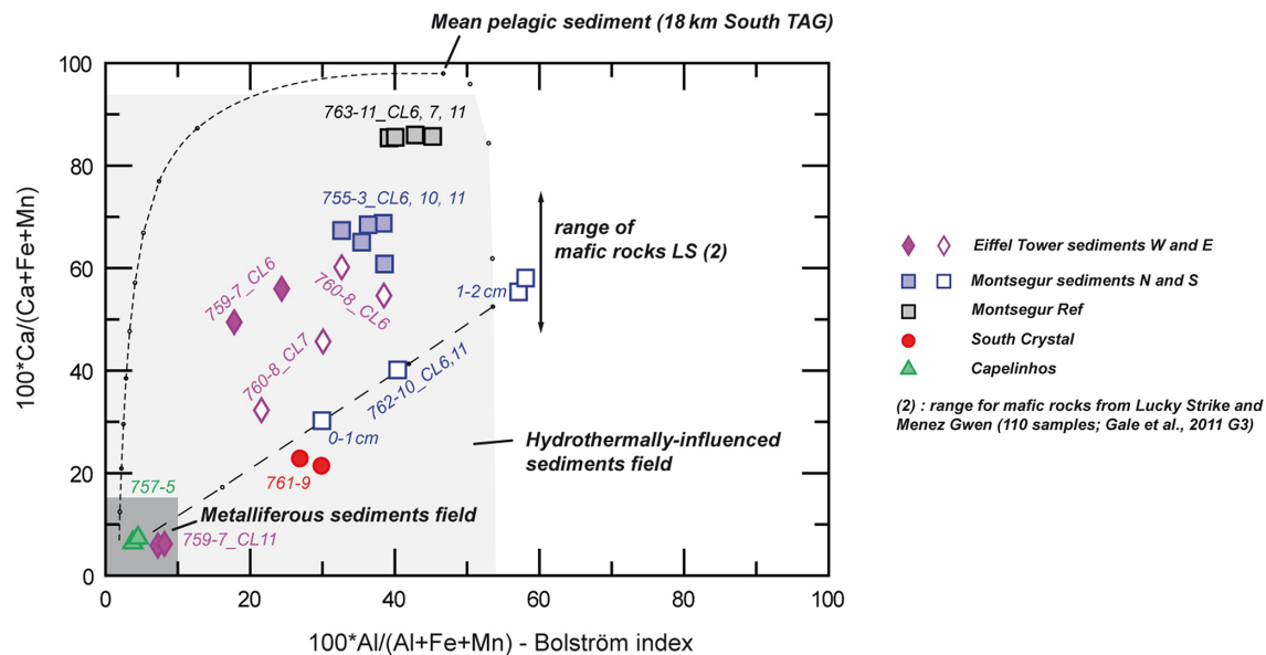
Figure 3. Bolström diagram representing the geochemical analyses of the top sediment layers (0–1 cm) in the peripheries of four active edifices on the Lucky Strike vent field (Mid-Atlantic Ridge), corresponding to cores analyzed for foraminiferal analyses.
