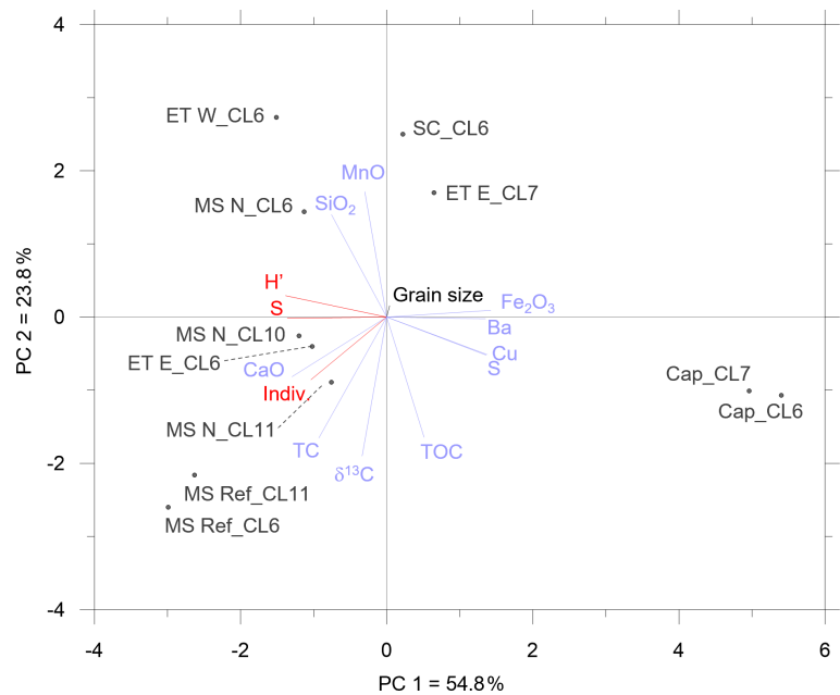
Figure 4. Principal Component Analysis with environmental parameters in blue and biological metrics in red. H' = shannon index, S = specific richness, Indiv. = number of individuals.
