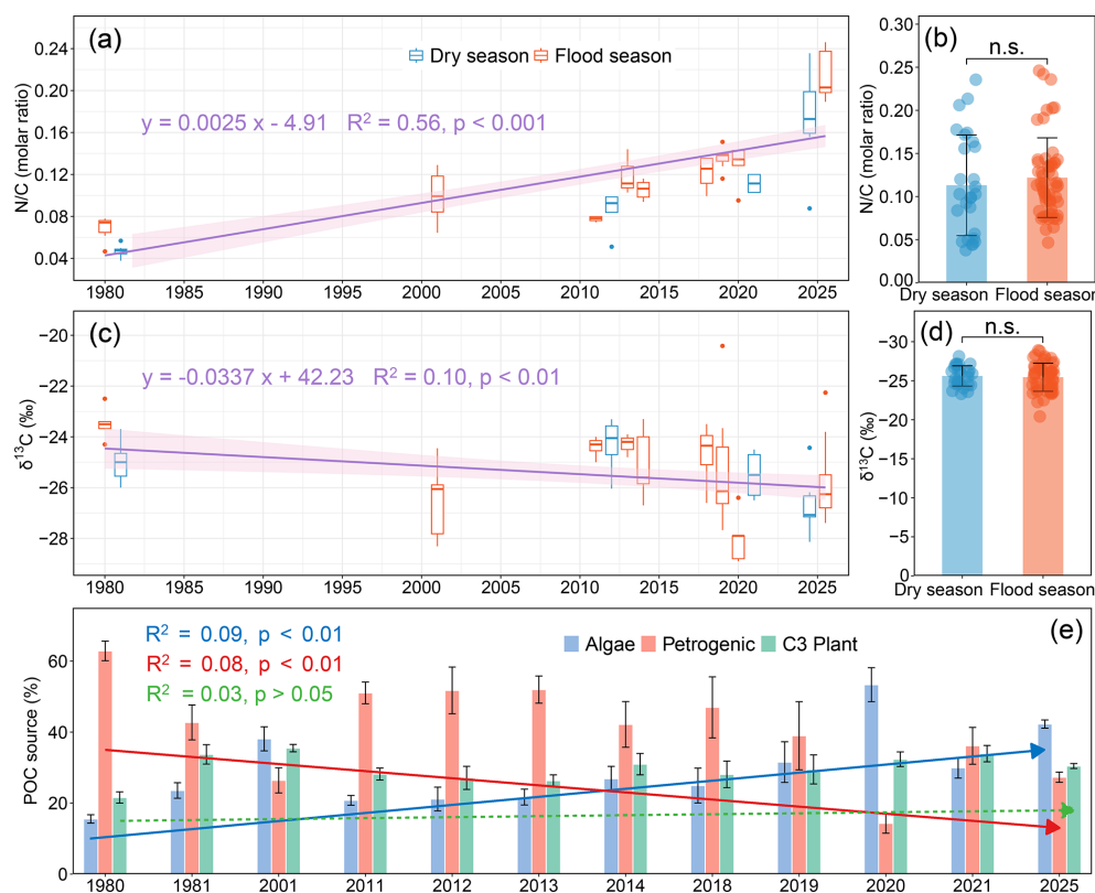
Figure 2. Temporal variations of N / C molar ratios (a) and \delta^{13}\text{C} values (c) in suspended particulate matter (SPM) collected in surface water in the Changjiang Estuary from 1980 to 2025. Differences of N / C molar ratios (b) and \delta^{13}\text{C} values (d) between dry and flood seasons. Temporal trends of proportions of particulate organic carbon (POC) derived from different terrestrial sources (freshwater algae, petrogenic and C3 plant sources) estimated through a Bayesian End-member Mixing approach from 1980 to 2025 (e). Solid lines represent significant ( p < 0.05 ) linear associations, and the light purple areas around the line indicate 95 % confidence interval. The n.s. indicates non-significant ( p > 0.05 ) differences.
