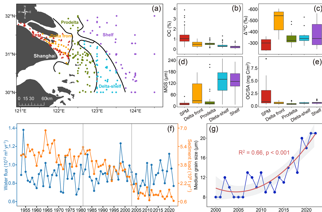
Figure 1. Sampling sites of suspended particulate matters (SPM) and surface sediment in Changjiang Estuary and its adjacent areas, including both field-collected samples and literature-compiled data (a). Differences in parameters between riverine SPM and deltaic sediments, including organic carbon (OC) contents (wt % of dry sediment) (b), \Delta^{14}\text{C} (c), medium grain size (MGS) (d) and ratios between OC contents and specific surface area (OC/SA) (e). Variations of annual mean water flux and sediment load of the Changjiang River from 1953 to 2022 (f). Changes of annual MGS of the sediment delivered by the Changjiang River from 2000 to 2022 (g). Four sedimentary facies (Delta front, Prodelta, Delta-shelf and Shelf) of the Changjiang subaqueous delta in panel (a) are classified according to Chen et al. (1991) and delineated by black lines. In panels (b–e), the horizontal line inside each box represents the median, and the lower and upper edges of the box indicate the first and third quartiles, respectively. The box height denotes the interquartile range (IQR), and the whiskers extend to the most extreme data points within 1.5 \times \text{IQR} of the lower and upper quartiles. The two gray vertical lines in panel (f) correspond to the construction of the Gezhouba Dam in 1981 and the Three Gorges Dam in 2003, respectively, on the mainstream of the Changjiang River. Data of riverine water flux, sediment load and MGS in Datong Gauge Station are applied to represent characteristics of water and sediment input into the East China Sea based on Zhao et al. (2021a) and the China River Sediment Bulletin for 2000–2022 (Ministry of Water Resources of the People's Republic of China, 2001–2023). The fitted line in panel (g) represents a quadratic fit, and the gray shaded area indicates the 95 % confidence interval.
