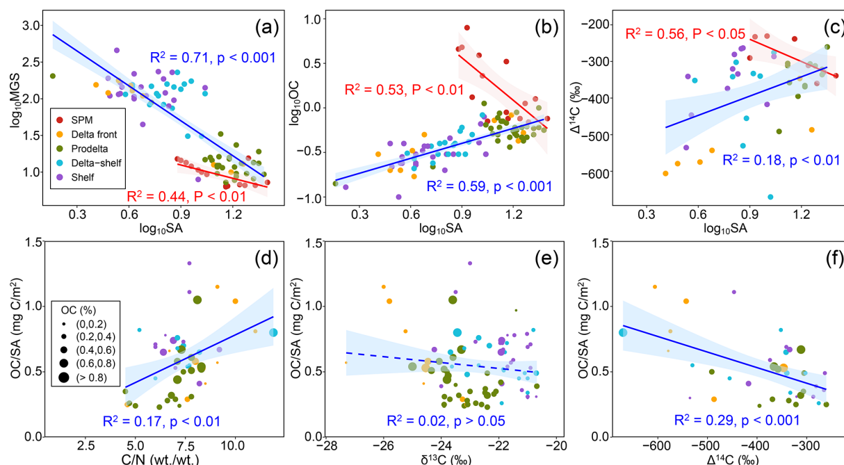
Figure 5. Relationships among medium grain size (MGS), specific surface area (SA), organic carbon (OC) properties, and SA-normalized OC loading (OC / SA) in suspended particulate matter (SPM) from the Changjiang Estuary and surface sediments from the Changjiang subaqueous delta. Relationships of SA with MGS (a), OC content (b) and \Delta^{14}\text{C} (c) in SPM and surface sediments. Relationships of OC / SA with C / N (d), \delta^{13}\text{C} (e), and \Delta^{14}\text{C} (f) in surface sediments. Solid and dashed lines indicate statistically significant ( p < 0.05 ) and non-significant ( p > 0.05 ) relationships, respectively. Shaded areas represent 95 % confidence intervals.
