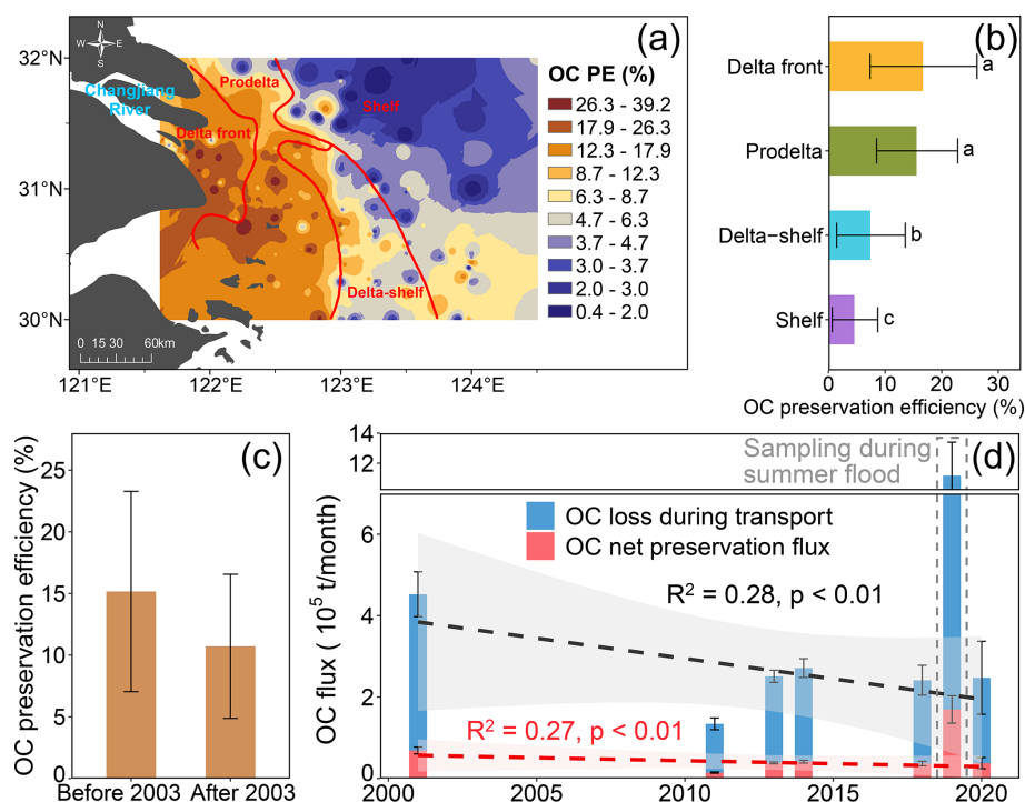
Figure 4. Spatial pattern of organic carbon (OC) preservation efficiency in the Changjiang subaqueous delta (a), and OC preservation efficiency in different sedimentary facies (b). Changes in OC preservation efficiency in the Changjiang subaqueous delta before and after 2003 (c). Temporal trends in the amount of OC preserved in deltaic sediments (red dashed line) and riverine OC flux (black dashed line) from 2001 to 2020, and the blue bars reflect OC loss (difference between amount of OC preservation and riverine OC flux) during sediment transport (d). The PE indicates preservation efficiency in panel (a). Different lowercase letters in panel (b) denote statistically significant differences ( p < 0.05 ) among sedimentary facies. In panel (d), the high value in 2019 (gray dashed circles) primarily induced by extreme summer flood (Sun et al., 2021) was excluded from trend analysis. The dashed lines indicate linear relationships, and the light gray and red areas around the line represent 95 % confidence interval.
