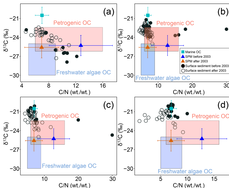
Figure 3. Relationships between \delta^{13}\text{C} and C / N in surface sediments in the Delta front (a), Prodelta (b), Delta-shelf (c) and Shelf (d) before and after 2003. Light red and blue areas represent ranges of \delta^{13}\text{C} and C / N corresponding to terrestrial organic carbon (OC) derived from petrogenic and freshwater algae sources, respectively, in terms of Lamb et al. (2006) and Menges et al. (2020). The marine OC end-member of \delta^{13}\text{C} is from -19.2\text{‰} to -21.8\text{‰} and of C / N is 6–8 (Xing et al., 2011; Bao et al., 2018).
