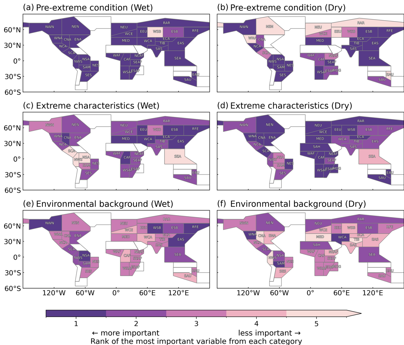
Figure 3. Relevance of pre-extreme vegetation condition, extreme characteristics and environmental background for negative vegetation responses to (a, c, e) wet and (b, d, f) dry events. Relevance is expressed as the rank of the most important variable for explaining vegetation greenness anomalies during extremes from each category. The top variables are ranked across categories. Note that each category contains a different number of variables and the attribution is based only on extremes with negative NDVI anomalies (see Table S1 and Sect. 2.3).
