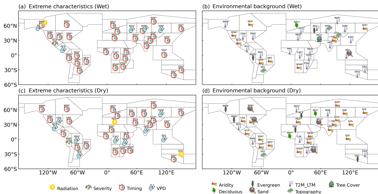
Figure 4. Most relevant variables for negative vegetation responses during wet (a, b) and dry (c, d) extremes in terms of extreme characteristics and environmental background. Multiple variables are shown in case their relevance is the same according to the ranking. The asterisk next to each region label indicates that the most relevant variable was selected at least 50 % more frequently than the second most relevant variable within that category. Note that the attribution analysis is based only on extremes with negative NDVI anomalies.
