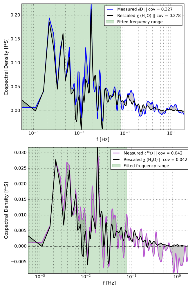
Figure A2. Example co-spectral analysis, and implementation of the spectral correction method described in Moonen et al. (2023), of the 30 min interval starting at 14:00 on 12 August 2022. Note that the covariance of both species with the vertical wind ( w ) is shown. The green window indicates the time scales which were used to rescale \chi(\text{H}_2\text{O}) . The contributions to the \delta^{18}\text{O} flux around 10^0 have a negative sign, which we believe must be a measurement artifact.
