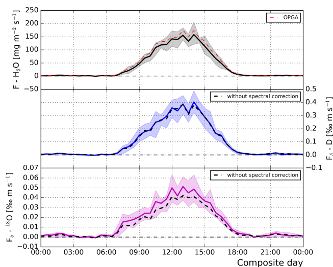
Figure 2. (top) Composite day 30 min average water flux derived using the closed path isotope analyser and an Open Path Gas Analyser (OPGA, shown in red). (middle and bottom) Composite day 30 min average D and ^{18}\text{O} \delta fluxes derived using the water isotope analyser combined with the EC method. The dashed black lines show the data before correction of signal loss at high frequencies. The shaded areas indicate the 25 to 75 % quantiles of the 13 d contributing to the composite day.
