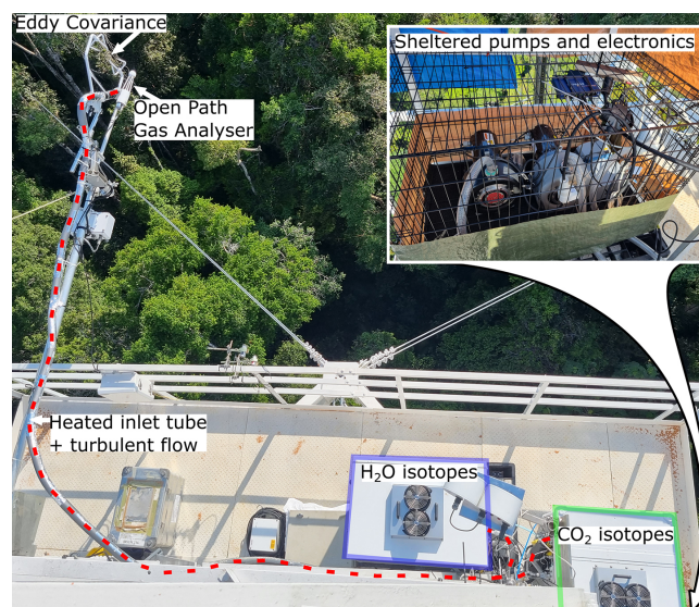
Figure 1. Picture of the isotopologue flux setup which was installed on the 54 m balcony of the ATTO tower in Central Amazonia, Brasil. The schematic overlay highlights the key components of the setup. The picture was taken by Oscar Hartogensis (oscar.hartogensis@wur.nl).
