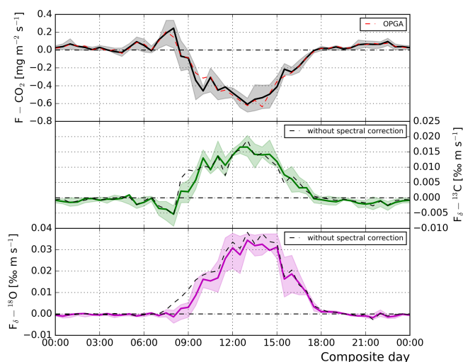
Figure 4. (top) Composite day 30 min average \text{CO}_2 fluxes derived using the closed path isotope analyser and an Open Path Gas Analyser (OPGA, shown in red). (middle) and (bottom) Composite day 30 min average ^{13}\text{C} and ^{18}\text{O} \delta fluxes derived using the \text{CO}_2 isotope analyser combined with the EC method. The dashed black lines show the data before correction of signal loss at high frequencies. The shaded areas indicate the 25 % to 75 % quantiles of the 13 d contributing to the composite day.
