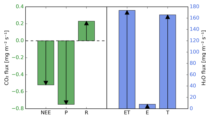
Figure 7. Results of the partitioning of the net ecosystem exchange fluxes NEE and ET based on the 13 d composite 14:00 isotopic state, following Eq. (2). For NEE, the ^{18}\text{O}\text{-CO}_2 isotope was used following the approach described in Sect. 2.3. For ET, the average of the partitioning results derived from \delta\text{D} and \delta^{18}\text{O} is shown (see Sect. 2.2).
