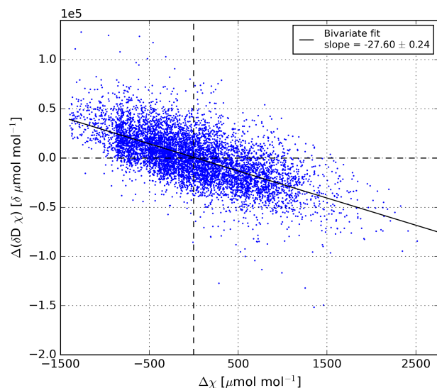
Figure A1. Example Miller-Tans analysis of the 30 min interval starting at 15:00 on 15 August 2022. The variations in \delta values and \text{H}_2\text{O} mole fractions ( \chi ) were measured using the \text{H}_2\text{O} isotope analyser measuring from the inlet at 57 m. The \Delta refers to the difference between the measured value and the atmospheric background (Miller and Tans, 2003).
