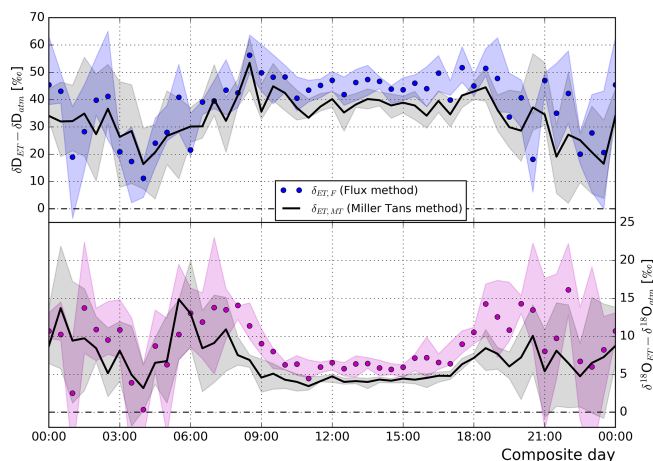
Figure 3. Composite day representation of 30 min average isotopic compositions of the net flux ( \delta_{\text{ET}} ) derived using measurements performed with the water isotope analyser. The flux method composition ( \delta_{\text{ET},\text{F}} ) was derived using Eq. (4). Both the Miller-Tans and flux methods are described in Sect. 2.1. The shaded areas indicate the 25 % to 75 % quantiles of the 13 d contributing to the composite day.
