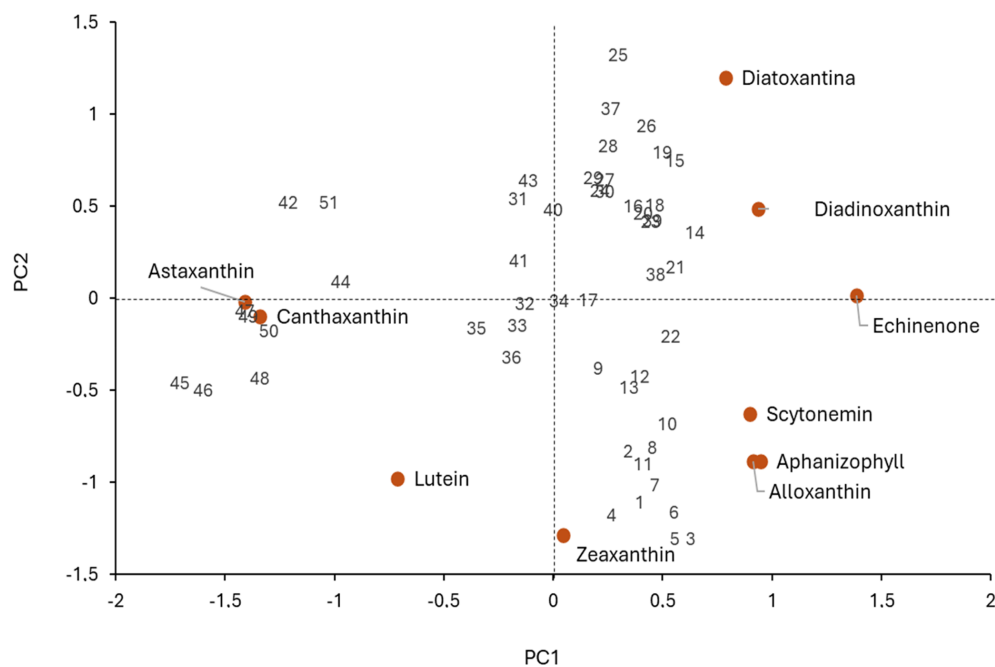
Figure 5. Principal component analysis (PCA) biplots of the pigment assemblages from sediment core SSBG-21 extracted from Borreguil Lake for the last ~ 430 years. Numbers refer to the sample sites being 1 the most modern sample and 51 the oldest sample.
