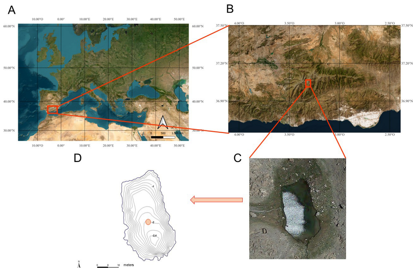
Figure 1. (A) Location of Borreguil Lake, Sierra Nevada, Spain. (A) Location of Sierra Nevada in southern Spain; (B) Location of Borreguil Lake in the range; (C) Borreguil Lake; (D) Bathymetric map of the lake (extracted from digitized map of bathymetry report from Egmasa S.A.). The orange dot indicates the point at which the sediment core was retrieved. Imagery ©Landsat/Copernicus, Map data © 2025 Google.
