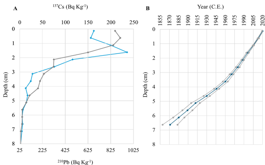
Figure 2. (A) Radiometric chronology showing 210 Pb (grey line) and 137 Cs (blue line) activity (Bq kg -1 dried sediment) from sediment core SSBG-21 extracted from Borreguil Lake. (B) 210 Pb-estimated age (using the constant rate of supply model) versus core depth (black line) and the associated errors (grey lines).
