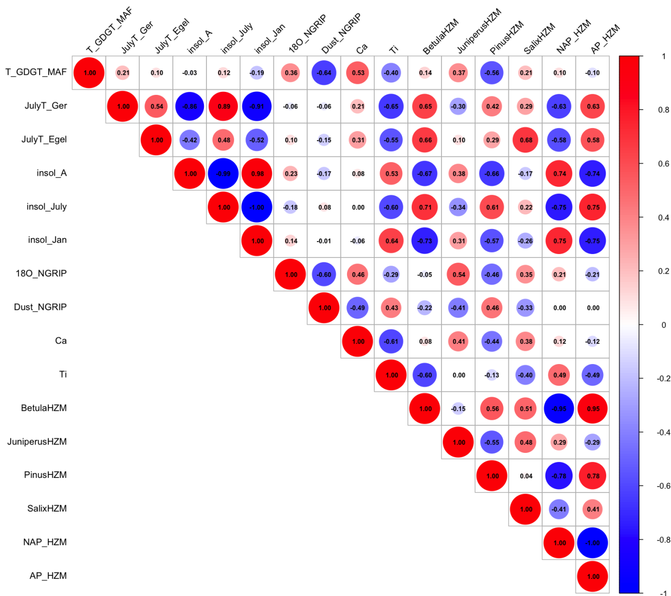
Figure B1. Correlation matrix of environmental variables used in RDA analysis. Pearson correlation coefficients between the 16 environmental predictor variables ( T\_GDGT\_MAF =GDGT temperature of months above freezing, JulyT_Ger/Egel=July temperatures from Gerzensee and Egelsee, insol A /July/Jan=annual/seasonal insolation, 18O_NGRIP/Dust_NGRIP=stable isotope and dust proxy from NGRIP ice core, Ca/Ti=geochemical elements from XRF analysis, pollen percentages=BetulaH2M, JuniperusH2M, PinusH2M, SalixH2M, NAP_H2M, AP_H2M). Circle size and color intensity indicate correlation strength, with red indicating positive correlations and blue indicating negative correlations. Absolute correlation values are displayed for all variable pairs. This matrix demonstrates substantial inter-relationships among climatic predictors, particularly between temperature metrics and orbital insolation variables, which justified the application of a VIF < 10 threshold to balance multicollinearity control while retaining ecologically meaningful temperature signals for the constrained ordination analysis.
