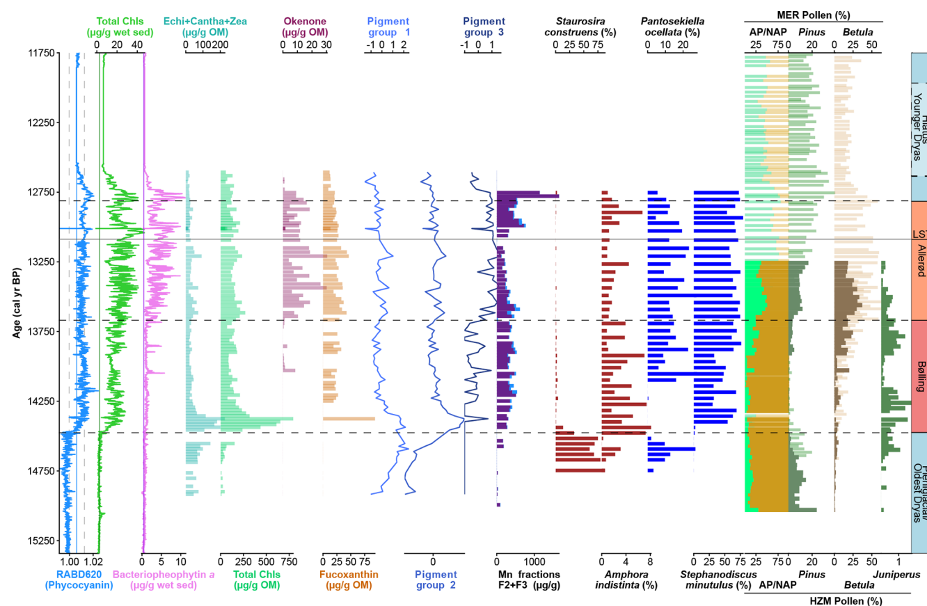
Figure 4. Stratigraphic variation of hyperspectral imaging data, selected sedimentary pigments, pigment communities derived from correlation (see Fig. 3), selected redox fractions (Mn), selected diatom species and pollen in Holzmaar (and Meerfelder Maar) (Litt and Stebich, 1999; Litt et al., 2009; Litt and Stebich, 2001; Litt, 2019, 2010). Downcore profiles of relative abundance of phycocyanin as RABD620, with solid line representing the mean value and dashed lines \pm 1\sigma , calibrated hyperspectral imaging bulk pigments data (expressed as \mu\text{g g}^{-1} of wet sediment) with the limit of quantification as a solid vertical line, and HPLC-analysed pigment concentrations (expressed as \mu\text{g g}^{-1} of OM) are plotted against age (cal yr BP). The pigment communities are plotted as z-scores. Benthic diatoms are plotted in dark red and planktonic diatoms are displayed in blue. Arboreal pollen is shown in light green and non-arboreal pollen in orange (Litt and Stebich, 1999; Litt et al., 2009; Litt and Stebich, 2001; Litt, 2019, 2001). Finally, Holzmaar pollen is in solid colour, whereas Meerfelder Maar pollen is underlying the Holzmaar pollen and is transparent. The horizontal gray bar marks the stratigraphic position of the Laacher See Tephra (LST) and the stratigraphy is following Lang et al. (2023); Litt and Stebich (1999) with the exact age boundaries following Birlo et al. (2023).
