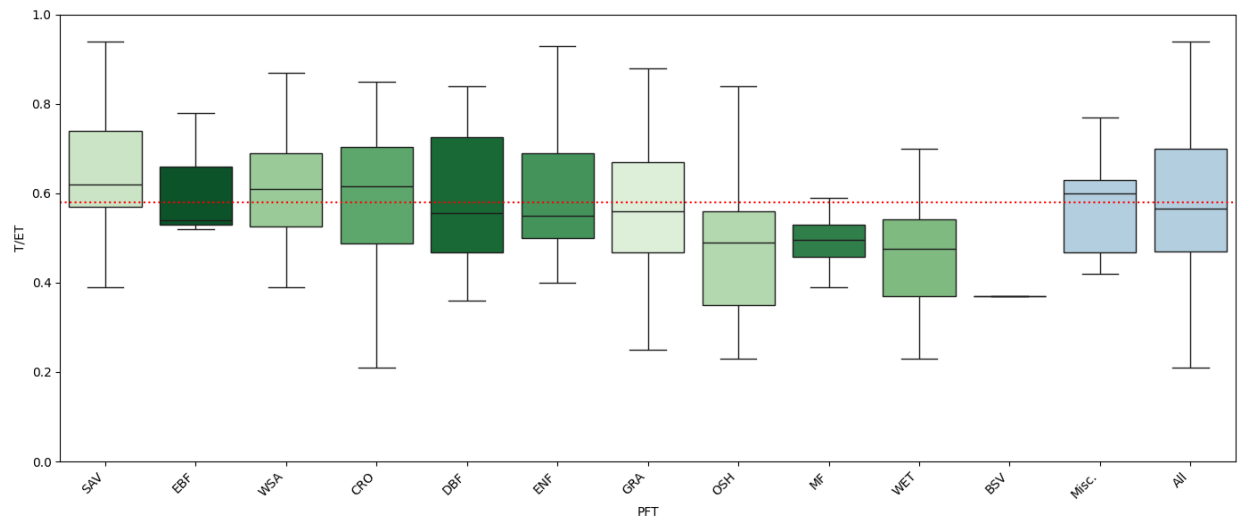
Figure S1: Box and whisker plots of ET partitioning estimates across plant functional types (PFT) created using all quantitative data extracted from the literature search. PFTs are shaded according to the estimated typical ecosystem LAI with the darker greens representing higher LAI. Misc. represents studies who reported data from combined ecosystem types, while All represents all data found from the literature search. The red dotted line ( T/ET = 0.57 ) represents the mean reported from global studies across methods. SAV: savanna, EBF: evergreen broadleaf forest, WSA: woody savanna, CRO: cropland, DBF: deciduous broadleaf forest, ENF: evergreen needleleaf forest, GRA: grassland, MF: mixed forest, OSH: open shrubland, WET: wetland, BSV: bare sparse vegetation.
