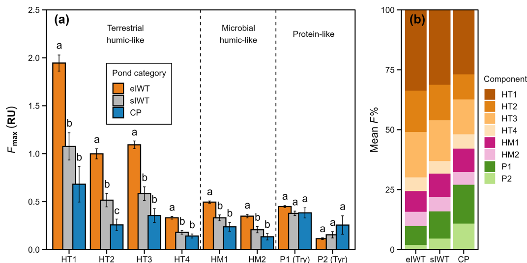
Figure 2. Absolute (a; mean \pm SE, n = 5 ) and relative (b; mean) fluorescence intensity for the components identified by PARAFAC analysis at the beginning of the bioassay for each pond category. The components are divided to terrestrial humic-like (HT1–HT4), microbial humic-like (HM1 and HM2), and protein-like (tryptophan-like component P1 = Try, and tyrosine-like component P2 = Tyr) according to their fluorescence characteristics. For each component, different letters in panel (a) represent significant differences between pond categories as determined by Tukey HSD tests ( P < 0.05 ).
