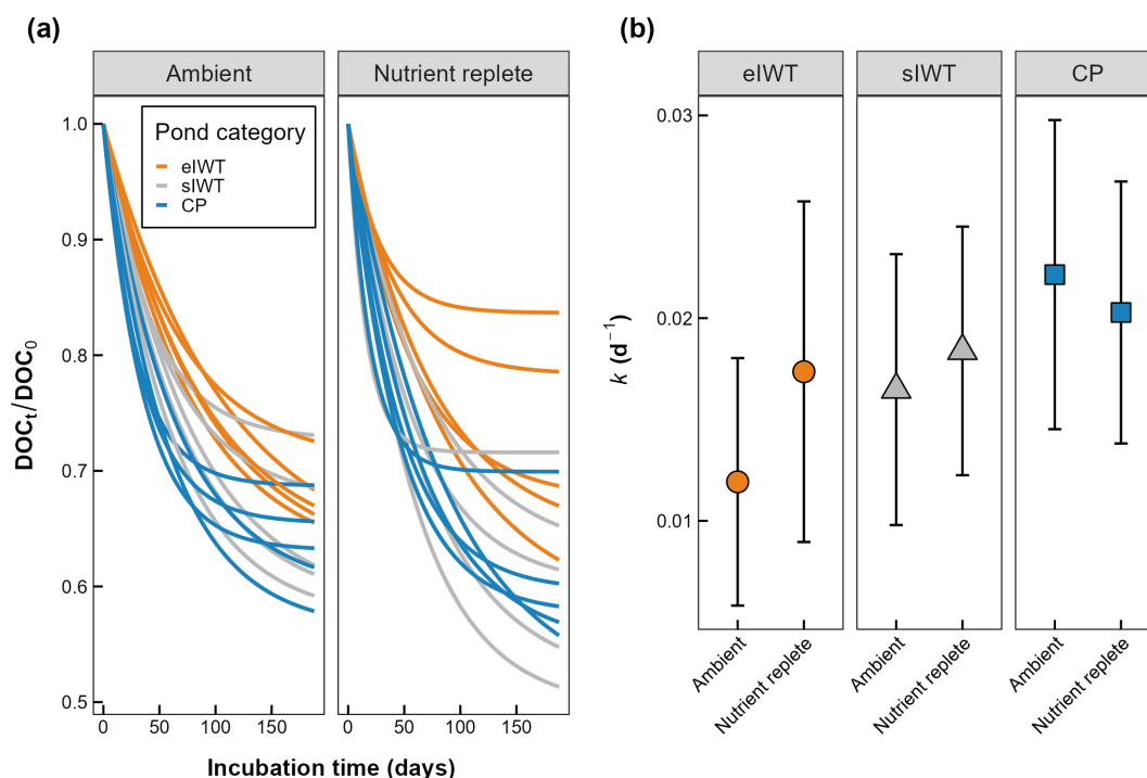
Figure 4. (a) Exponential decay model with residual DOC pool fitted to the time series of relative DOC decomposition during the 188 d dark bioassay using 2.7 \mu\text{m} -filtered pond water incubated at 15 ^{\circ}\text{C} , and (b) estimated decay coefficients and their 95 % confidence intervals among the three pond categories ( n = 5 ). The samples were incubated at ambient nutrient concentrations or amended with inorganic nitrogen and phosphorus (nutrient replete).
