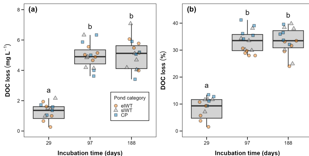
Figure 3. DOC loss during the 188 d dark bioassay using 2.7 \mu\text{m} -filtered pond water incubated at 15^\circ\text{C} at ambient nutrient concentrations ( n = 15 ). Results are expressed as DOC loss (a) and percentage DOC loss relative to initial DOC concentration (b). Boxplots indicate median (line), 1st and 3rd quartile (box margins), and 5 % and 95 % percentiles (whiskers). Different letters represent significant differences as determined by pairwise t -tests with Bonferroni correction ( P < 0.0001 ).
