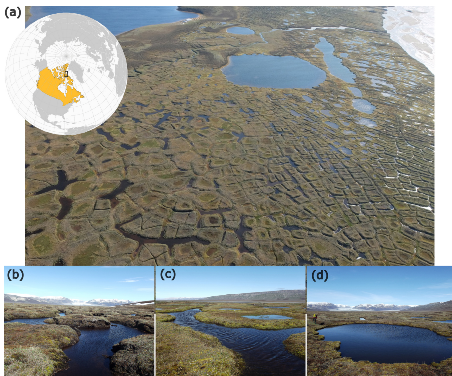
Figure 1. (a) Location of the study area and aerial view of the valley featuring an ice-wedge polygon complex (Isabelle Laurion). (b–d) Photographs of representative ponds: (b) an erosive ice-wedge trough pond, (c) a stable ice-wedge trough pond, and (d) a coalescent polygon pond (Thomas Pacoureau).
