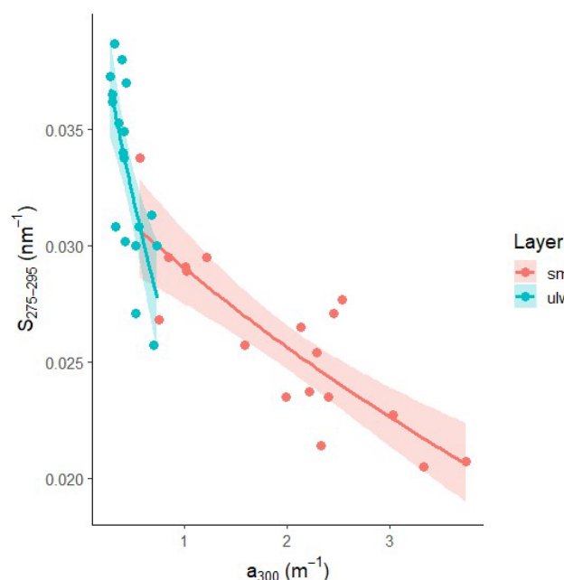
Figure 4. Predicted relationships between spectral slope ( S_{275-295} ) and absorption coefficient at 300 nm ( a_{300} ) based on the selected Gamma generalized linear model with log link. Points represent observed values, solid lines represent model predictions, and shaded areas indicate 95 % confidence intervals. Predictions are shown only within the observed range of a_{300} values for each layer.
