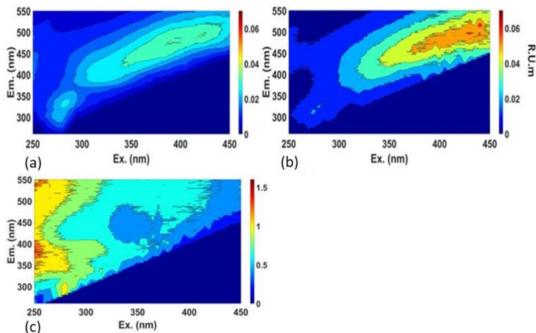
Figure 8. The FDOM/CDOM index (R.U. m) in the (a) SML, (b) ULW, (c) the ratio (\text{FDOM/CDOM})_{\text{sml}} / (\text{FDOM/CDOM})_{\text{ulw}} . (a, b) Depletion of the fluorescence intensity excited in the UV-A/near-visible range is apparent in the SML relative to the ULW. (c) Higher contribution of FDOM excited at short wavelength (UV-C/UV-B) to CDOM is apparent in the SML.
