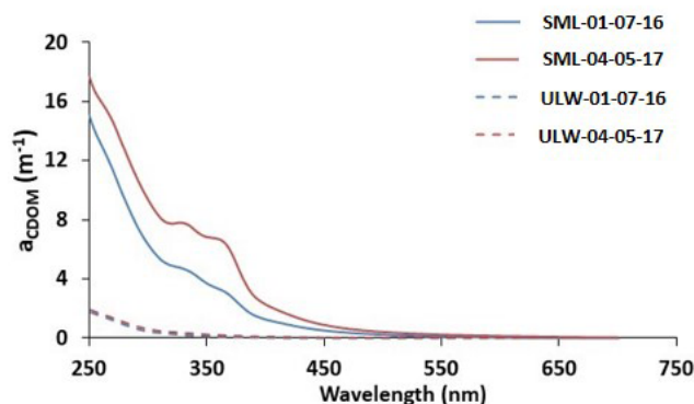
Figure 5. CDOM absorption spectra in the SML (solid lines) and ULW (dashed lines) on 1 July 2016 (blue) and 4 May 2017 (red). Spectral bands with maxima at 330, 360 nm are indicative of MAA absorption.
