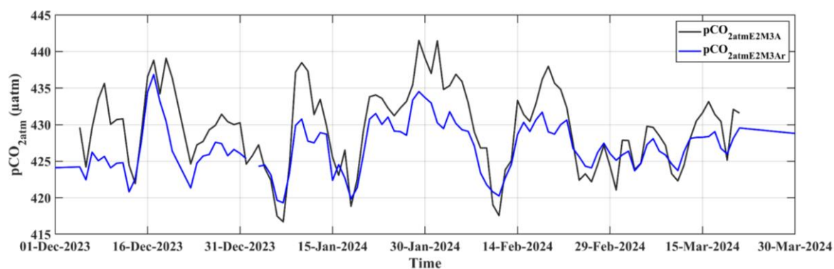
Figure S1. Time series of daily p\text{CO}_{2\text{atm}} measured at the EMSO-E2M3A ( p\text{CO}_{2\text{atmE2M3A}} , \mu\text{atm} ) in black and the p\text{CO}_{2\text{atm}} calculated from x\text{CO}_2 from Lampedusa ( p\text{CO}_{2\text{atmE2M3Ar}} , \mu\text{atm} ) in blue between December 2023 and March 2024. p\text{CO}_{2\text{atmE2M3Ar}} has been calculated according to Eqs. (1) and (2).
