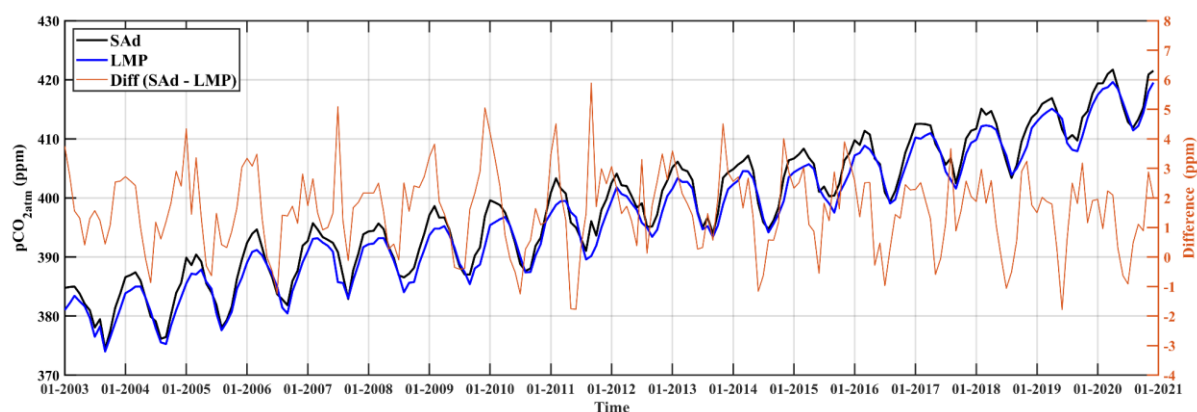
Figure S3. Monthly time series of p\text{CO}_{2\text{atm}} (ppm) at EMSO-E2M3A (SAd) and at Lampedusa (LMP) in black and blue respectively from the CAMS reanalysis of the European Centre for Medium-Range Weather Forecasts (ECMWF). The difference between the values in the two sites (SAd - LMP) is represented by the orange line.
