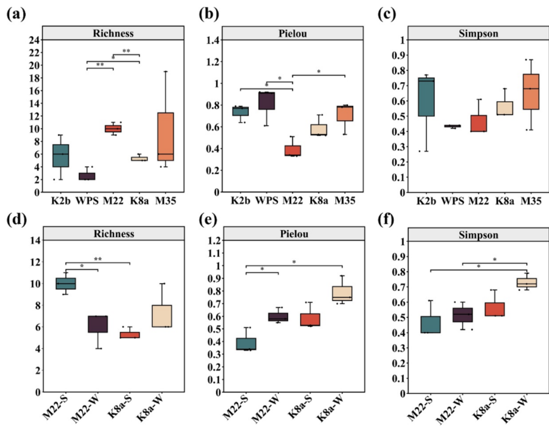
Figure 4. Alpha diversity index of the diatom community. (a, d) Richness index; (b, e) Pielou evenness index; (c, f) Simpson index. (a–c) Alpha diversity indices during the summer season. (d–f) Comparison of alpha diversity indices between summer and winter. “M22-S”, “M22-W”, “K8a-S”, and “K8a-W” represent M22-summer, M22-winter, K8a-summer, and K8a-winter, respectively. The boxes indicate the ranges of the first and third quartiles, the line inside each box represents the median, and the whiskers show the lowest and highest data points (mean ± 1.5 SD). Note that Simpson’s index is presented as 1-D. Asterisks indicate statistically significant results (* p < 0.05 ; ** p < 0.01 ).
