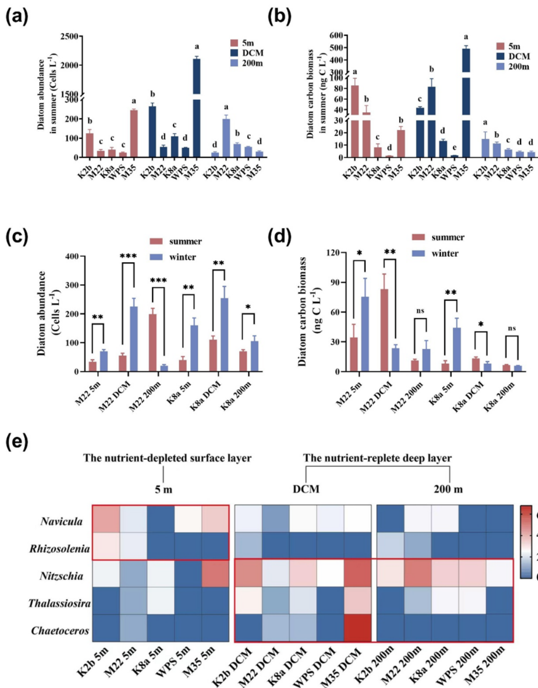
Figure 3. The regional heterogeneity of diatom abundance, estimated carbon biomass, and dominated species in the western North Pacific Subtropical Gyre (NPSG). (a) Abundance of diatoms at three depths across five stations in summer. The significance marked in the legend represents the within-layer comparison. (b) Estimated carbon biomass of diatoms at three depths across five stations in summer. The significance marked in the legend represents the within-layer comparison. (c) Comparison of diatom abundance between summer and winter. (d) Comparison of diatom carbon biomass estimates between summer and winter. (e) Heat map depicting the relative abundance of dominant diatoms in the water column. KE: Kuroshio Extension area; NEC: North Equatorial Current. The DCM layer depths in summer for stations K2b, WPS, M22, K8a, and M35 are 110, 145, 155, 150, and 95 m, respectively. In winter, the DCM layer depths for stations M22 and K8a are 135 and 146 m, respectively.
