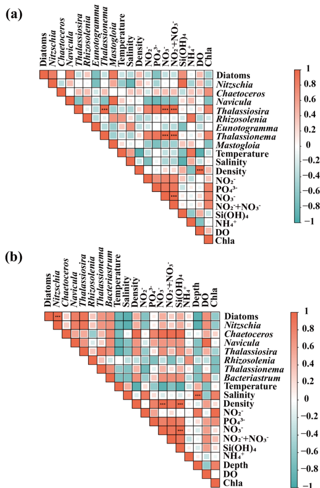
Figure 5. Spearman's correlation between diatoms and environmental factors in summer. (a) Surface seawater layer (b) Deep chlorophyll maximum (DCM) layer. \text{NO}_2^- : nitrite, \text{PO}_4^{3-} : phosphate, \text{NO}_3^- : nitrate, \text{Si(OH)}_4 : silicic acid, \text{NH}_4^+ : ammonium, DO: dissolved oxygen, Chl a : chlorophyll a . Asterisks denote significant correlations after Benjamini-Hochberg correction (***, p < 0.001 ).
