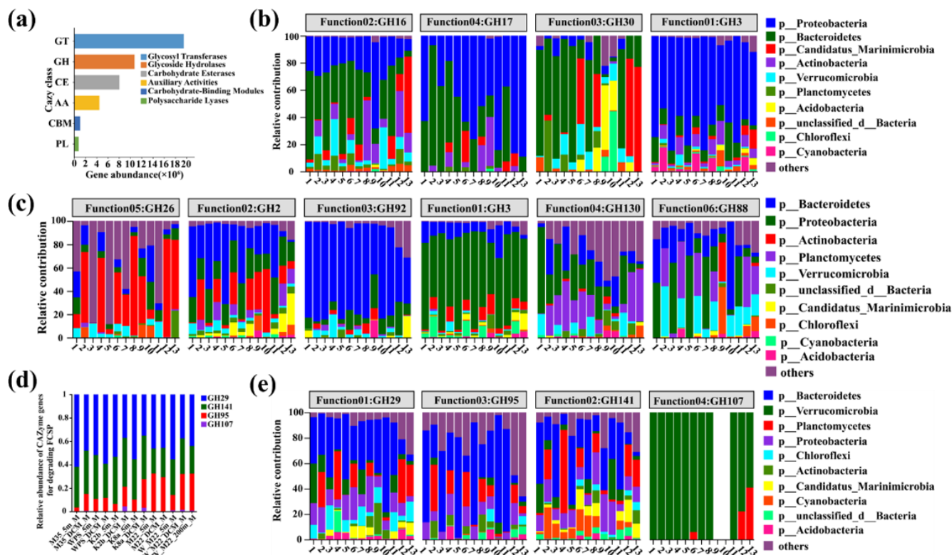
Figure 7. Composition and abundance of CAZyme genes, along with the contribution of dominant microbial groups at the phylum level. (a) CAZyme gene composition and abundance detected in this study. (b) Contribution of dominant microbial groups to CAZymes for degrading laminarin. (c) Contribution of dominant microbial groups to CAZymes for degrading mannans. (d) Composition and relative abundance of CAZyme genes for degrading fucose-containing sulfated polysaccharides (FCSP). (e) Contribution of dominant microbial groups to CAZymes for degrading FCSP. “M35_5m_M” and “M35_DCM_M” denote water samples collected at depths of 5 m and the depth of maximum chlorophyll a (DCM), respectively, from station M35 during the summer cruise for metagenomic analysis. This naming convention is consistently applied to samples from four additional stations (WPS, K2b, M22, and K8a). “W_M22_5m_M”, “W_M22_DCM_M”, and “W_M22_200m_M” refer to water samples collected at depths of 5 m, DCM, and 200 m, respectively, from station M22 during the winter cruise for metagenomic analysis. Samples “1” to “10” represent summer collections at M35_5m, M35_DCM, WPS_5m, WPS_DCM, K2b_5m, K2b_DCM, K8a_5m, K8a_DCM, M22_5m, and M22_DCM, while “11”, “12”, and “13” represent winter collections at M22_5m, M22_DCM, and M22_200m, respectively. Taxa with a relative abundance below 0.01 in all samples were aggregated into the category “others”.
