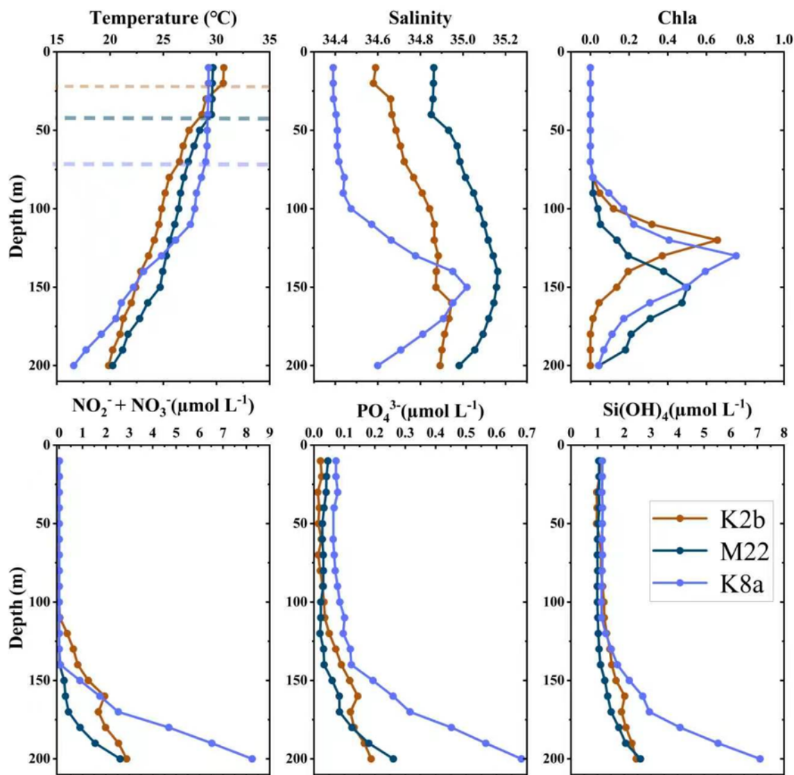
Figure 2. Vertical profiles of temperature, salinity, nutrients, and chlorophyll a within the 0–200 m layer during summer season. In the temperature graph, the dotted lines indicate the approximate positions of the bottom of the surface mixed layer at different stations.
