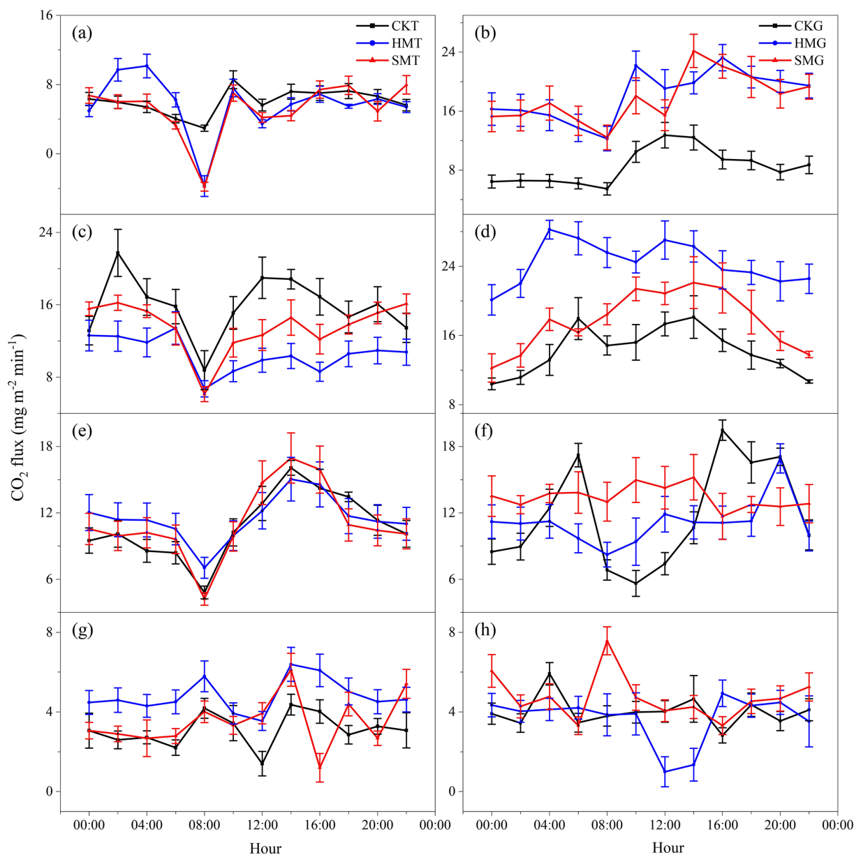
Figure 4. Diurnal variation in soil CO 2 fluxes from (a, c, e, g) tea rows and (b, d, f, h) inter-row zones under different green manure intercropping treatments across seasons: (a, b) spring, (c, d) summer, (e, f) autumn, and (g, h) winter. CK for control; SM and HM for intercropping types, T for tea row, G for inter-row.
