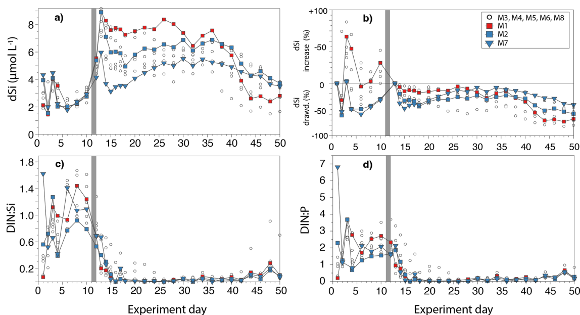
Figure 2. Dissolved concentrations and nutrient ratios during the experiment. The deep water (DW) additions on days 11 and 12 are marked by a gray bar. M1 data are indicated with filled red squares, M2 with filled blue squares, and M7 with filled blue triangles, indicating the admixture with either “extreme” DW (red) or “moderate” DW (blue). Open black symbols in (a) show the dSi range of the other mesocosm experiments as a comparison. (a) dSi concentration (in \mu\text{mol L}^{-1} ), (b) dSi drawdown (in %) calculated by dividing the dSi concentration during the experiment with the initial dSi at the beginning of the experiment (day 1) and after replenishment of dSi on day 12. The horizontal line indicates the initial 100 % calculated with the initial dSi on day 1 for the first 10 d and day 12 for the rest of the experiment. Data above the 100 % line must be influenced by mixing with high dSi from the BL. (c) DIN : P ratio (in \text{mmol mol}^{-1} ), (d) DIN : dSi (in \text{mmol mol}^{-1} ). N reflects all dissolved nitrogen species ( \text{DIN} = \text{NO}_x and \text{NH}_4 ).
