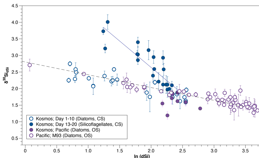
Figure 6. Compilation of \delta^{30}\text{Si}_{\text{dSi}} versus the natural logarithm of dSi displaying data of this study separated for samples from day 1 to 10 (open blue circles), when diatoms dominated the phytoplankton community and from day 13 to 20 (closed blue circles), when silicoflagellates were dominant. Colored dots indicate \delta^{30}\text{Si}_{\text{dSi}} data from the Pacific from this study (sampled outside of the mesocosms; closed purple circles) and a previous cruise (open purple circles; M93) published in Grasse et al. (2021), where diatoms were the dominating phytoplankton. CS: closed system OS: open system. Regression lines for diatom-dominated samples are defined as 2.80 + (-0.39) \cdot x ; r^2 = 0.38 and for silicoflagellate-dominated samples: 5.82 + (-1.60) \cdot x ; r^2 = 0.78 .
