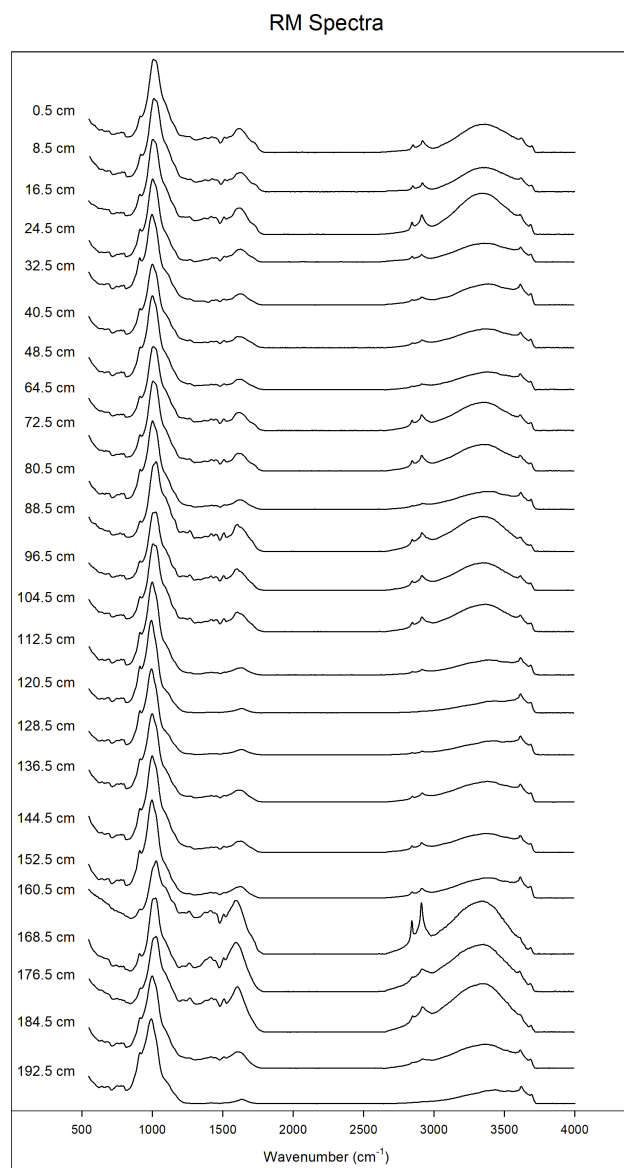
Figure A2. Stacked overlay of the FTIR spectra, Red Mangrove (RM) core.
