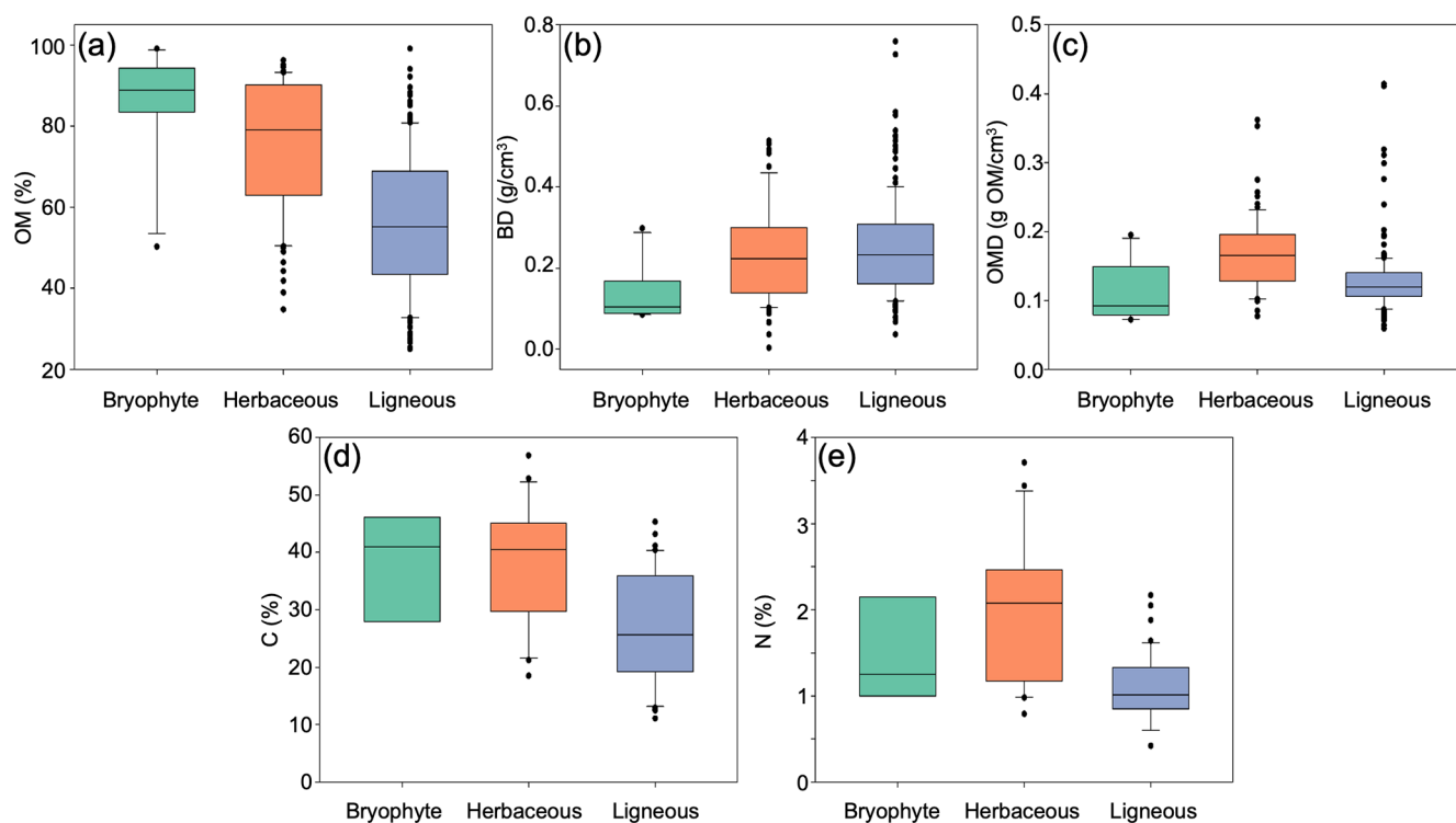
Figure 4. Box plots of geochemical data by peat type. (a) Organic matter content (%), (b) Bulk density ( \text{g cm}^{-3} ), (c) Organic matter density ( \text{g cm}^{-3} ), (d) Carbon content (%), and (e) Nitrogen content (%).
