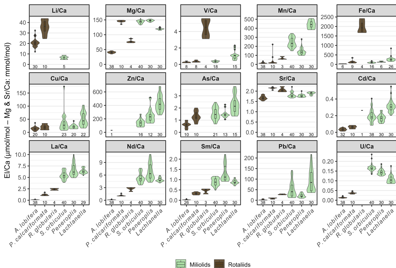
Figure 4. Distribution of El/Ca between different taxa. Values are expressed as \mu\text{mol mol}^{-1} except for Mg/Ca and Sr/Ca that are \text{mmol mol}^{-1} . The colors separate the species into two orders; rotaliids (brown) and miliolid (green) foraminifera. Letters above each distribution indicate statistically significant differences between species in each order. Numbers at the x axes represents the number of replicate analyses. The arrow marks an outlier Zn/Ca value ( 4063 \mu\text{mol mol}^{-1} ) that was excluded from the plot.
