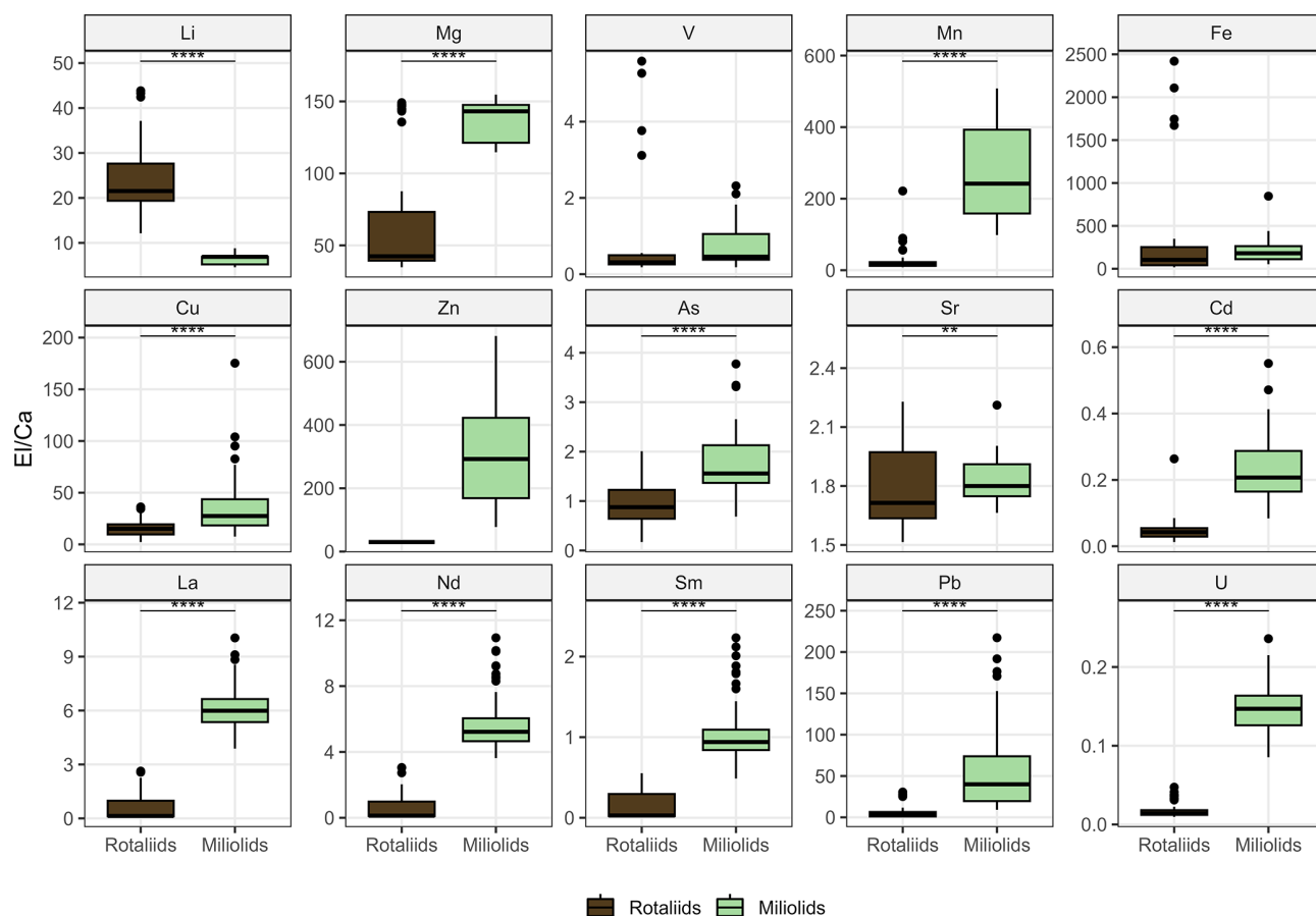
Figure 2. Comparison of element / Ca ratios in rotaliids and miliolids calcite tests. Values shown in \mu\text{mol mol}^{-1} , except for Mg/Ca and Sr/Ca, which are expressed in \text{mmol mol}^{-1} . Two asterisks indicate 0.95 and three indicate 0.99 p value based on Mann–Whitney U tests with FDR correction.
