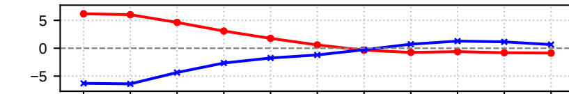
(k) MLD (m)
