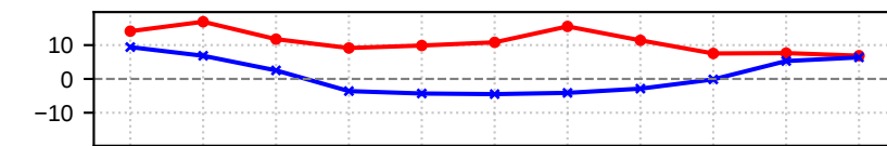
(m) SW ( \text{W m}^{-2} )
