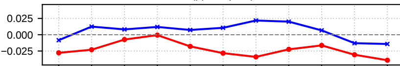
(p) TP (mm)
