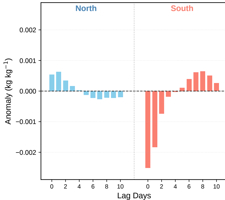
(b) QV2M-qs(SST)
