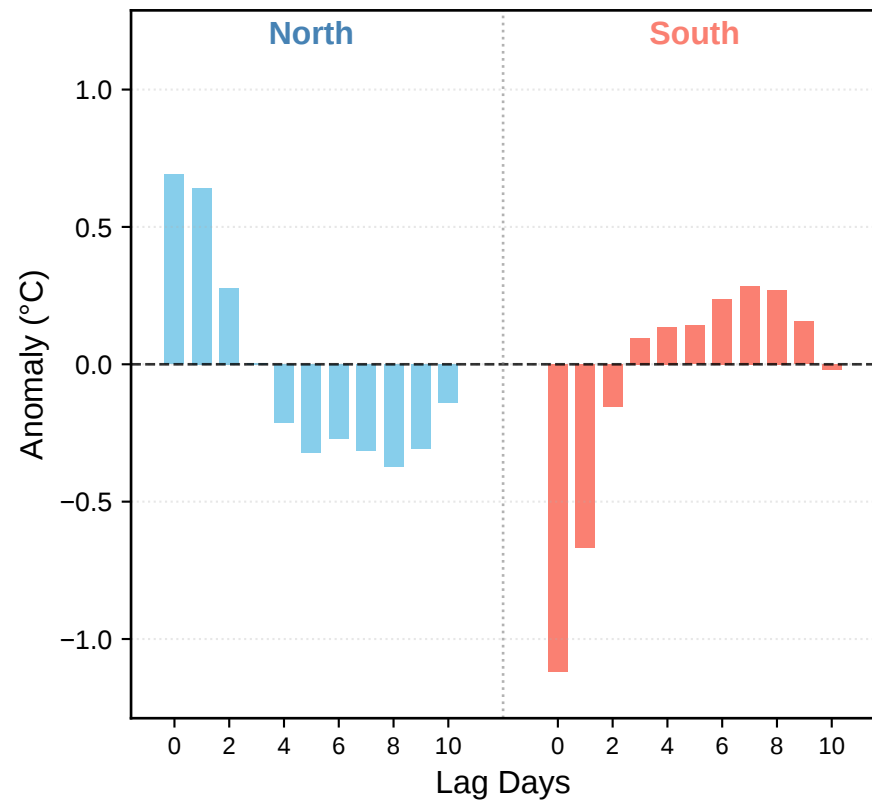
(a) T2M-SST
