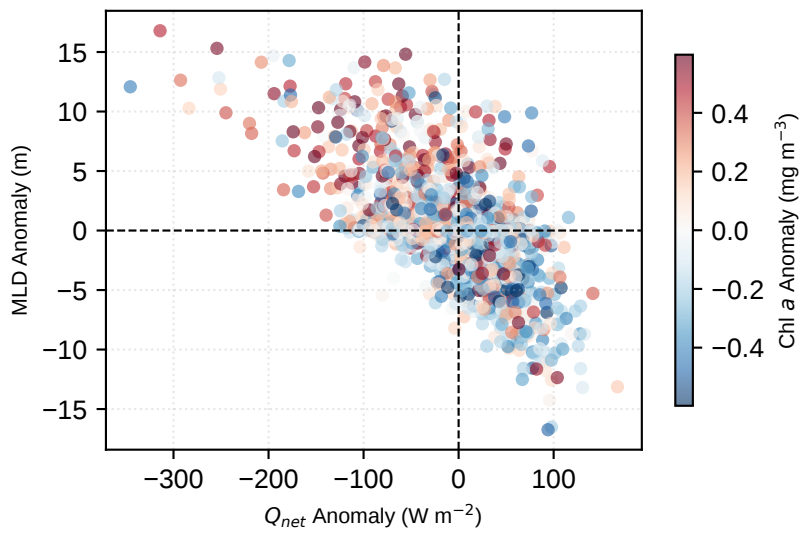
(b) Northern Region Q_{net}(t-1) vs MLD(t), R=-0.62
