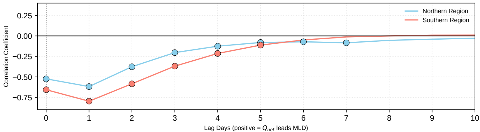
(b) Northern Region Q_{net}(t-1) vs MLD(t), R=-0.62
