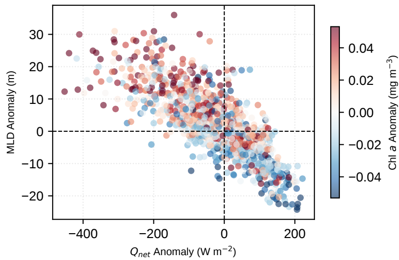
(c) Southern Region Q_{net}(t-1) vs MLD(t), R=-0.80
