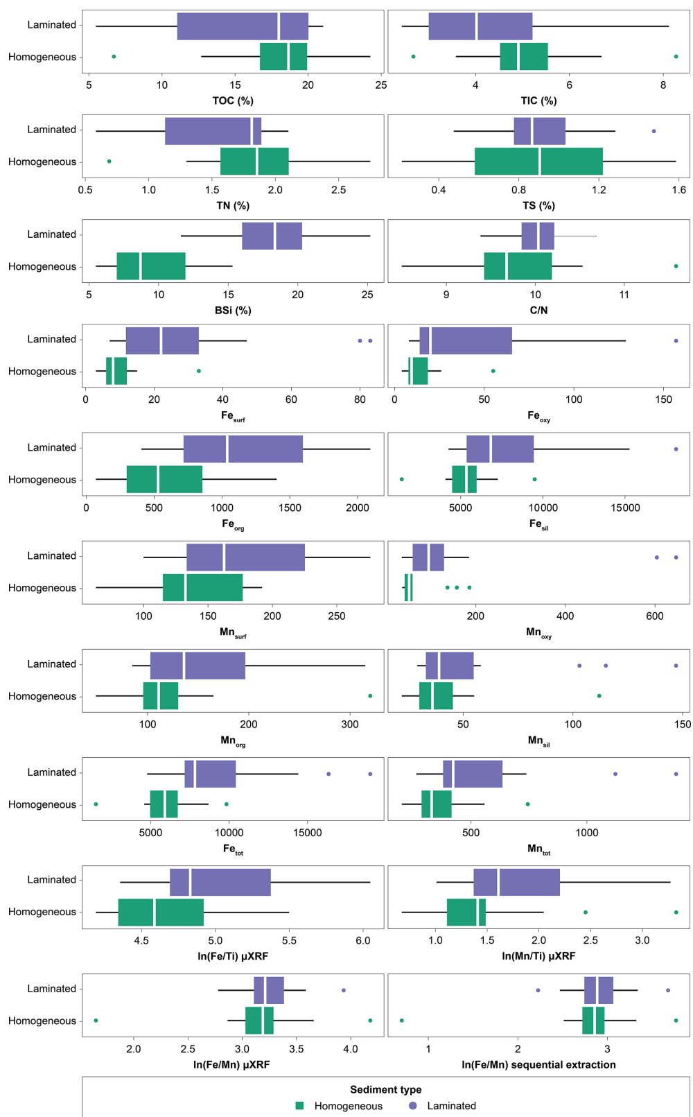
Figure A4. Boxplots of selected geochemical variables grouped by sediment type.
