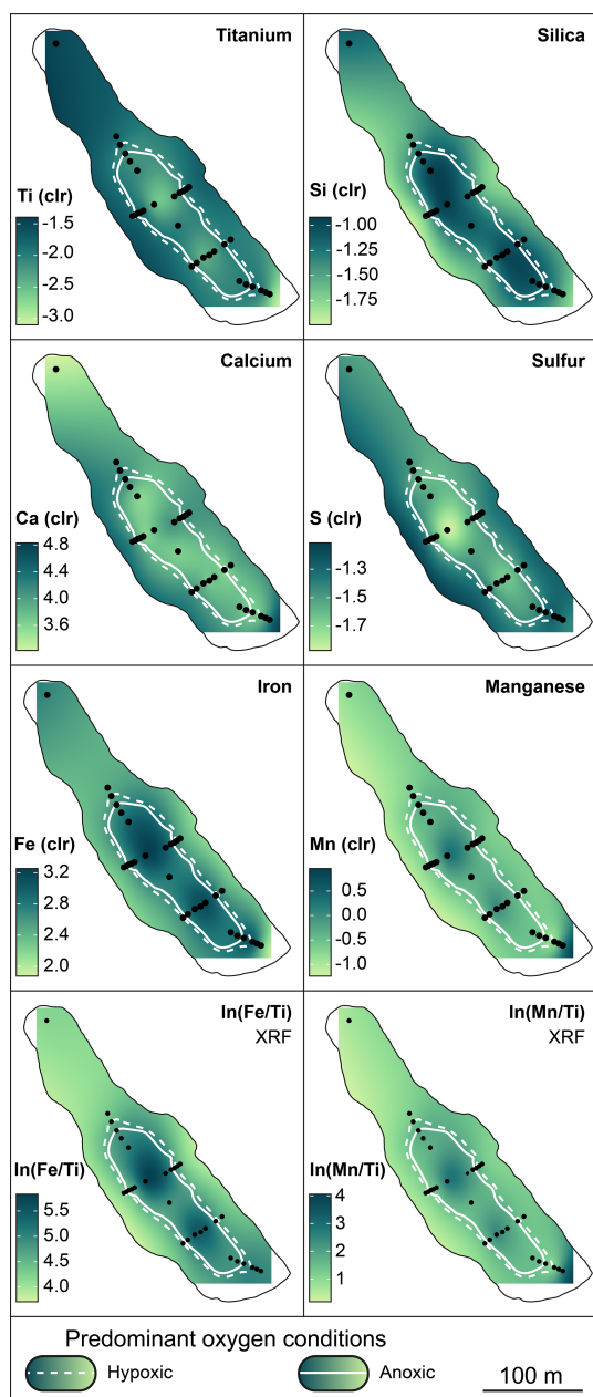
Figure 4. Spatial variability of selected elements and their ratios from the \mu XRF scan. Dots indicate coring locations.
