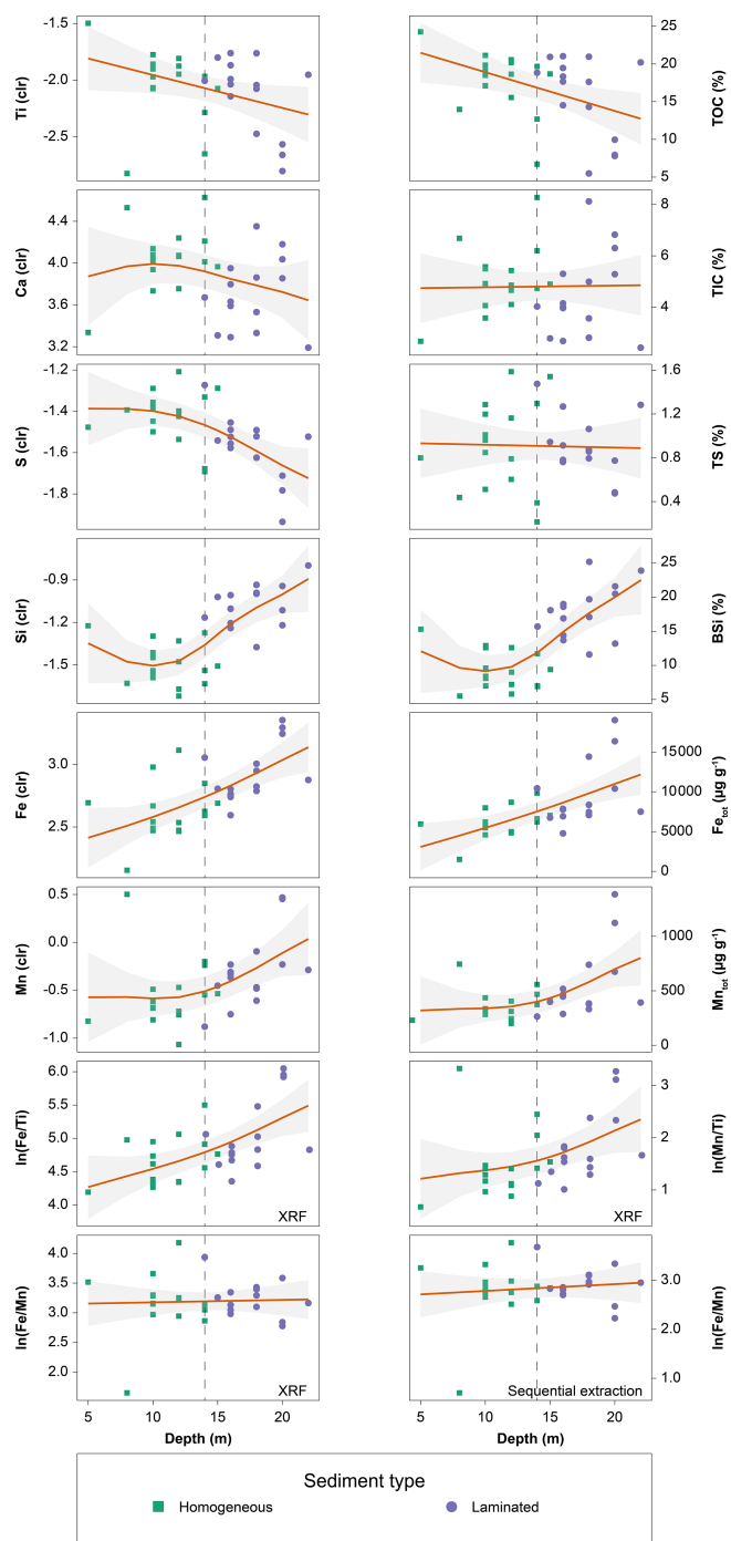
Figure 7. Change in measured element abundances, concentrations, and ratios with water depth. GAMs are shown as smooth lines with a 0.95 confidence interval.
