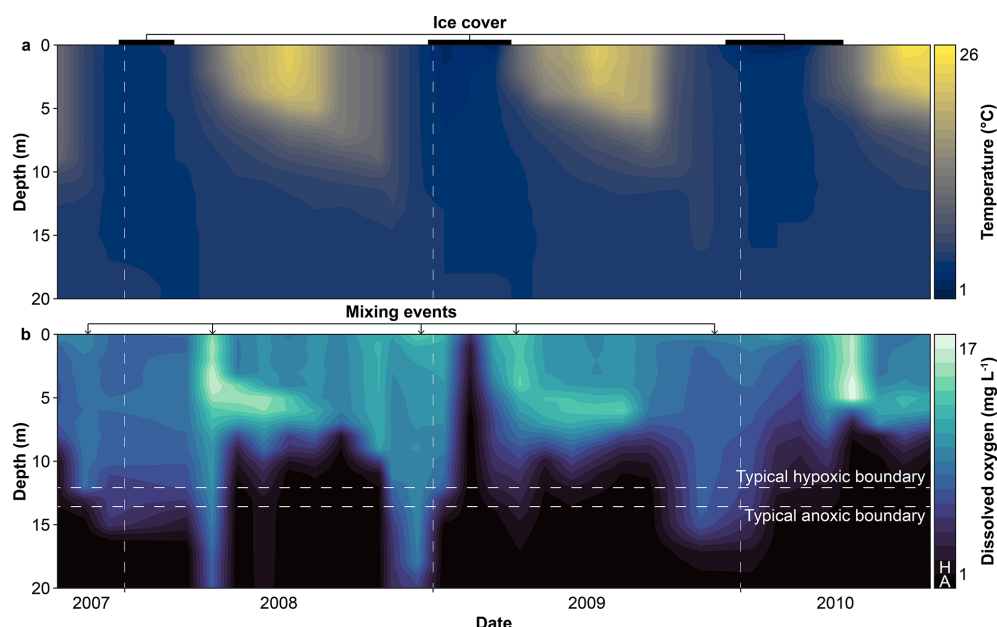
Figure 2. Lake Łazduny water properties based on in situ measurements between October 2007 and August 2010: (a) water temperature and (b) dissolved oxygen concentration. Black horizontal bars indicate ice cover.
