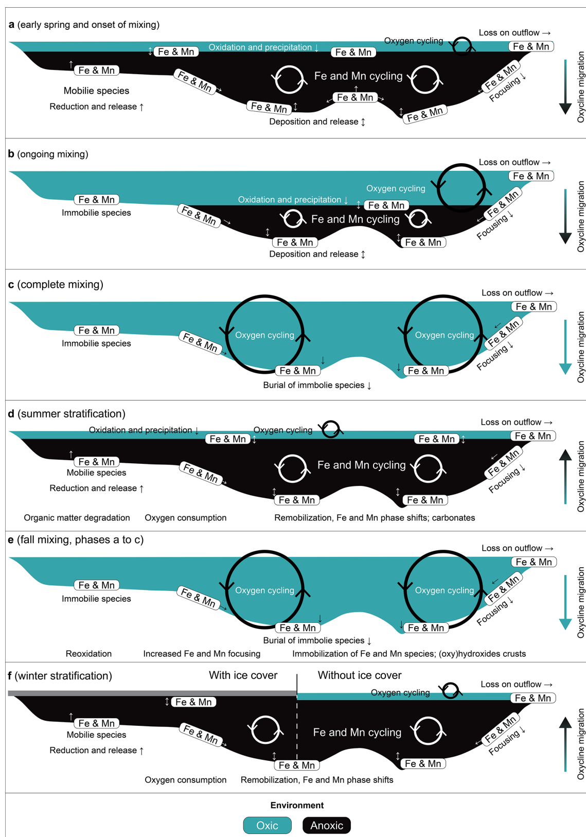
Figure 8. Schematic of mixing-driven geochemical Fe and Mn focusing in the Lake Łazduny.
