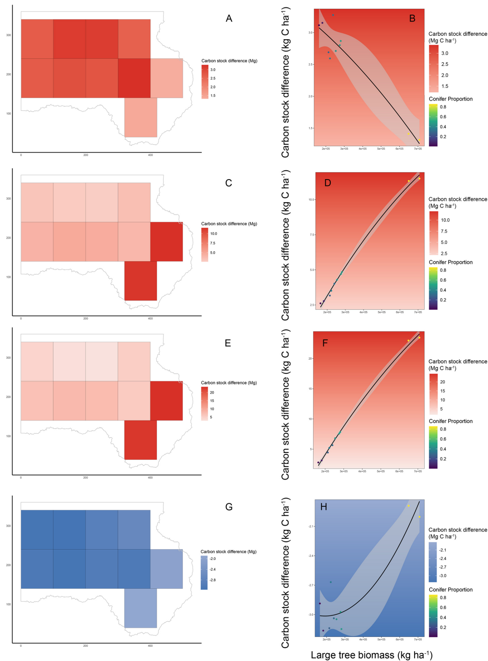
Figure 4. Differences in ha-scale carbon ( C_{ha} ) stocks (measured in Mg\ C\ ha^{-1} ) estimated using different wood carbon fraction (CF) assumptions. Per ha-level differences are calculated as the difference between C_{ha1} (generated using species-specific wood CF data) and C_{ha2} (panels A–B; generated assuming wood CFs for temperate biome trees specific to conifers and angiosperms); C_{ha3} (panels C–D; generated assuming non-biome-specific wood CFs for conifers and angiosperms); C_{ha4} (panels E–F; generated assuming a single IPCC default wood CF assumption); and C_{ha5} (panels G–H; generated assuming a single 50 % wood CF assumption). Therefore in all maps and graphs, (i) all values above 0 and in red shading indicate instances where species-specific wood CFs ( C_{ha1} ) are higher compared to estimates generated using generalized wood CF assumptions ( C_{ha2} – C_{ha5} ), and (ii) all values below 0 and in blue shading indicate instances where species-specific wood CFs ( C_{ha1} ) are lower compared to estimates generated using generalized wood CF assumptions ( C_{ha2} – C_{ha5} ). Left-side panels show spatial variability in differences in subplot-level C stocks for n = 10 ha designations distributed across a 13.5 ha forest dynamics plot in Haliburton, Ontario, Canada. Right-hand panels show statistically significant relationships between differences in C stock estimates (as described above) modeled as a function of large tree biomass ( \geq 10 cm diameter at 1.3 m aboveground) in each ha of forest, and a second-order polynomial term for large tree biomass. In these graphs, error bars represent 95 % confidence limits surrounding model fits, and point colors correspond to the proportion of biomass represented by conifers in each ha of forest (a full analysis of covariance model parameters for each fit is presented in Table S4).
