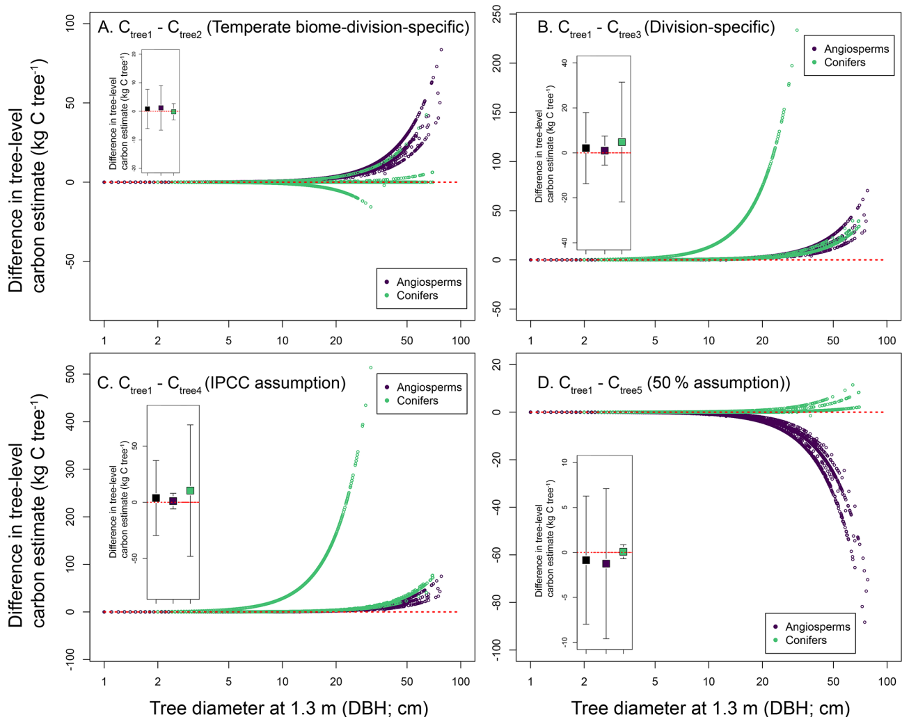
Figure 2. Differences in tree-level carbon (C) stocks (measured in kg C per tree) estimated using different wood carbon fraction (CF) assumptions. Main panels show differences in tree-level C stocks for n = 39\,064 trees distributed across angiosperms ( n = 27\,589 individual trees; purple open points) and conifers ( n = 11\,475 individual trees; green open points). Differences in tree-level C estimates are calculated as follows: (A) C_{\text{tree1}} (generated using species-specific wood CF data) minus C_{\text{tree2}} (generated assuming wood CFs for temperate biome trees specific to conifers and angiosperms). (B) C_{\text{tree1}} minus C_{\text{tree3}} (generated assuming non-biome-specific wood CFs for conifers and angiosperms). (C) C_{\text{tree1}} minus C_{\text{tree4}} (panel C; generated assuming a single IPCC default wood CF assumption). (D) C_{\text{tree1}} minus C_{\text{tree5}} (generated assuming a single 50% wood CF assumption). Red dotted lines denote 0 differences in tree-level C stock estimates, such that (i) all values above 0 indicate instances where species-specific wood CFs ( C_{\text{tree1}} ) are higher compared to estimates generated using generalized wood CF assumptions ( C_{\text{tree2}}\text{--}C_{\text{tree5}} ), and (ii) all values below 0 indicate instances where species-specific wood CFs ( C_{\text{tree1}} ) are lower compared to estimates generated using generalized wood CF assumptions ( C_{\text{tree2}}\text{--}C_{\text{tree5}} ). Inset graphs in each panel represent mean differences in C_{\text{tree}} estimates (calculated as in the main panels) across all trees (black symbols), angiosperms (purple-filled symbols), and conifers (green-filled symbols), with error bars denoting 2 standard deviations about the mean.
