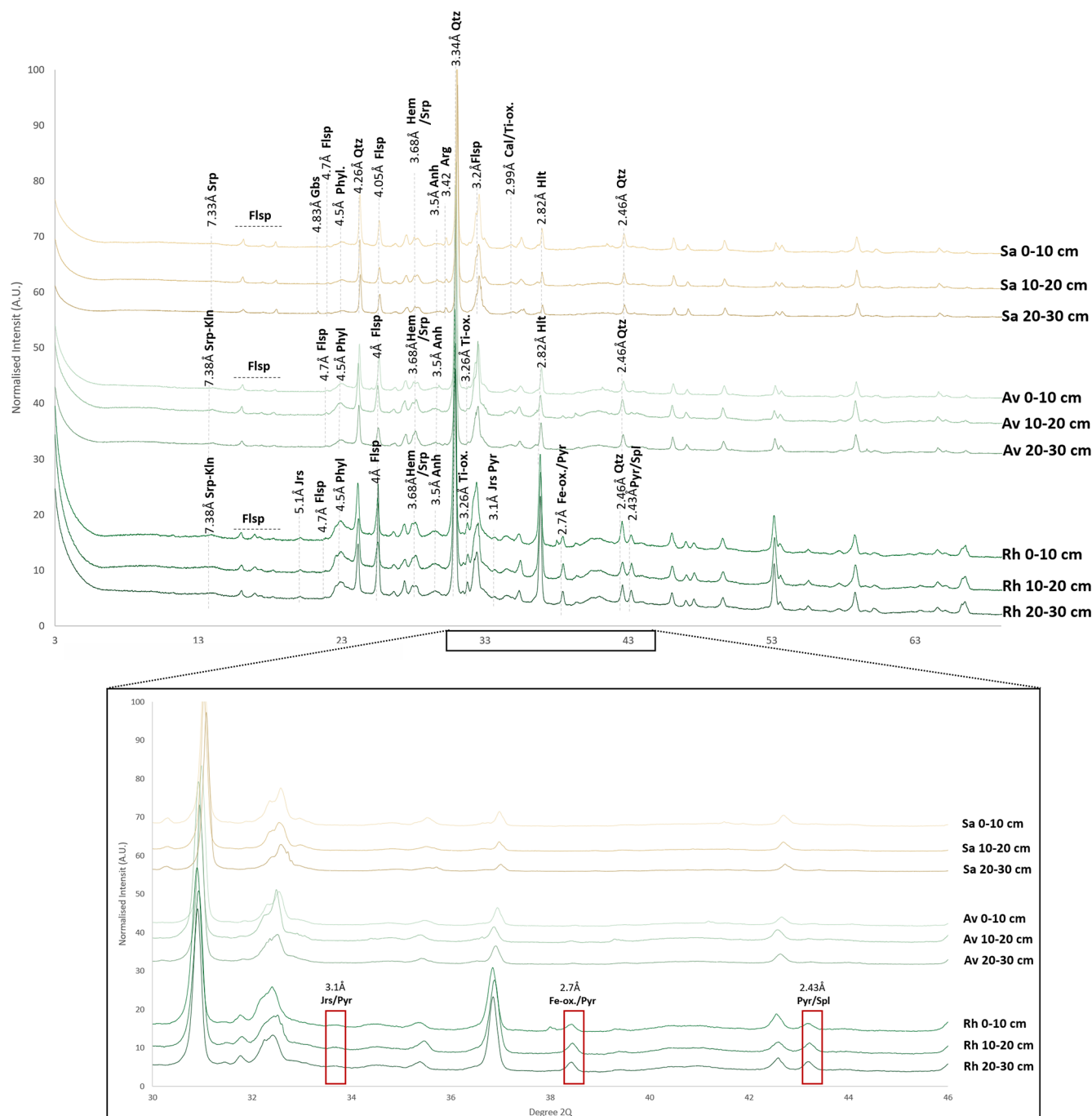
Figure 3. X-ray diffraction (XRD) patterns of soil samples collected from Salt-flat (Sa), Avicennia marina (Av), and Rhizophora stylosa (Rh) stands. Major identified mineral phases include: Srp: Serpentine, Kln: Kaolinite, Flsp: feldspar, Jrs: jarosite, Gbs: gibbsite, Phyl: phyllosilicates, Qtz: quartz, Hem: hematite, Anh: anhydrite, Arg: aragonite, Ti-Ox: titanium oxides, Pyr: pyrite, Cal: Calcite ( \text{Mg}^{2+} ), Hlt: halite, Fe-ox: iron oxides and oxyhydroxides (grouped).
