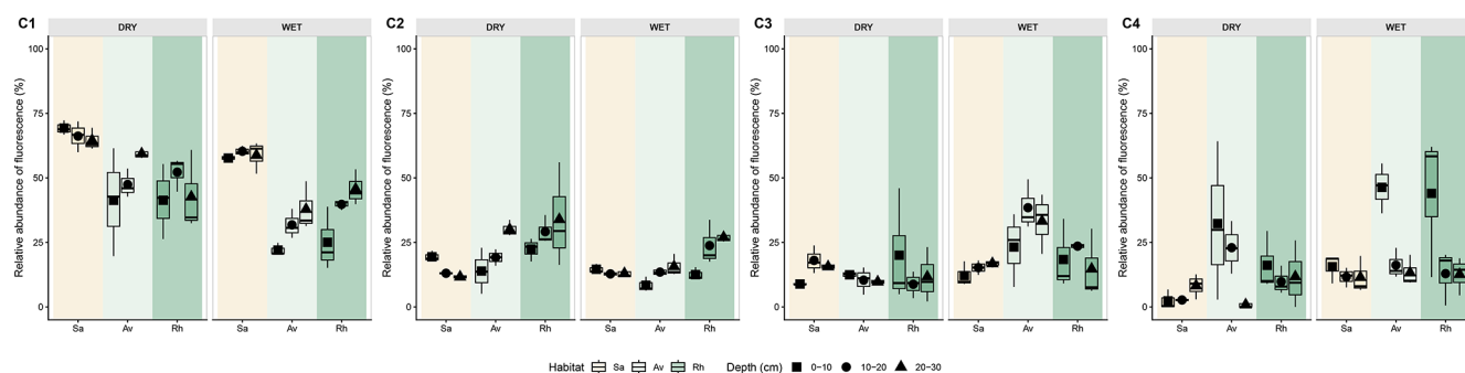
Figure A7. EEM contour plots of the four PARAFAC components (C1, C2, C3, C4) and seasonal variations in their relative fluorescence abundance (%) across a land-sea gradient in salt-flat (Sa), Avicennia marina (Av), and Rhizophora stylosa (Rh). Symbols represent soil depth layers (squares: 0–10 cm; circles: 10–20 cm; triangles: 20–30 cm).
