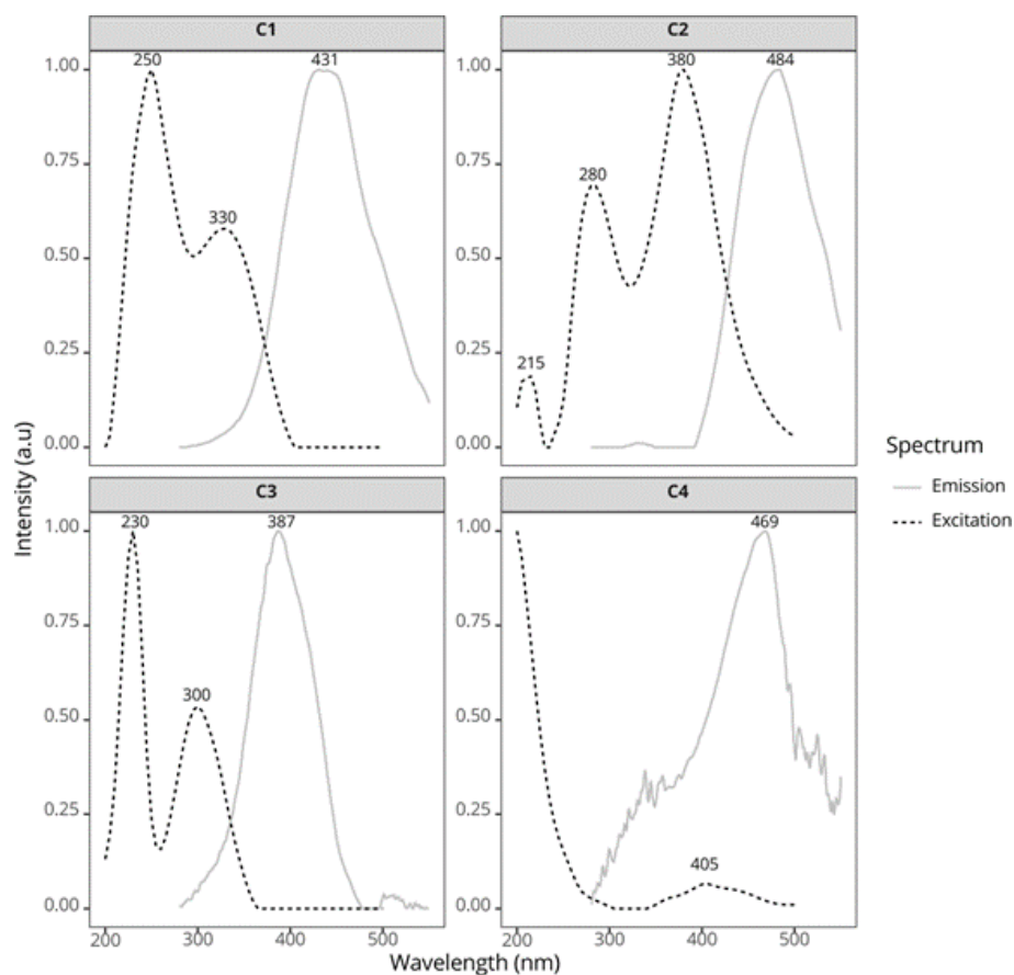
Figure A2. Excitation and emission spectra of the four fluorescent components identified using the PARAFAC model, showing their respective excitation and emission maxima.
