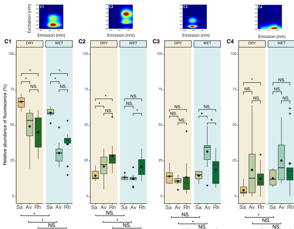
Figure 7. EEM contour plots of the four PARAFAC components (C1, C2, C3, C4) and seasonal variations in their relative fluorescence abundance (%) across a land-sea gradient in salt-flat (Sa), Avicennia marina (Av), and Rhizophora stylosa (Rh). Significant differences between habitats (ANOVA/Kruskal–Wallis, see Table A8 for full test results) and between seasons (Student’s t -test/Mann–Whitney) are indicated (* p < 0.05 , NS = no significant difference, see Table A7 for full test results). Variations across soil depth layers are presented in Fig. A7.
