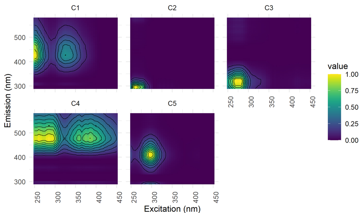
Figure 3. Excitation-emission matrix (EEM) fluorescence spectra of the 5-component PARAFAC model. Fluorescence is expressed in Raman Unit (RU).
