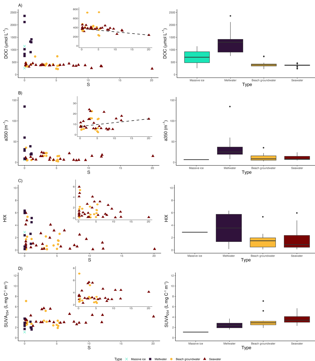
Figure 5. Distribution of (A) DOC, (B) a_{350} , (C) HIX, and (D) \text{SUVA}_{254} across the salinity gradient ( S ) and among the different sample types (i.e., beach groundwater, massive ice, meltwater, and seawater). Note that only one massive ice sample is included. The zoomed-in panels display only beach groundwater (yellow dots) and seawater (brown triangle) samples, along with a theoretical mixing line (dashed black line) connecting the “fresh” and “salty” endmembers for DOC and a_{350} . These endmembers were defined based on the most enriched and depleted stable isotope signatures in the dataset, corresponding to salinity values of 20.08 ( N = 1 ) and 0.18–0.30 ( N = 8 ), respectively. As the underlying fluorescence and absorbance components used to calculate HIX and \text{SUVA}_{254} indices were not retained, non-linear mixing curves could not be reconstructed. In the boxplots, black lines indicate the medians, whiskers represent the full range of data, and individual points denote outliers.
