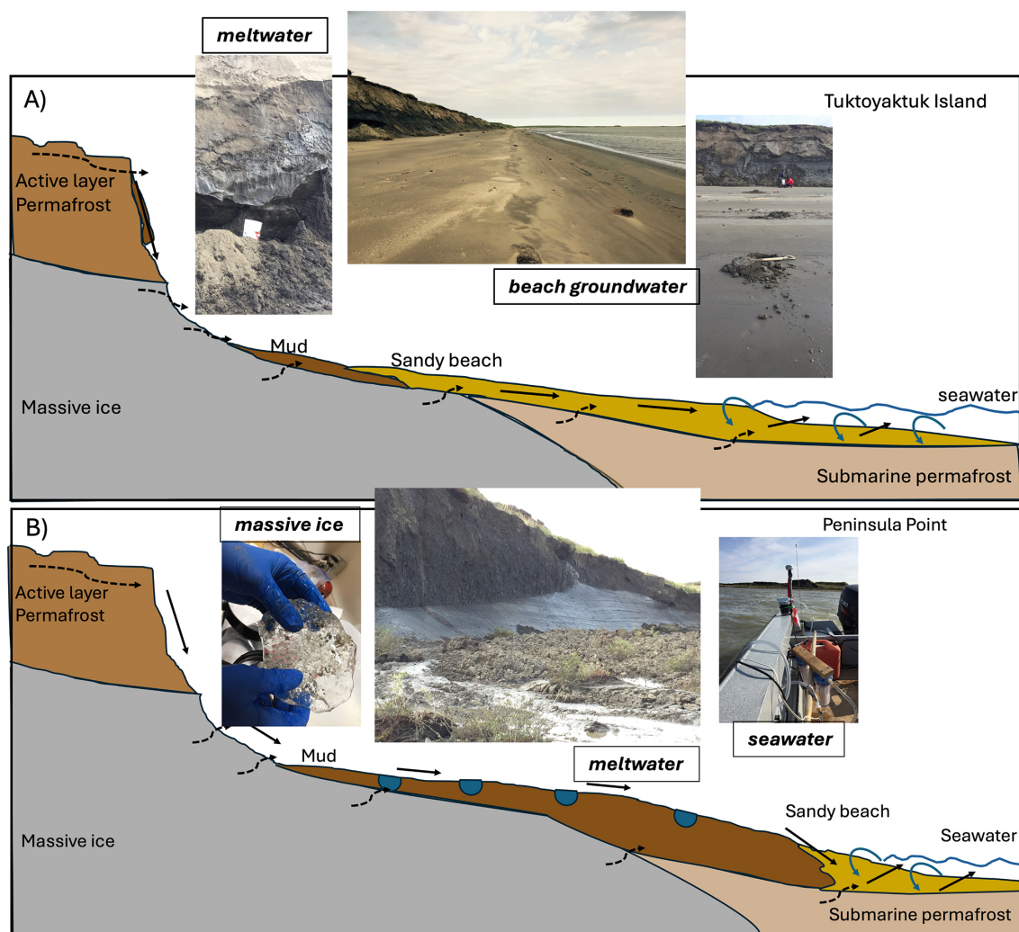
Figure 2. Schematic cross-sections and photographs illustrating the coastal permafrost landscape at Tuktoyaktuk Island (A) and Peninsula Point (B; not to scale) as examples of a retrogressive thaw slump system. Black arrows show theoretical surface (solid lines) and subsurface (dashed lines) flow paths, while blue arrows represent recirculating seawater driven by tidal and wave inputs into the intertidal zone of sandy beaches. Blue dots in panel (B) mimic melt ponds. The locations of the different sample types (“massive ice”, “meltwater”, “beach groundwater”, and “seawater”) are indicated. These conceptual models are adapted from Kipp et al. (2025) based on Hayes et al. (2022) for Peninsula Point and Whalen et al. (2022) and Coote et al. (2025) for Tuktoyaktuk Island.
