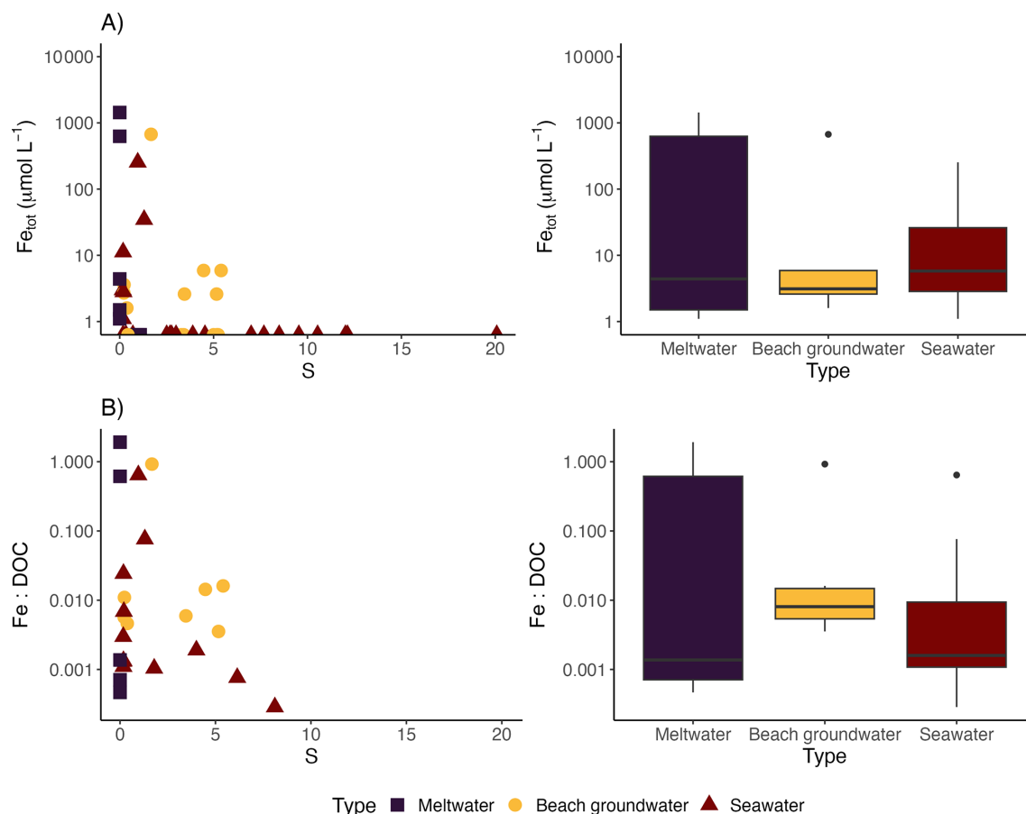
Figure 7. Distribution of total dissolved Fe ( \text{Fe}_{\text{tot}} , \mu\text{mol L}^{-1} ) (A), and Fe-DOC ratio (B) across the salinity gradient ( S ), and by sample type. The y-axis in each panel is shown on a logarithmic scale to accommodate the broad range of Fe concentrations. Note that there is no \text{Fe}_{\text{tot}} data from the massive ice samples and Fe : DOC ratios were calculated only for \text{Fe}_{\text{tot}} concentration higher than the detection limit.
