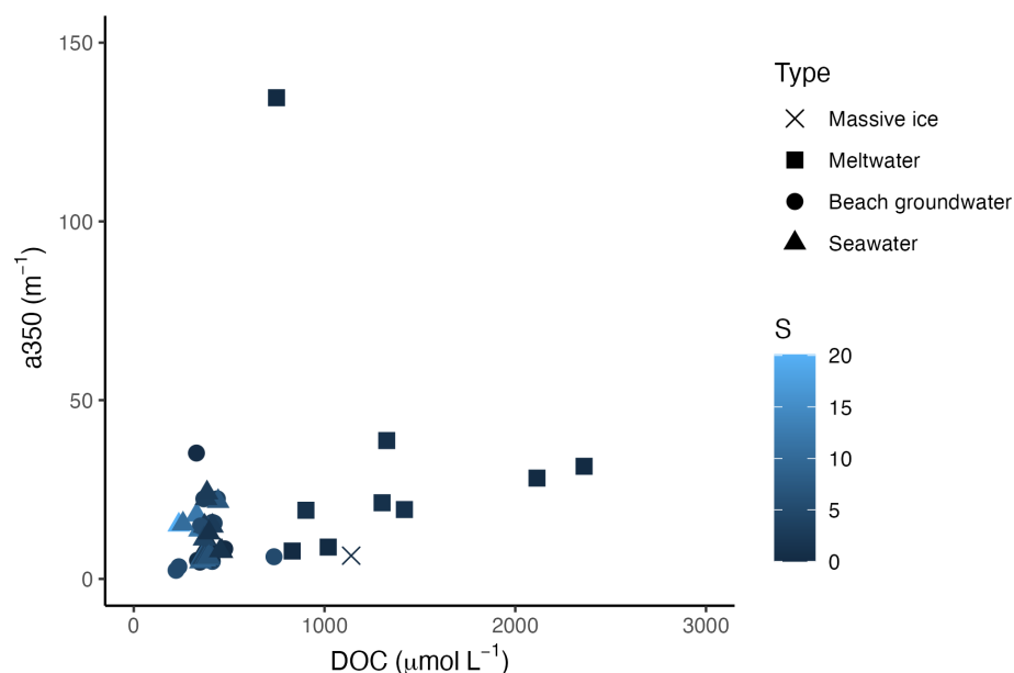
Figure 6. Relationship between absorption coefficients at 350 nm ( a_{350} , \text{m}^{-1} ) and DOC concentrations ( \mu\text{mol L}^{-1} ) across all samples along the permafrost-to-nearshore aquatic continuum.
