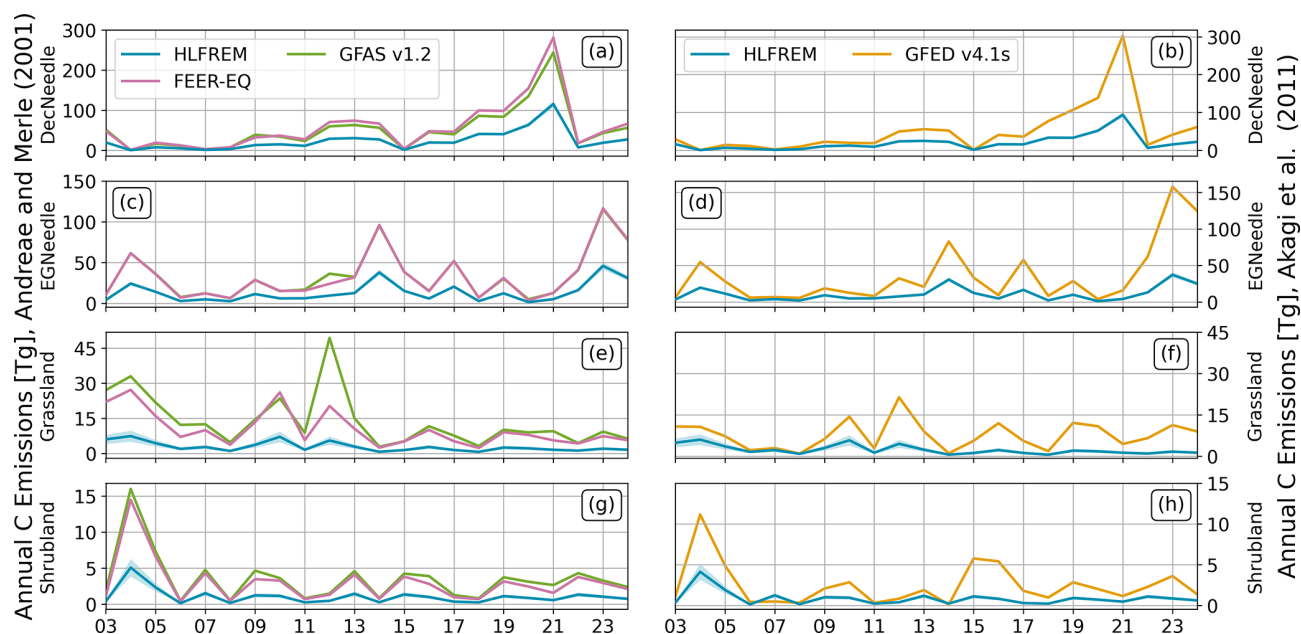
Figure 12. Timeseries of HL Wildfire Emissions of Carbon for (a, b) Deciduous Needleleaf Forest, (c, d) Evergreen Needleleaf Forest, (e, f) Grasslands, and (g, h) Shrublands biomes, for (a, c, e, g) FEER, GFAS v1.2, and HLFREM (using EFs from Andreae and Merlet, 2001), and (b, d, f, h) GFEDv4.1s and HLFREM (using EFs from Akagi et al., 2011). Regression analysis on the timeseries can be found in Fig. A4 in Appendix A.
