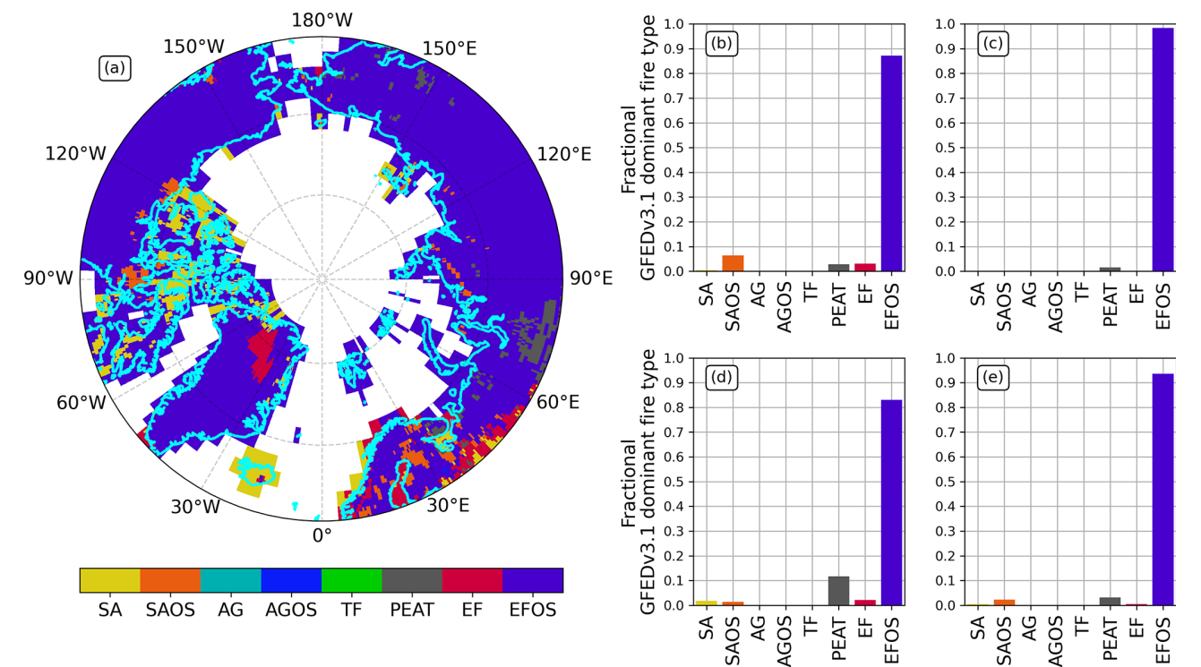
Figure 10. GFAS v1.2 land cover classes, based on dominant fire type in GFED v3.1 and organic soils and peat maps, taken from Kaiser et al. (2012). (a) Land cover classes map, for Savannah (SA), Savannah with organic soils (SAOS), Agriculture (AG), Agriculture with organic soils (AGOS), Tropical Forest (TF), Peat (PEAT), Extratropical Forest (EF), and Extratropical Forests with organic soils (EFOS). 60° N is denoted with a red line. (b–e) Fractional land cover for (b) HL DecNeedle, (c) HL EGNeedle, (d) HL Grassland, and (e) HL Shrubland.
