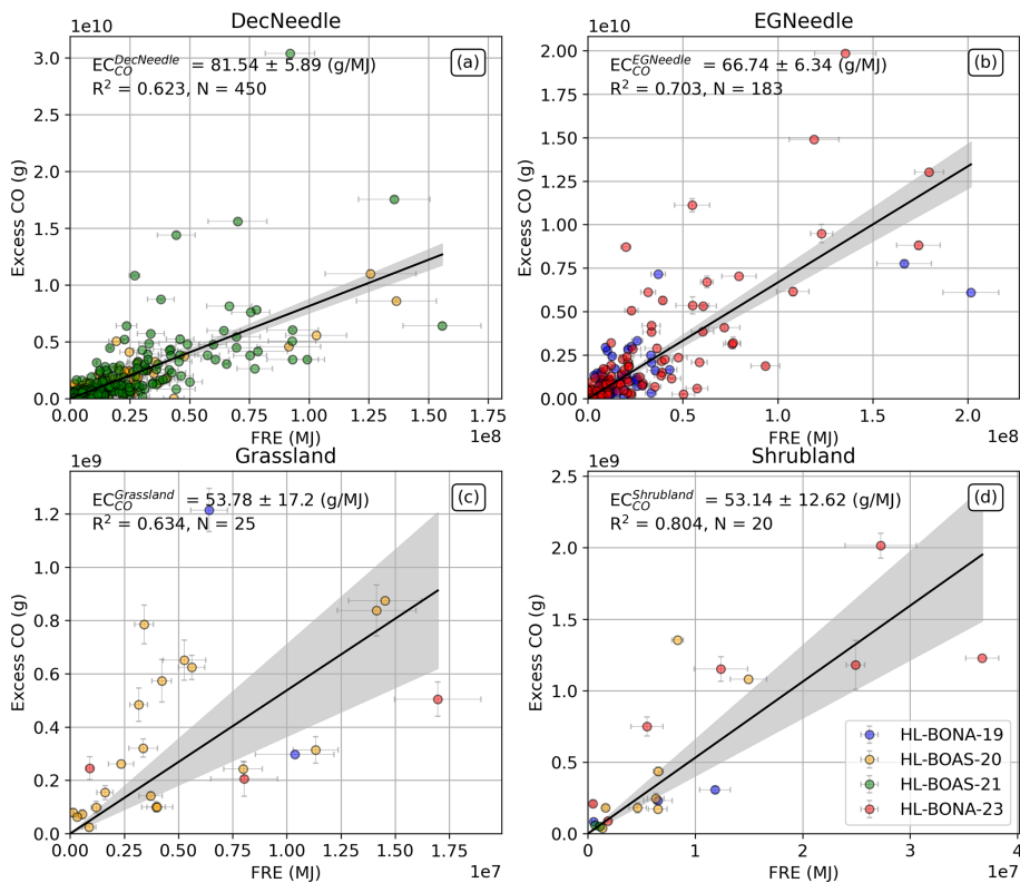
Figure 7. HLFREM biome-specific CO emission coefficients ( EC_{CO}^b , in g MJ -1 ) derived from the set of matchup fires for (a) Deciduous Needleleaf Forests, (b) Evergreen Needleleaf Forests, (c) Grasslands, and (d) Shrubland fire-biomes. Each datapoint represents a single matchup fire that had its plume total Excess CO and total released FRE assessed for a matching time-period, and the EC_{CO}^b value for the fire-biome is derived from the slope of the OLS linear best fit (solid black line) to these data. Colour of the scatter points denotes the ROI containing the fire (see Fig. 3c). Error bars denote the standard deviation of FRP values and the uncertainty in the SSP TCCO produce respectively, as calculated following (Nguyen et al., 2023). The shaded area indicates the uncertainty on the slope of the linear best fit, taken to be the uncertainty on the derived EC_{CO}^b value.
