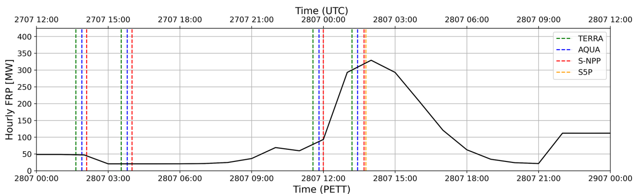
Figure 5. Example of the hourly FRP time-series from GFAS v1.4, used to generate an FRE measure for a single matchup fire (i.e. the match-up fire in Fig. 4, as shown above). The hourly FRP timeseries data were generated from the set of individual FRP observations provided by MODIS on AQUA and TERRA, using the diurnal cycle model of Andela et al. (2015). Additionally, the VIIRS observations on S-NPP used for fire-matchup identification are also shown. Times of the individual satellite overpasses, as well as of the S5P overpass time used to provide the TCCO data for this fire-matchup, are indicated.
