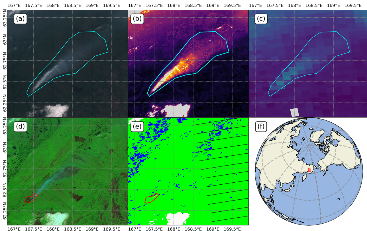
Figure 4. Example of a matchup fire imaged in Siberia ( 62.39^{\circ}\text{N} , 167.49^{\circ}\text{E} ) on 28 July 2020 at 01:42 UTC (13:42 PETT). The digitised outline of the plume (cyan) and burning area (red) are shown superimposed on (a) RGB (M05-M04-M03) imagery via S-NPP (VIIRS), (b) AOD (processed via EPS) from S-NPP (VIIRS), (c) Sentinel-5P TCCO data, (d) False Colour Composites (M11-I02-I01) via S-NPP (VIIRS), (e) VIIRS Active Fire Product (VNP14) from S-NPP (VIIRS). Green: Non burning vegetation. Yellow: Active Fire Hotspot, Blue: Water, White: Cloud, Black: No Data. (f) Geographic location and extent of the plots shown (red). VIIRS imagery courtesy of NOAA/NASA (S-NPP). AOD processing courtesy of EUMETSAT EPS. Sentinel-5P TROPOMI data courtesy of ESA/Copernicus. VIIRS Active Fire Product (VNP14) courtesy of NASA/NOAA.
