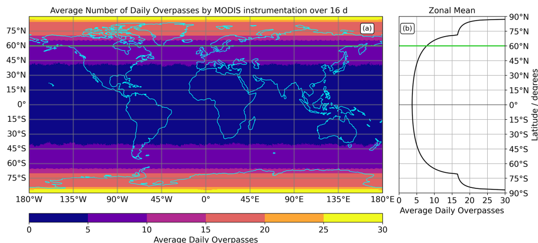
Figure 1. (a) Mean number of daily overpasses at any Earth location made by MODIS on AQUA and TERRA, and (b) zonal mean number of daily overpasses. Daily averages based on 16 d of data taken between 11 August 2024, 00:00 UTC and 27 August 2024, 00:00 UTC, gridded to a regular 0.5^\circ \times 0.5^\circ grid. At latitudes where HL fires occur ( 60\text{--}75^\circ\text{N} , green line and above), there is a latitudinal observation frequency dependence that provides on average between 8 and 18 daily satellite observations from these two systems alone. Each cloud-free observation provides an FRP measure, and which can be used to estimate FRE via temporal integration.
