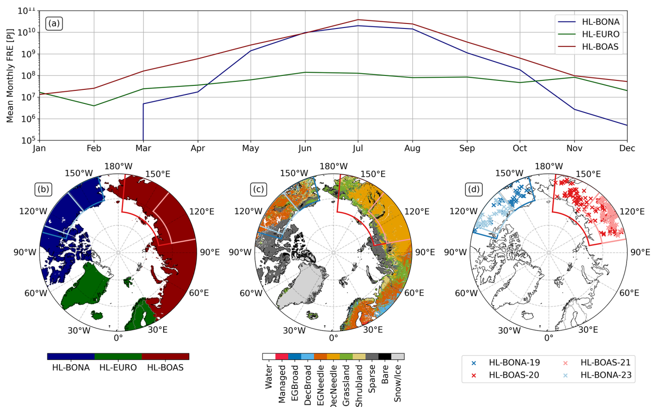
Figure 3. HL fire information. (a) Mean monthly FRE (2003–2024) for HL fires ( \geq 60^\circ \text{N} ) in the regions used by the Global Fire Emissions Database (GFED; Randerson et al., 2017, BONA: Boreal North America, EURO: Europe, BOAS: Boreal Asia), as derived from GFAS v1.2. (b) HL regions used for the mean monthly FRE estimation in (a), as defined by GFED. (c) ROI and aggregated fire biome map, as derived from the CCI Land Cover 2018 map (ESA, 2017) and with biome aggregation detailed in Table A1. (d) The four ROIs used in this study within which the 833 fire-matchup (shown as crosses) were identified. GFAS v1.2 data courtesy of Copernicus Atmosphere Monitoring Service (CAMS)/ECMWF. CCI Land Cover 2018 data courtesy of ESA/Copernicus Climate Change Initiative.
