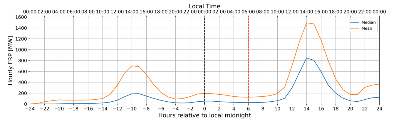
Figure A1. Median (blue) and mean (orange) hourly FRP of all plumes identified in the HLFREM study, during the day before observation (negative hours relative to local midnight) and day of observation (positive hours relative to local midnight) from the hourly FRP dataset. Local midnight and 06:00 local time is shown with the black and red line, respectively.
