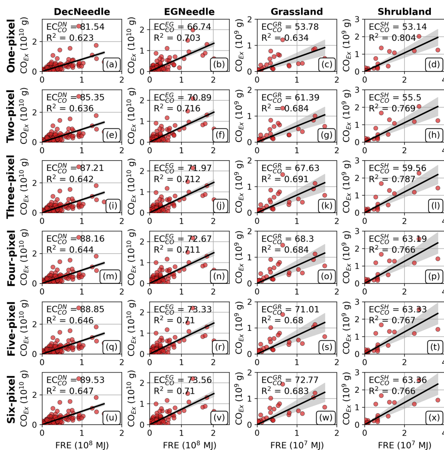
Figure A2. HLFREM biome-specific CO emission coefficients ( \text{EC}_{\text{CO}}^b , in \text{g MJ}^{-1} ) derived for Deciduous Needleleaf Forests (DecNeedle, a, e, i, m, q, u), Evergreen Needleleaf Forests (EGNeedle, b, f, j, n, r, v), Grassland (Grassland, c, g, k, o, s, w), and Shrubland (Shrubland, d, h, l, p, t, x), using a one- (a, b, c, d), two- (e, f, g, h), three- (i, j, k, l), four- (m, n, o, p), five- (q, r, s, t), and six-pixel buffer (u, v, w, x) to determine the background TCCO values, used in Table 5. R^2 values are also shown.
