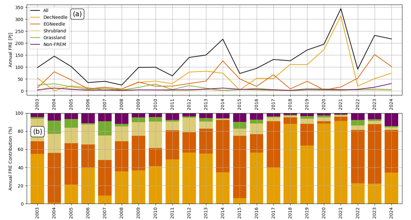
Figure 6. Mean annual HL FRE (a) totals (PJ), and (b) contribution (%) of each of the four most well sampled biomes identified as part of the fire-matchups database, as well as from additional biomes, taken from GFAS v1.2 (2003–2024).
