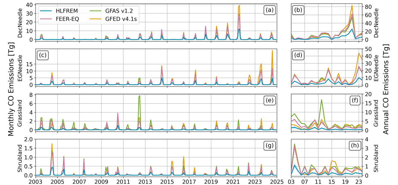
Figure 9. Timeseries of Monthly (a, c, e, g) and Annual (b, d, f, h) HL Wildfire emissions of CO for (a, b) DecNeedle, (c, d) EGNeedle, (e, f) Grassland, and (g, h) Shrubland biomes, calculated using the EC_{CO}^b from HLFREM (blue) and FEER (red) as detailed in Table 4 using daily FRE totals generated by GFAS v1.2. GFAS v1.2 (green) and GFED v4.1s (orange) CO emissions for the same biomes are shown in green. OLS regression analysis can be found in Fig. A3 in Appendix A.
